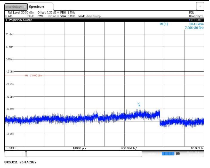
Band26-5MHz-QPSK-27015-1RB#0-Range2:1000~10000MHz
