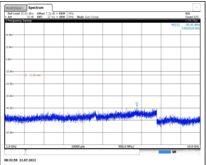
Band26-3MHz-QPSK-26915-1RB#0-Range2:1000~10000MHz
