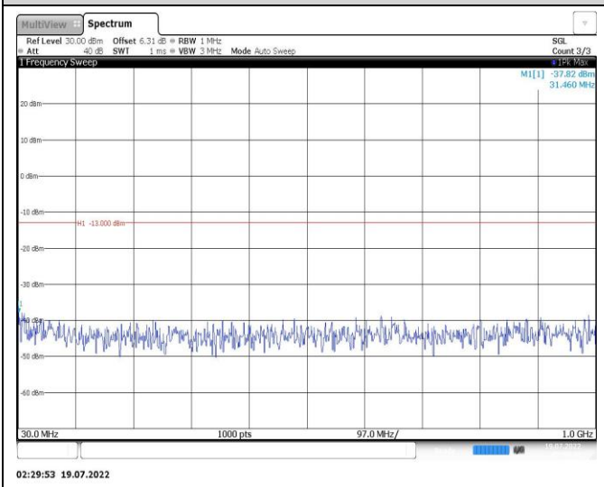
Band25-15MHz-16QAM-26115-1RB#0-Range1:30~1000MHz
