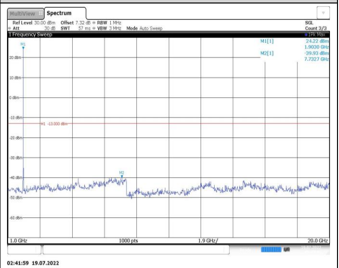
Band25-20MHz-16QAM-26140-1RB#0-Range2:1000~20000MHz
