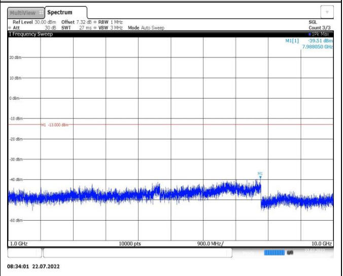
Band26-3MHz-16QAM-26705-1RB#0-Range2:1000~10000MHz
