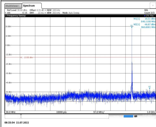
Band26-3MHz-16QAM-26705-1RB#0-Range1:30~1000MHz
