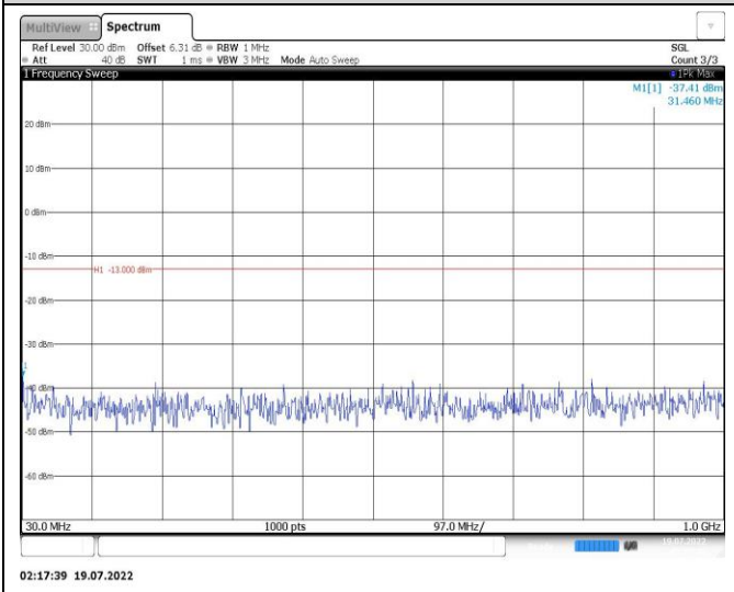
Band25-10MHz-16QAM-26640-1RB#0-Range1:30~1000MHz
