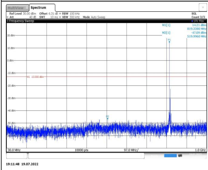
Band26-5MHz-16QAM-26815-1RB#0-Range1:30~1000MHz
