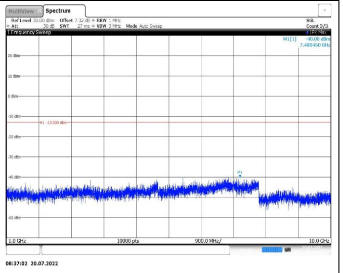
Band26-1.4MHz-QPSK-27033-1RB#0-Range2:1000~10000MHz
