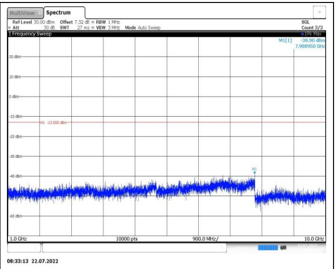
Band26-3MHz-16QAM-26915-1RB#0-Range2:1000~10000MHz
