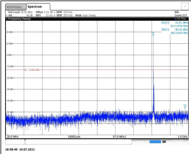
Band26-3MHz-16QAM-26740-1RB#0-Range1:30~1000MHz
