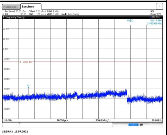
Band26-3MHz-QPSK-26805-1RB#0-Range2:1000~10000MHz
