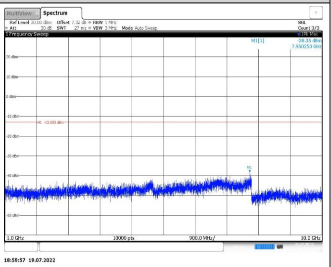
Band26-3MHz-16QAM-26805-1RB#0-Range2:1000~10000MHz
