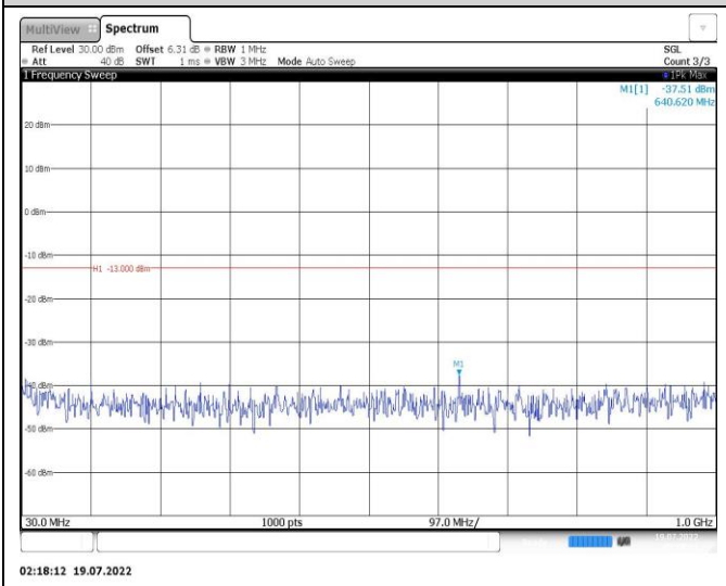
Band25-15MHz-QPSK-26115-1RB#0-Range1:30~1000MHz
