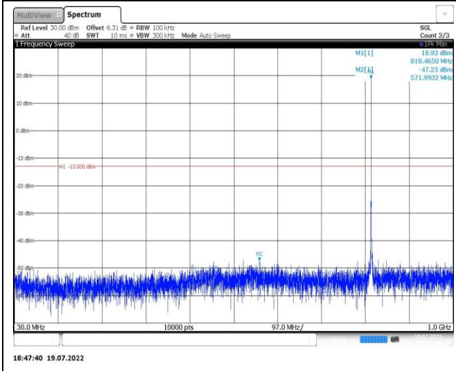
Band26-1.4MHz-16QAM-26783-1RB#0-Range1:30~1000MHz
