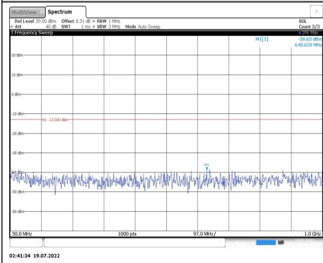
Band25-20MHz-16QAM-26590-1RB#0-Range1:30~1000MHz
