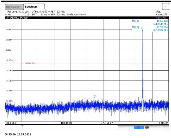
Band26-10MHz-QPSK-26740-1RB#0-Range1:30~1000MHz
