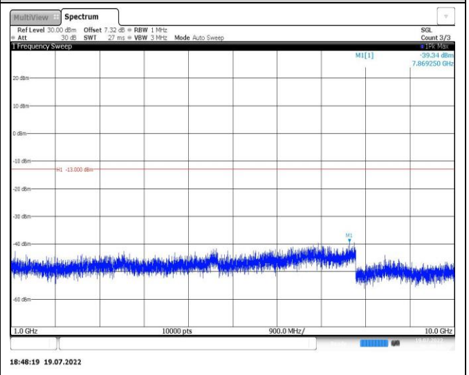
Band26-1.4MHz-16QAM-26797-1RB#0-Range2:1000~10000MHz
