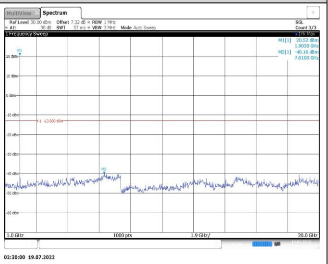
Band25-15MHz-16QAM-26115-1RB#0-Range2:1000~20000MHz
