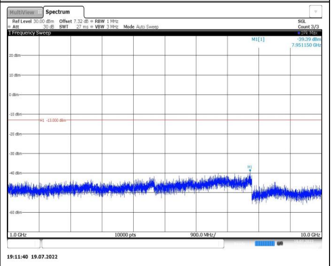
Band26-5MHz-QPSK-26815-1RB#0-Range2:1000~10000MHz
