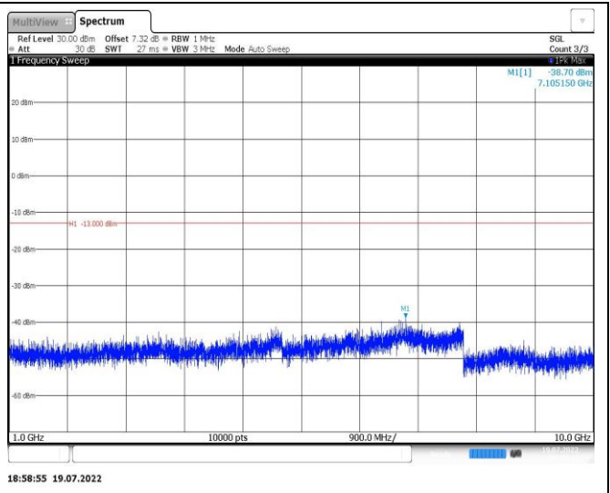
Band26-3MHz-16QAM-26740-1RB#0-Range2:1000~10000MHz
