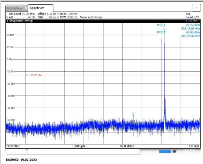
Band26-3MHz-16QAM-26805-1RB#0-Range1:30~1000MHz
