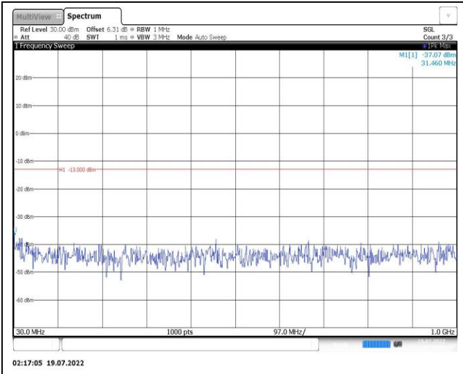
Band25-10MHz-16QAM-26365-1RB#0-Range1:30~1000MHz
