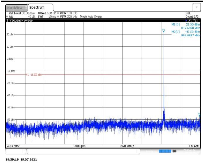
Band26-3MHz-16QAM-26775-1RB#0-Range1:30~1000MHz
