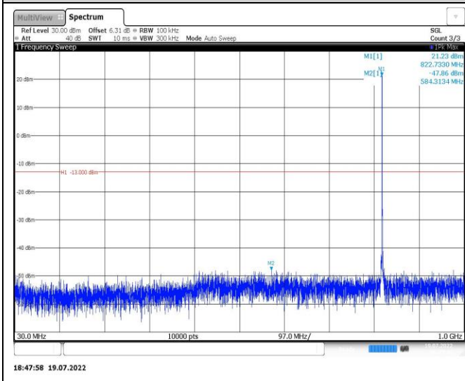
Band26-1.4MHz-QPSK-26797-1RB#0-Range1:30~1000MHz
