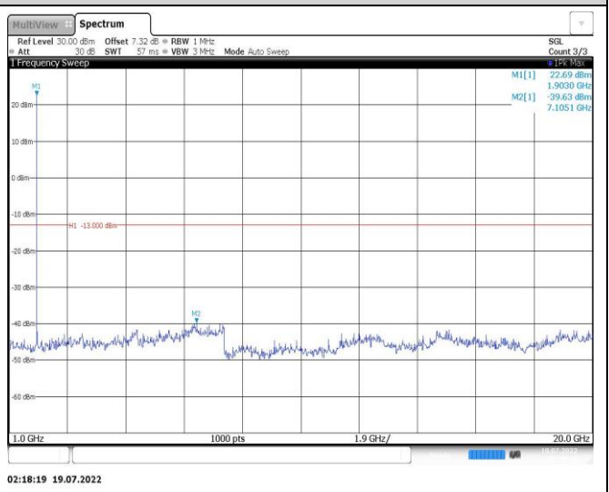
Band25-15MHz-QPSK-26115-1RB#0-Range2:1000~20000MHz
