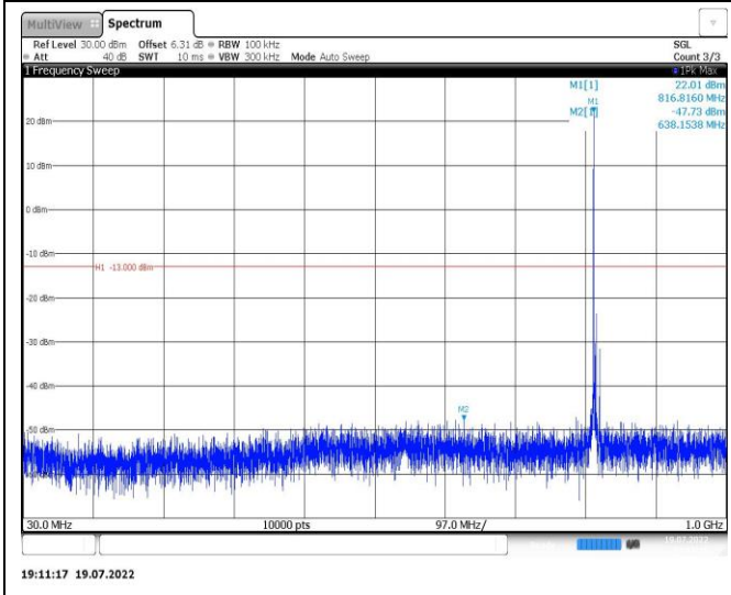
Band26-5MHz-16QAM-26765-1RB#0-Range1:30~1000MHz
