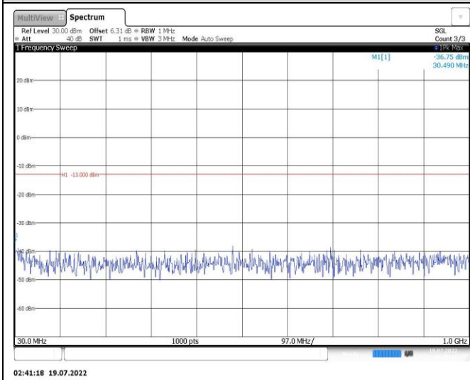
Band25-20MHz-QPSK-26590-1RB#0-Range1:30~1000MHz
