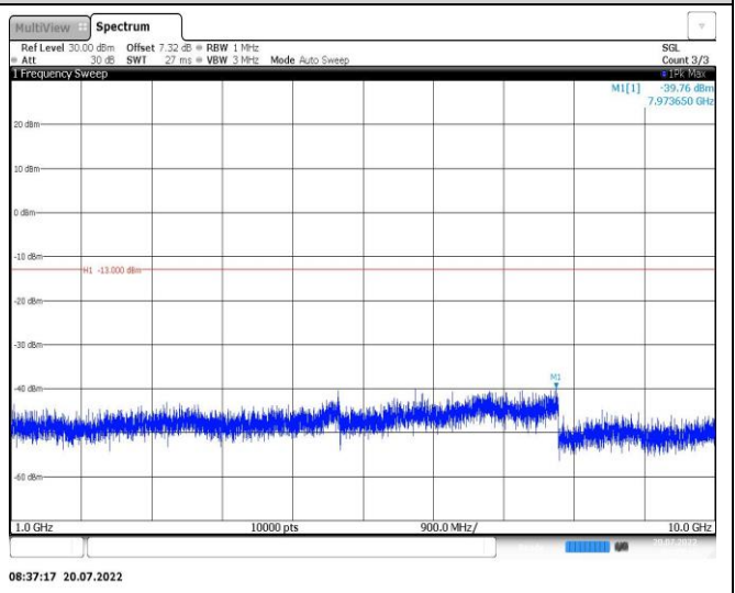
Band26-1.4MHz-16QAM-27033-1RB#0-Range2:1000~10000MHz
