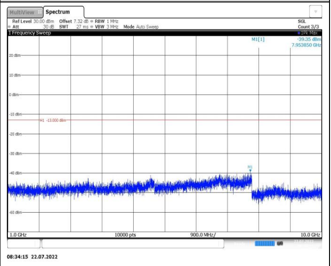
Band26-5MHz-QPSK-26715-1RB#0-Range2:1000~10000MHz
