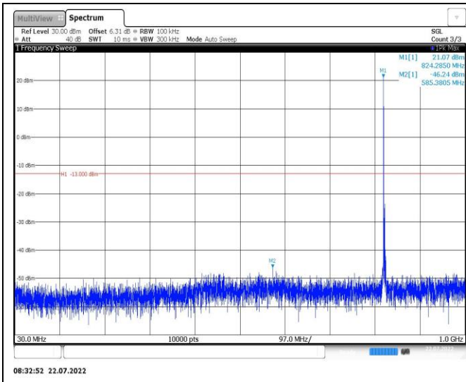
Band26-3MHz-QPSK-26915-1RB#0-Range1:30~1000MHz
