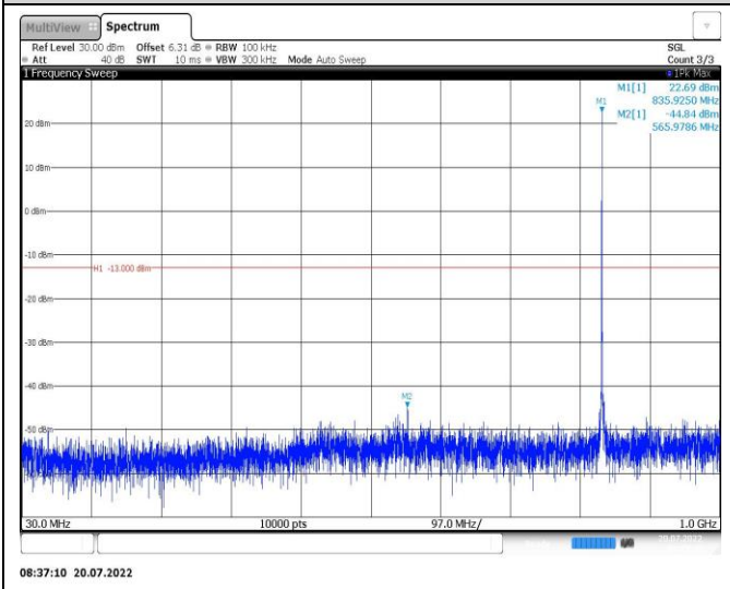
Band26-1.4MHz-16QAM-27033-1RB#0-Range1:30~1000MHz
