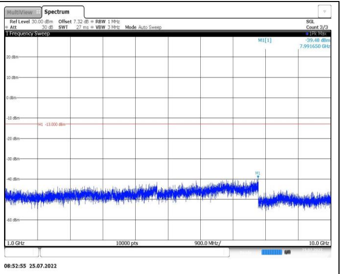
Band26-5MHz-16QAM-26915-1RB#0-Range2:1000~10000MHz
