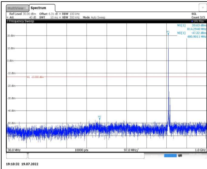
Band26-5MHz-QPSK-26740-1RB#0-Range1:30~1000MHz
