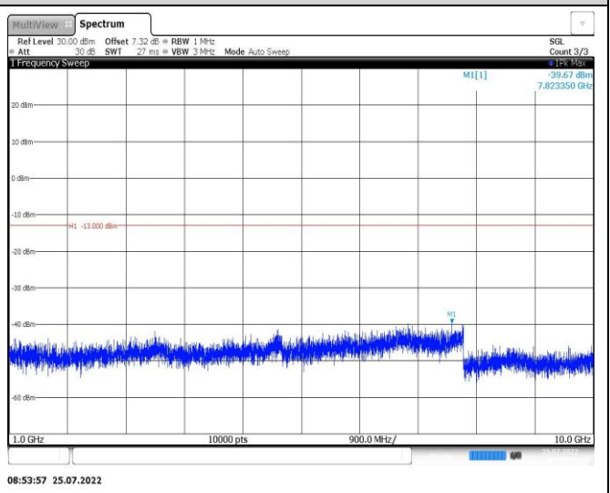
Band26-10MHz-QPSK-26740-1RB#0-Range2:1000~10000MHz
