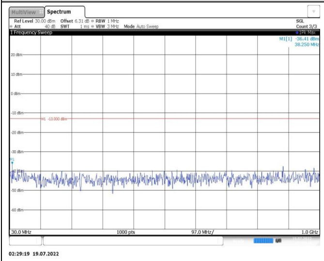
Band25-15MHz-QPSK-26615-1RB#0-Range1:30~1000MHz
