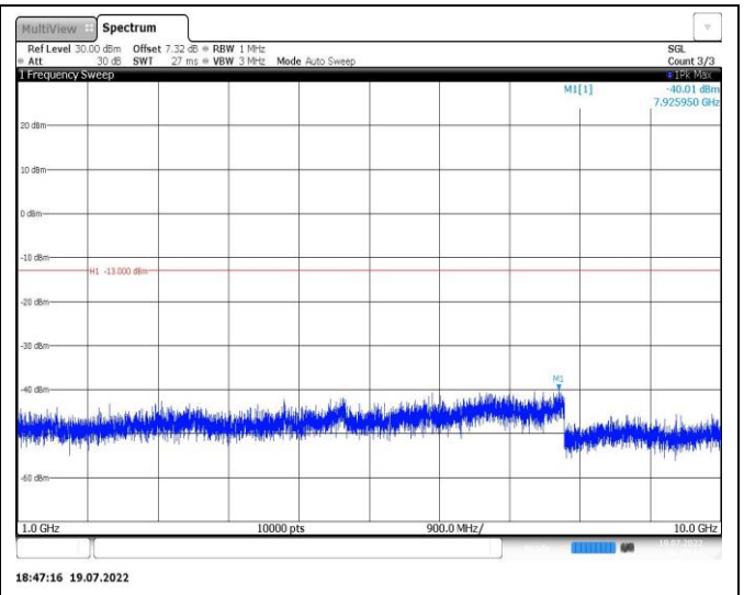
Band26-1.4MHz-16QAM-26740-1RB#0-Range2:1000~10000MHz
