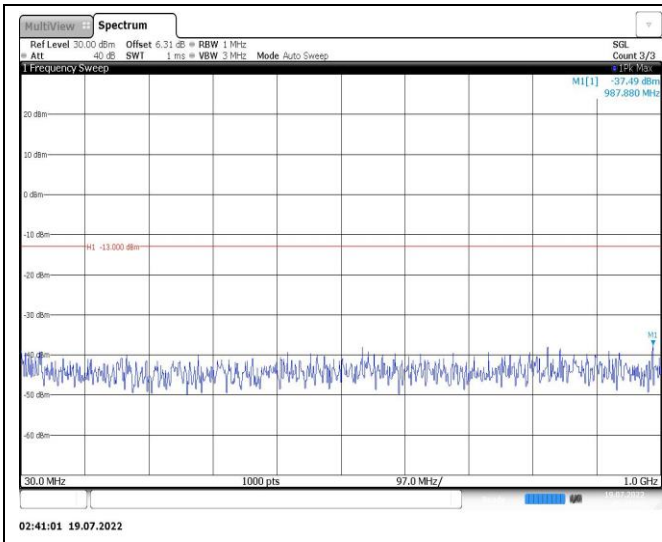
Band25-20MHz-16QAM-26365-1RB#0-Range1:30~1000MHz
