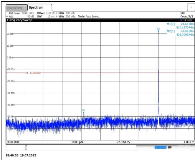
Band26-1.4MHz-QPSK-26740-1RB#0-Range1:30~1000MHz
