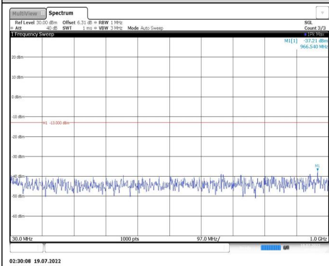
Band25-20MHz-QPSK-26140-1RB#0-Range1:30~1000MHz
