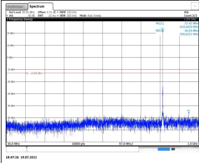
Band26-1.4MHz-QPSK-26783-1RB#0-Range1:30~1000MHz
