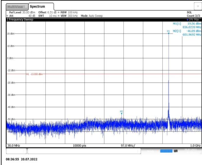
Band26-1.4MHz-QPSK-27033-1RB#0-Range1:30~1000MHz
