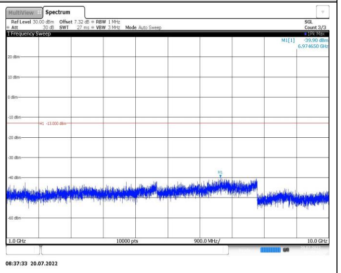
Band26-1.4MHz-16QAM-26697-1RB#0-Range2:1000~10000MHz
