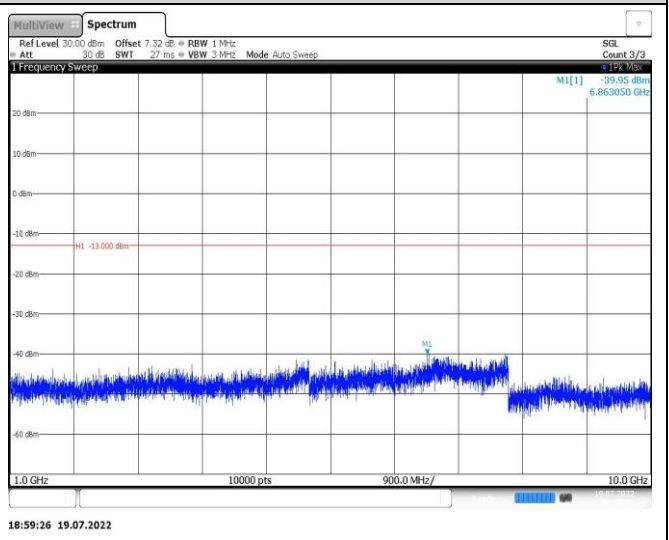
Band26-3MHz-16QAM-26775-1RB#0-Range2:1000~10000MHz
