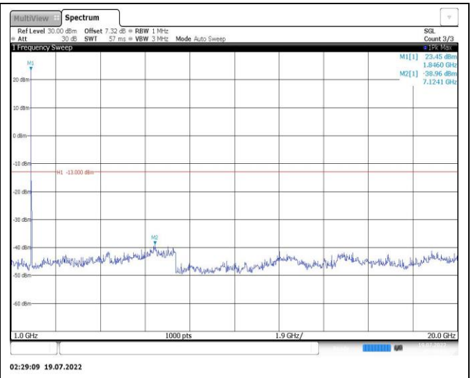
Band25-15MHz-16QAM-26365-1RB#0-Range2:1000~20000MHz
