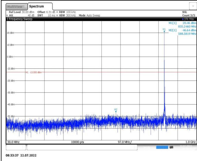
Band26-3MHz-16QAM-27025-1RB#0-Range1:30~1000MHz
