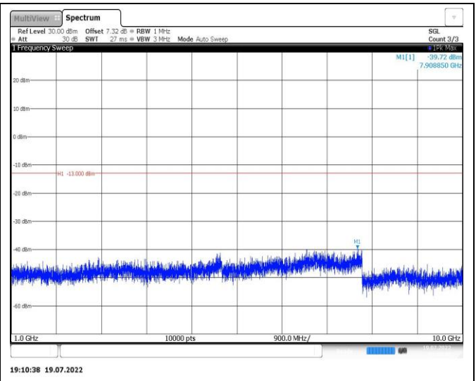
Band26-5MHz-QPSK-26740-1RB#0-Range2:1000~10000MHz
