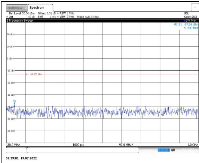
Band25-15MHz-16QAM-26365-1RB#0-Range1:30~1000MHz
