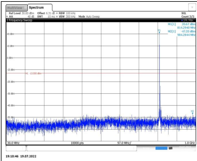
Band26-5MHz-16QAM-26740-1RB#0-Range1:30~1000MHz
