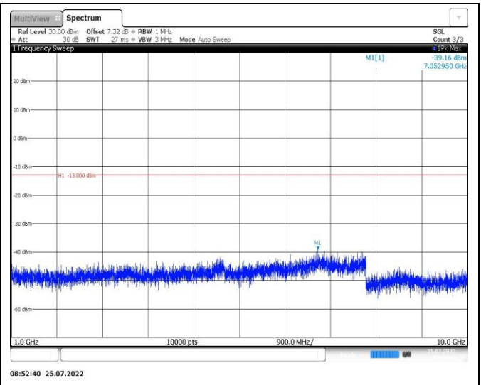
Band26-5MHz-QPSK-26915-1RB#0-Range2:1000~10000MHz
