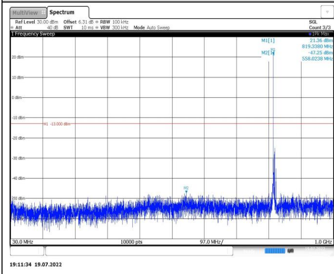
Band26-5MHz-QPSK-26815-1RB#0-Range1:30~1000MHz
