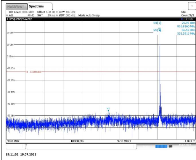
Band26-5MHz-QPSK-26765-1RB#0-Range1:30~1000MHz
