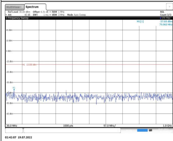
Band26-1.4MHz-QPSK-26697-1RB#0-Range1:30~1000MHz
