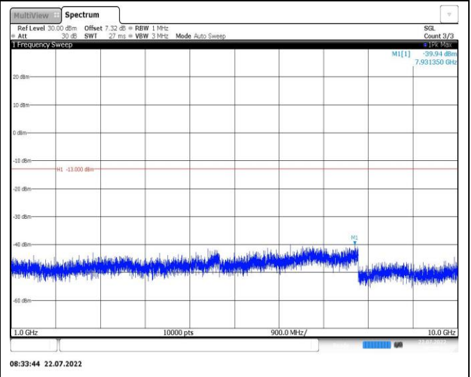
Band26-3MHz-16QAM-27025-1RB#0-Range2:1000~10000MHz
