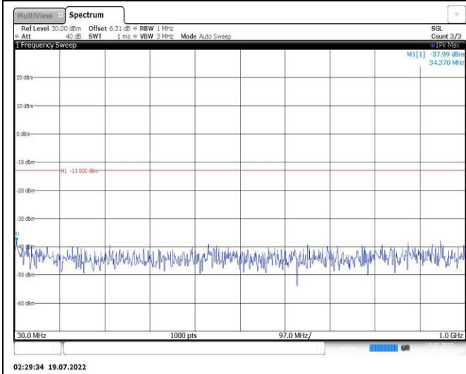
Band25-15MHz-16QAM-26615-1RB#0-Range1:30~1000MHz
