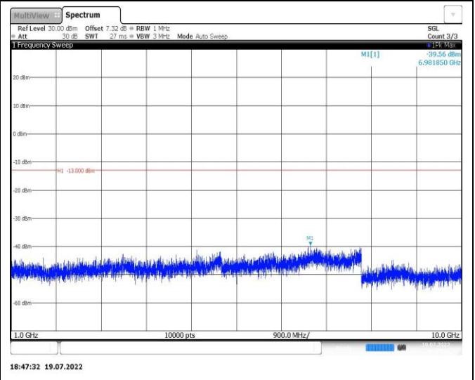
Band26-1.4MHz-QPSK-26783-1RB#0-Range2:1000~10000MHz
