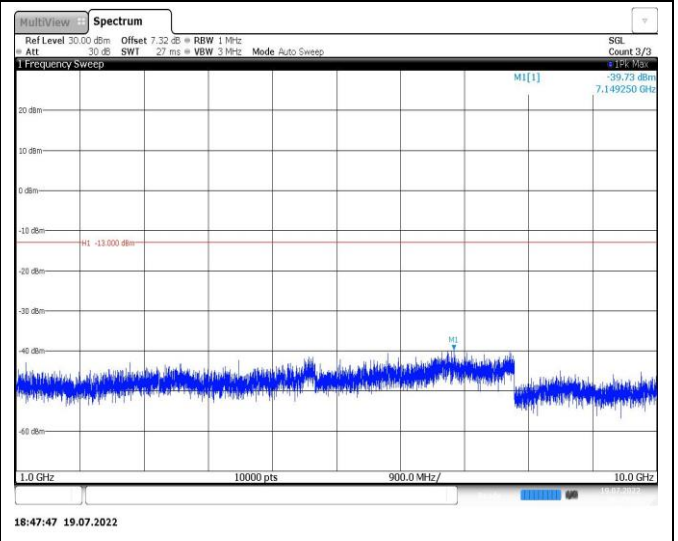
Band26-1.4MHz-16QAM-26783-1RB#0-Range2:1000~10000MHz
