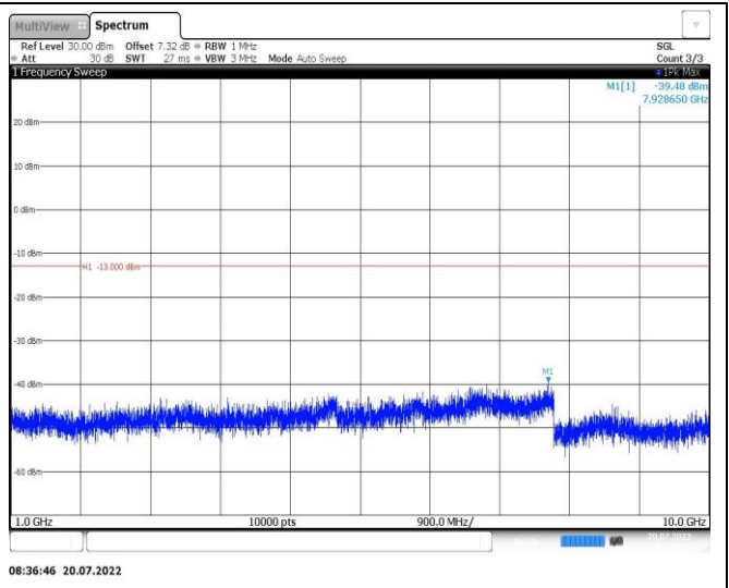
Band26-1.4MHz-16QAM-26915-1RB#0-Range2:1000~10000MHz
