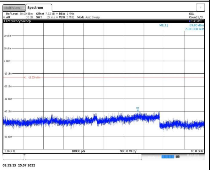
Band26-5MHz-16QAM-27015-1RB#0-Range2:1000~10000MHz
