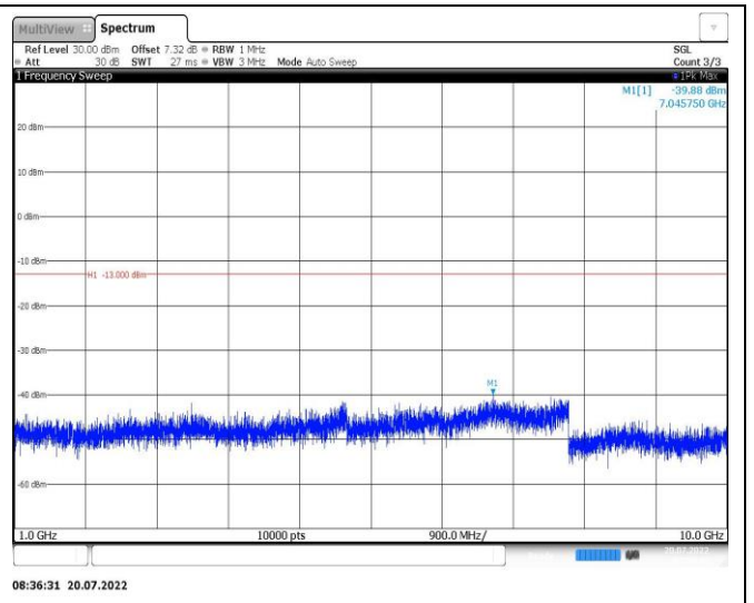
Band26-1.4MHz-QPSK-26915-1RB#0-Range2:1000~10000MHz
