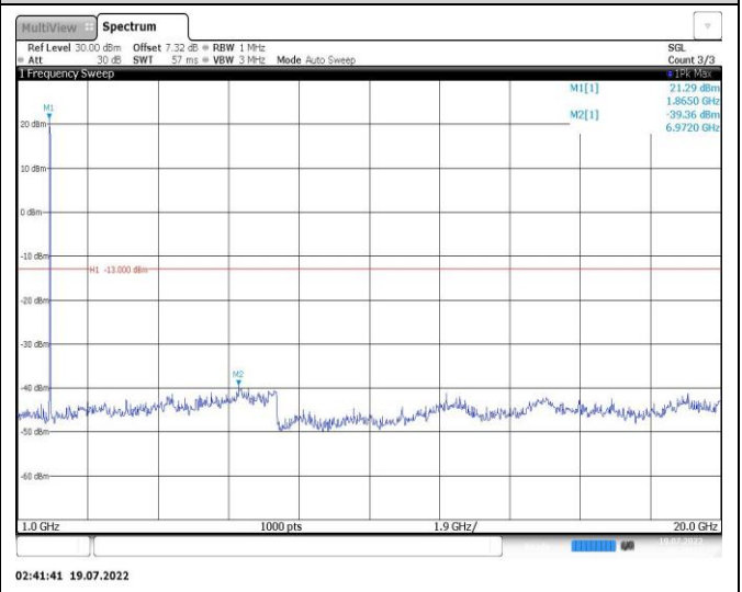
Band25-20MHz-16QAM-26590-1RB#0-Range2:1000~20000MHz
