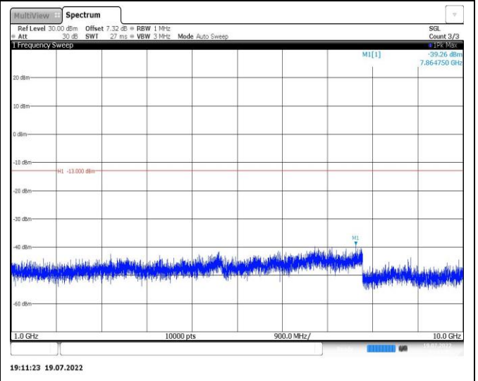
Band26-5MHz-16QAM-26765-1RB#0-Range2:1000~10000MHz
