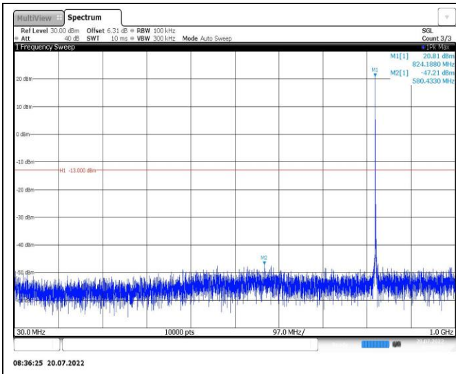
Band26-1.4MHz-QPSK-26915-1RB#0-Range1:30~1000MHz
