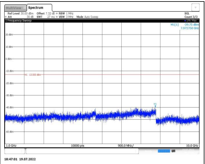
Band26-1.4MHz-QPSK-26740-1RB#0-Range2:1000~10000MHz
