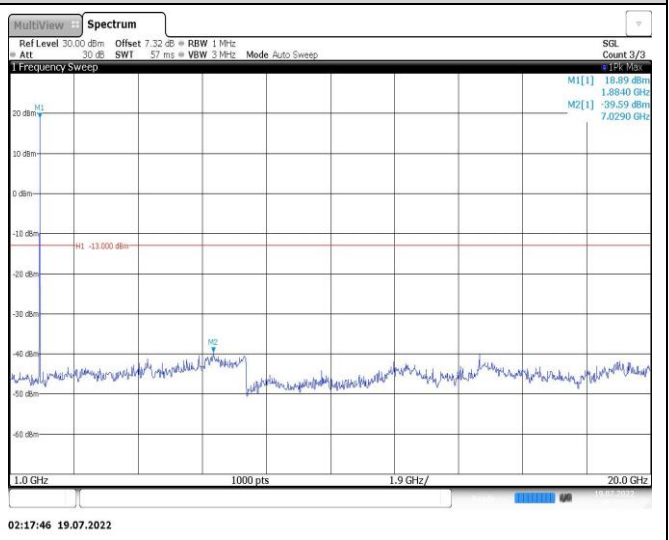
Band25-10MHz-16QAM-26640-1RB#0-Range2:1000~20000MHz
