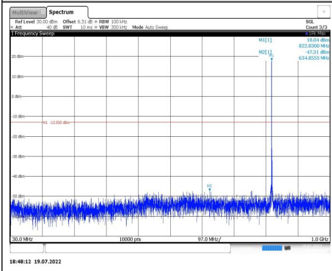
Band26-1.4MHz-16QAM-26797-1RB#0-Range1:30~1000MHz
