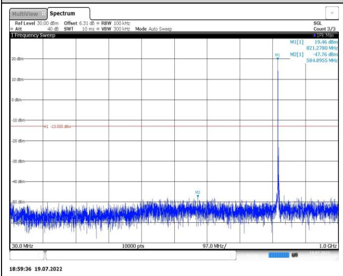
Band26-3MHz-QPSK-26805-1RB#0-Range1:30~1000MHz
