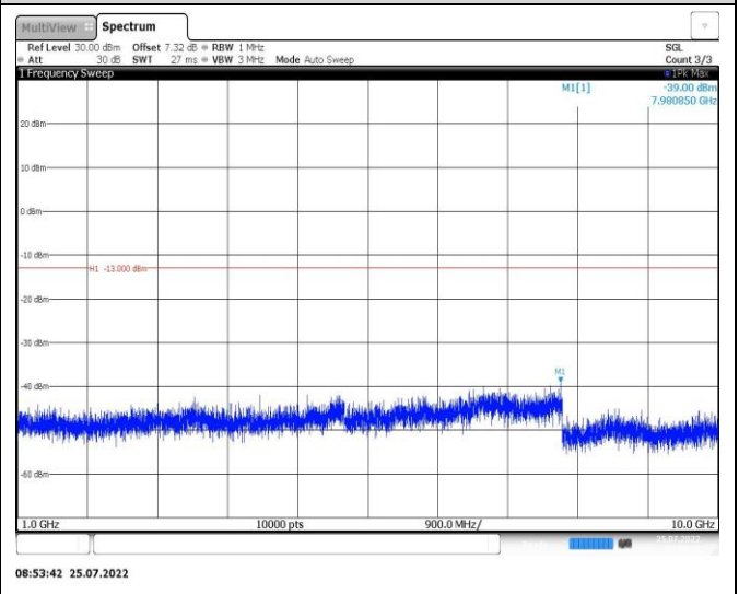
Band26-5MHz-16QAM-26715-1RB#0-Range2:1000~10000MHz
