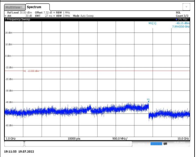
Band26-5MHz-16QAM-26815-1RB#0-Range2:1000~10000MHz
