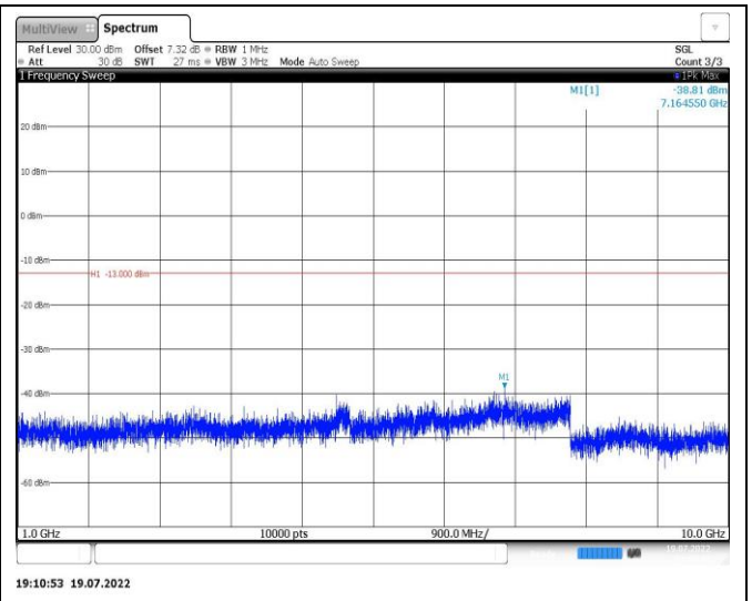
Band26-5MHz-16QAM-26740-1RB#0-Range2:1000~10000MHz
