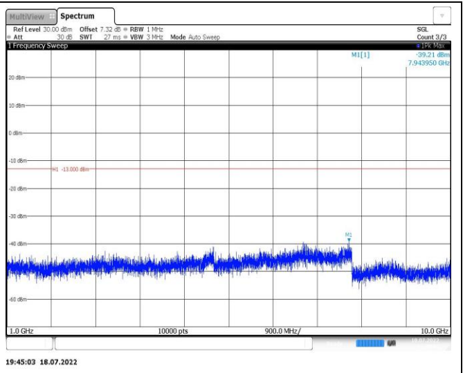
Band12-10MHz-16QAM-23095-1RB#0-Range2:1000~10000MHz
