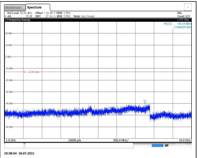
Band12-3MHz-QPSK-23095-1RB#0-Range2:1000~10000MHz
