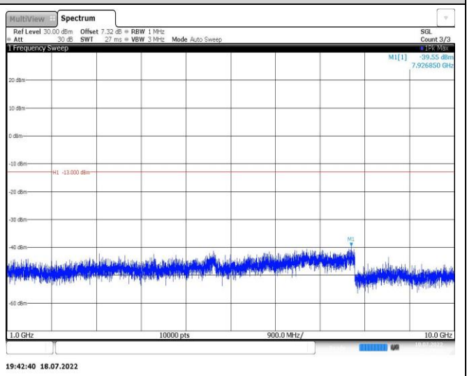
Band12-5MHz-16QAM-23035-1RB#0-Range2:1000~10000MHz
