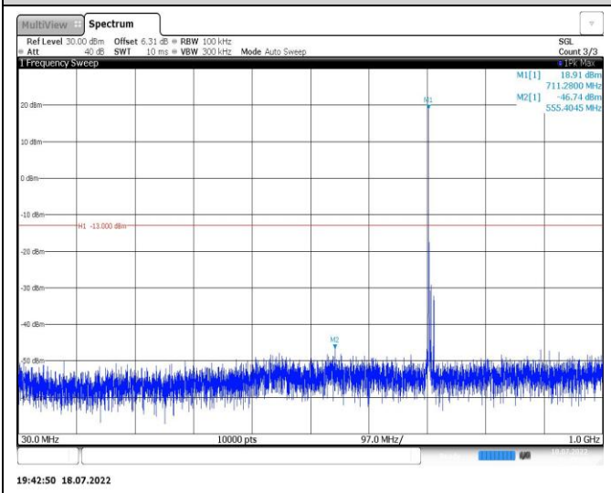
Band12-10MHz-QPSK-23060-1RB#0-Range1:30~1000MHz
