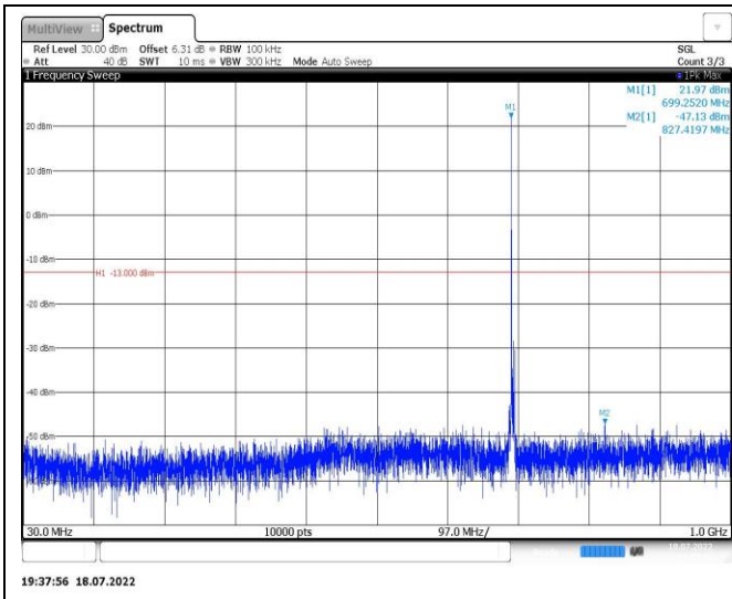
Band12-3MHz-QPSK-23095-1RB#0-Range1:30~1000MHz
