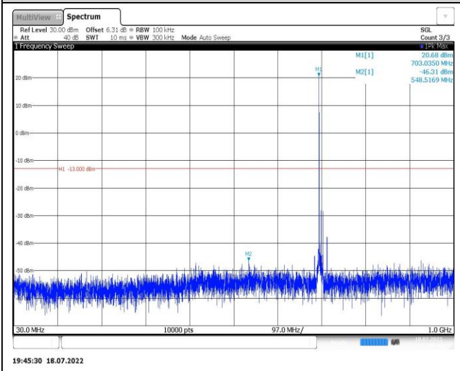
Band12-10MHz-16QAM-23130-1RB#0-Range1:30~1000MHz
