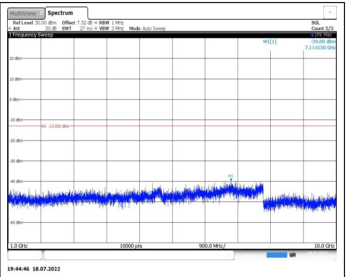
Band12-10MHz-QPSK-23095-1RB#0-Range2:1000~10000MHz
