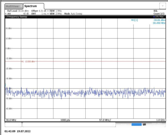
Band25-1.4MHz-16QAM-26683-1RB#0-Range1:30~1000MHz
