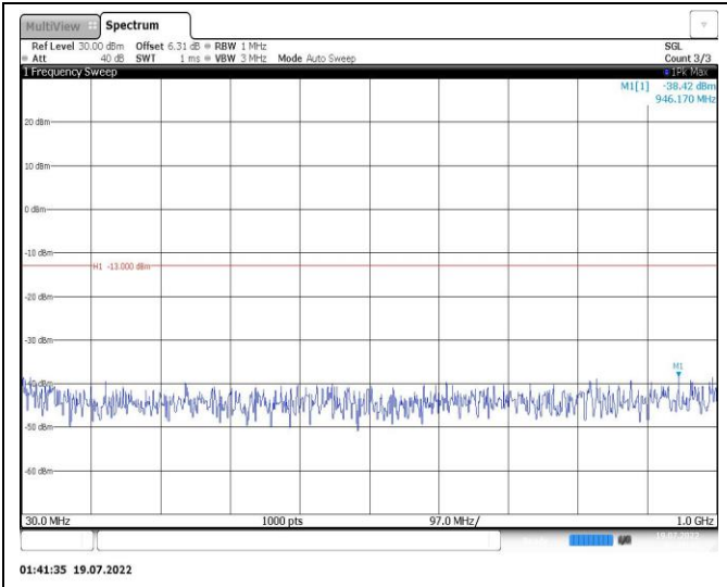
Band25-1.4MHz-16QAM-26365-1RB#0-Range1:30~1000MHz
