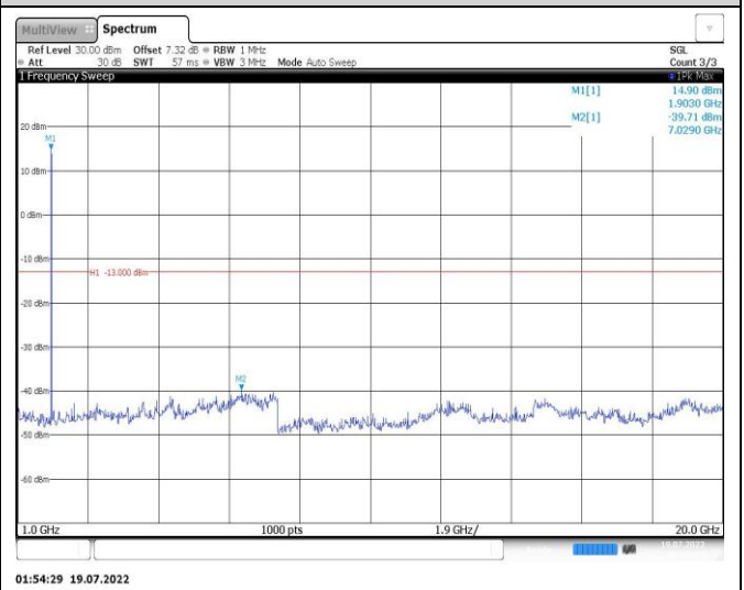
Band25-5MHz-QPSK-26065-1RB#0-Range2:1000~20000MHz
