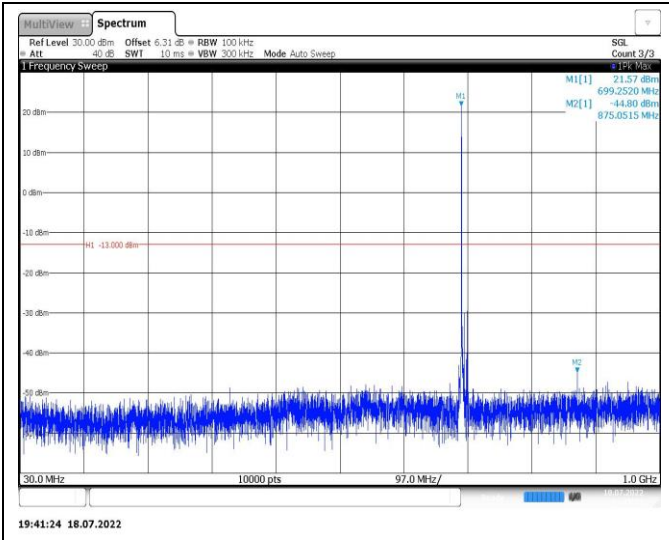
Band12-5MHz-QPSK-23095-1RB#0-Range1:30~1000MHz
