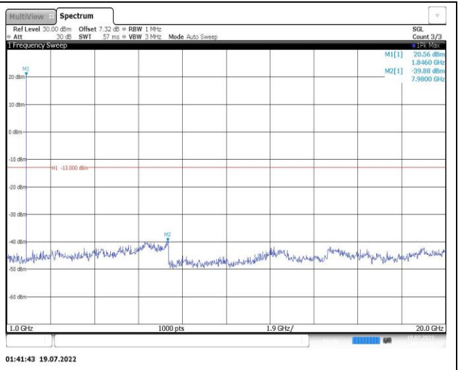
Band25-1.4MHz-16QAM-26365-1RB#0-Range2:1000~20000MHz
