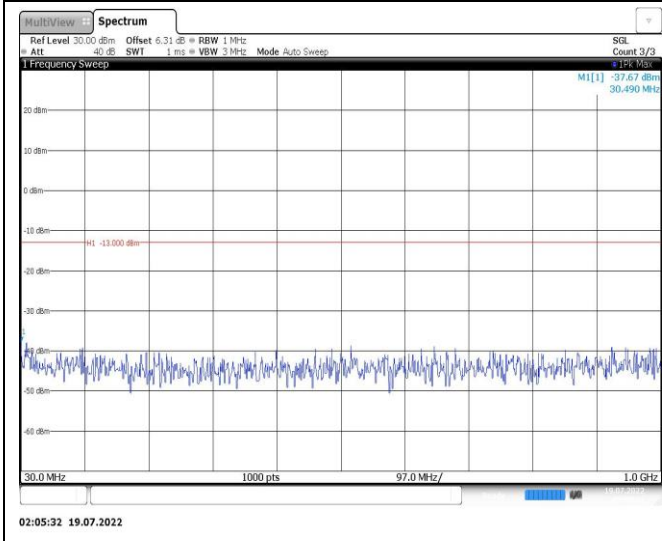
Band25-5MHz-QPSK-26665-1RB#0-Range1:30~1000MHz
