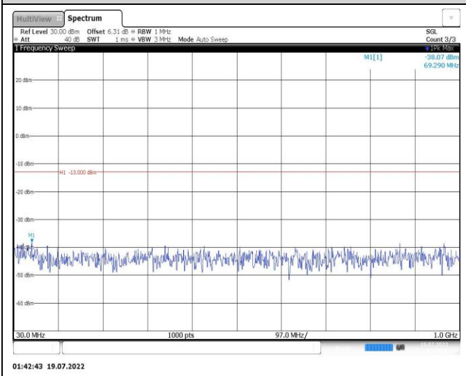
Band25-3MHz-QPSK-26055-1RB#0-Range1:30~1000MHz
