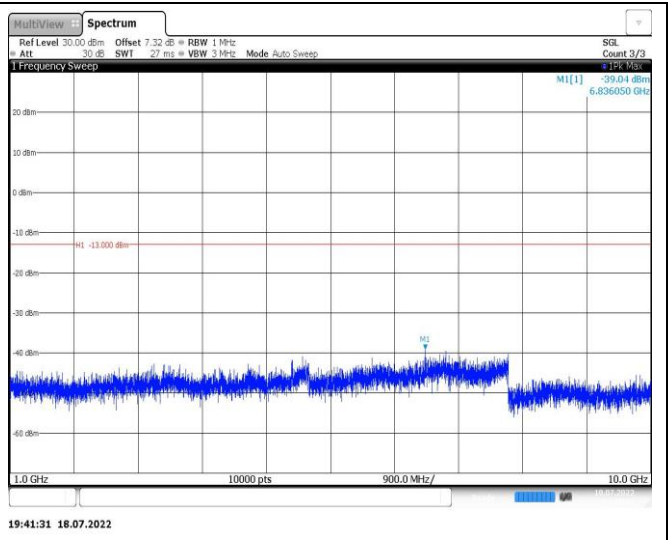
Band12-5MHz-QPSK-23095-1RB#0-Range2:1000~10000MHz
