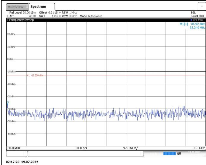
Band25-10MHz-QPSK-26640-1RB#0-Range1:30~1000MHz
