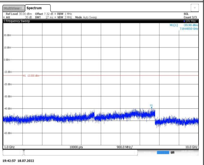
Band12-10MHz-QPSK-23060-1RB#0-Range2:1000~10000MHz
