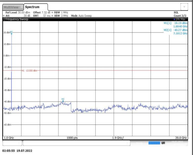
Band25-5MHz-16QAM-26665-1RB#0-Range2:1000~20000MHz
