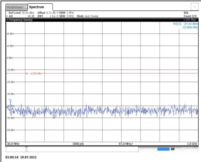
Band25-5MHz-16QAM-26365-1RB#0-Range1:30~1000MHz
