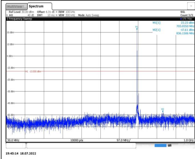
Band12-10MHz-QPSK-23130-1RB#0-Range1:30~1000MHz
