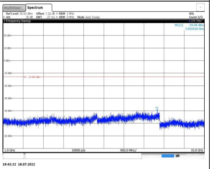
Band12-5MHz-16QAM-23155-1RB#0-Range2:1000~10000MHz
