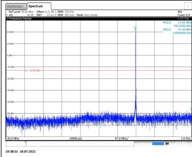
Band12-3MHz-QPSK-23165-1RB#0-Range1:30~1000MHz
