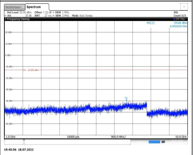
Band12-10MHz-16QAM-23060-1RB#0-Range2:1000~10000MHz
