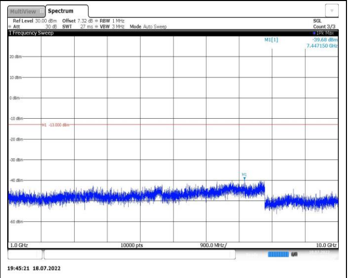
Band12-10MHz-QPSK-23130-1RB#0-Range2:1000~10000MHz
