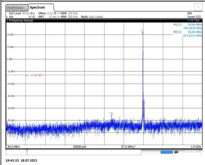
Band12-5MHz-16QAM-23155-1RB#0-Range1:30~1000MHz
