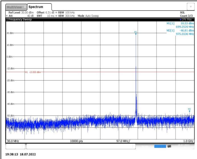
Band12-3MHz-16QAM-23095-1RB#0-Range1:30~1000MHz
