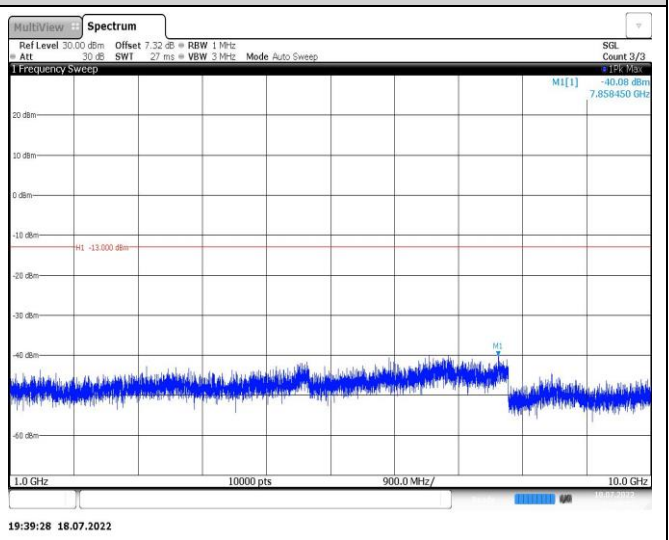
Band12-5MHz-QPSK-23035-1RB#0-Range2:1000~10000MHz
