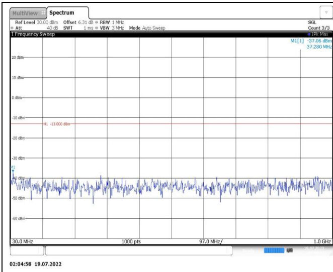
Band25-5MHz-QPSK-26365-1RB#0-Range1:30~1000MHz
