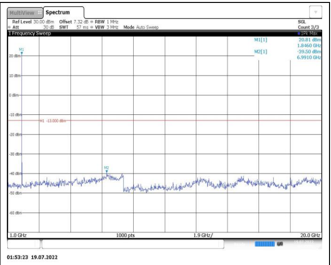
Band25-3MHz-16QAM-26365-1RB#0-Range2:1000~20000MHz
