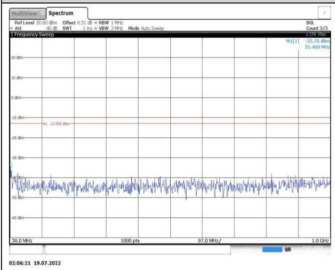
Band25-10MHz-QPSK-26090-1RB#0-Range1:30~1000MHz
