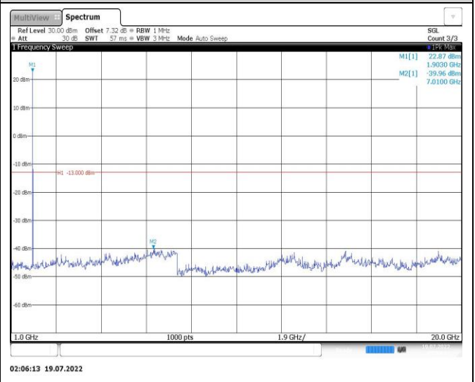
Band25-5MHz-16QAM-26065-1RB#0-Range2:1000~20000MHz
