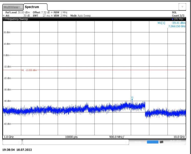
Band12-3MHz-16QAM-23165-1RB#0-Range2:1000~10000MHz
