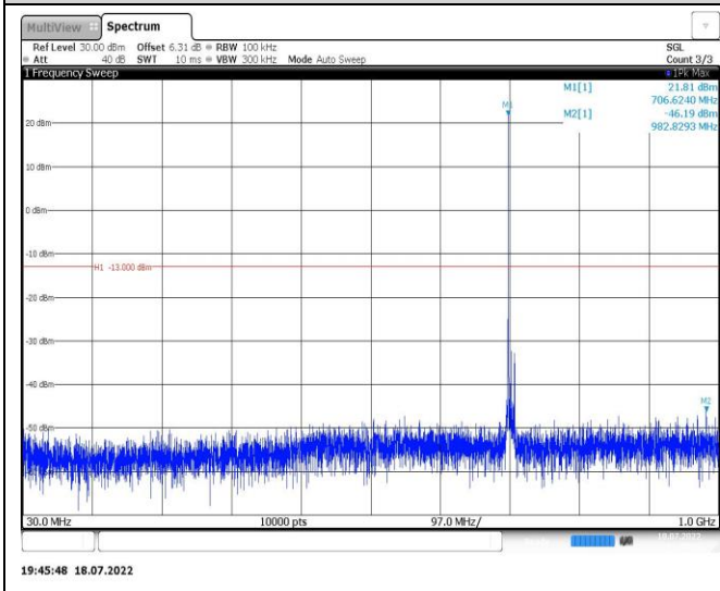
Band12-10MHz-16QAM-23060-1RB#0-Range1:30~1000MHz
