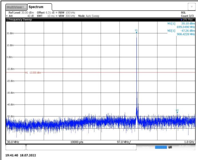
Band12-5MHz-16QAM-23095-1RB#0-Range1:30~1000MHz
