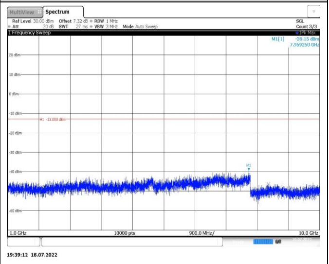
Band12-3MHz-16QAM-23025-1RB#0-Range2:1000~10000MHz
