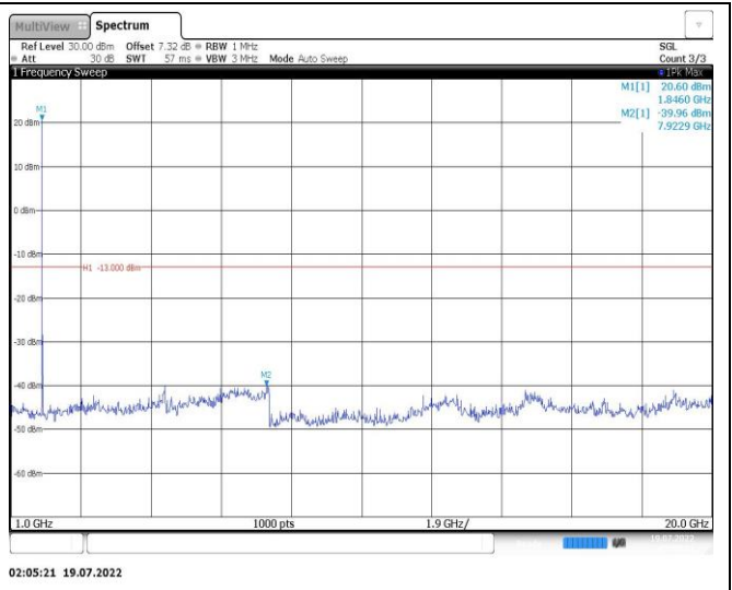
Band25-5MHz-16QAM-26365-1RB#0-Range2:1000~20000MHz
