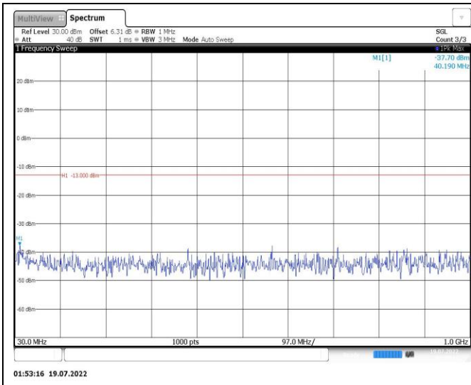
Band25-3MHz-16QAM-26365-1RB#0-Range1:30~1000MHz
