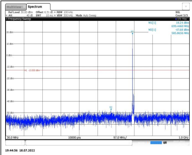
Band12-10MHz-16QAM-23095-1RB#0-Range1:30~1000MHz
