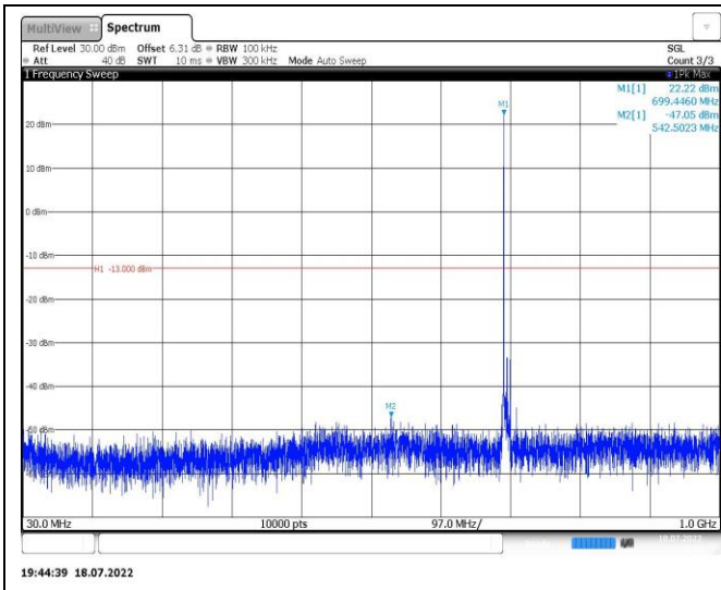
Band12-10MHz-QPSK-23095-1RB#0-Range1:30~1000MHz
