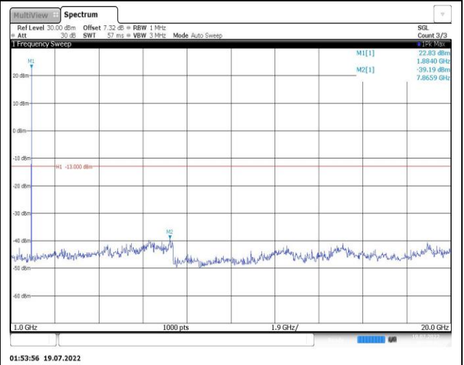
Band25-3MHz-16QAM-26675-1RB#0-Range2:1000~20000MHz
