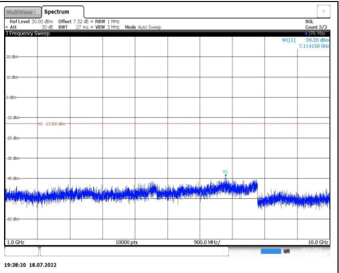
Band12-3MHz-16QAM-23095-1RB#0-Range2:1000~10000MHz
