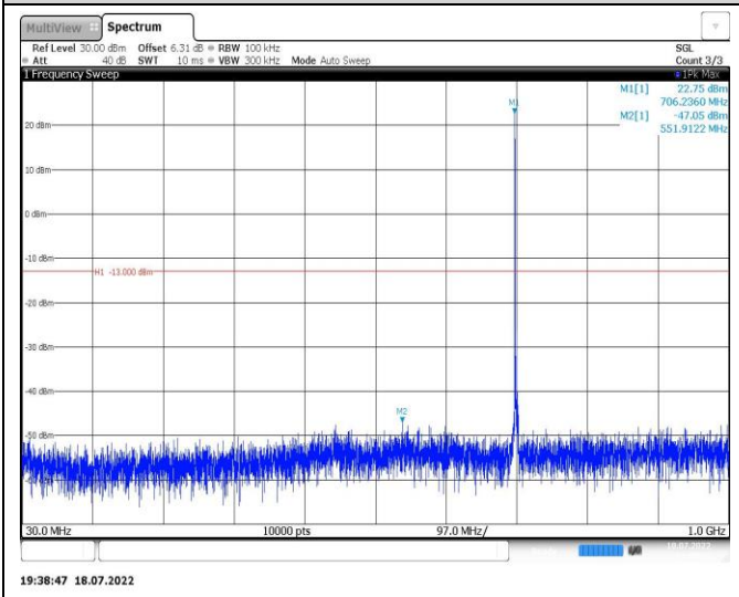
Band12-3MHz-16QAM-23165-1RB#0-Range1:30~1000MHz
