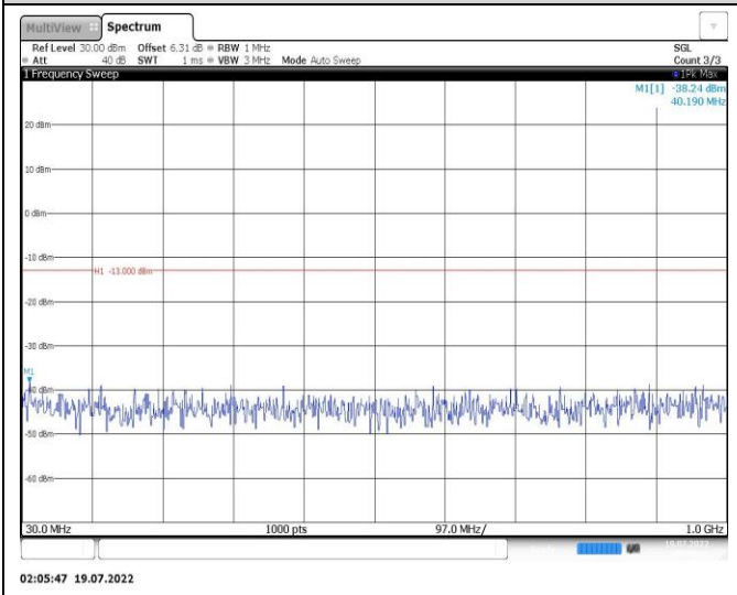
Band25-5MHz-16QAM-26665-1RB#0-Range1:30~1000MHz
