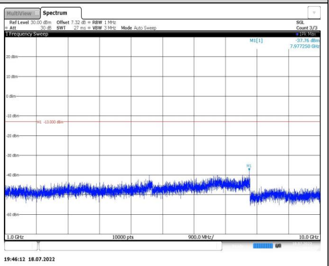
Band13-5MHz-QPSK-23205-1RB#0-Range2:1000~10000MHz
