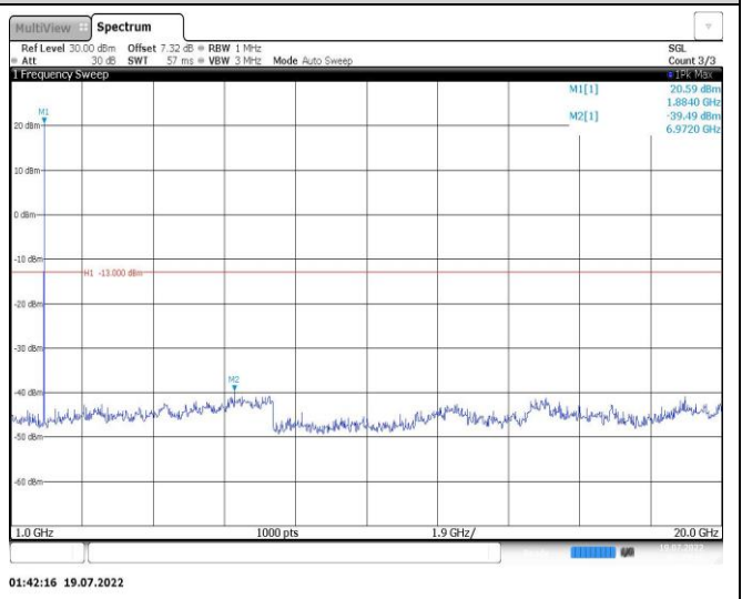
Band25-1.4MHz-16QAM-26683-1RB#0-Range2:1000~20000MHz
