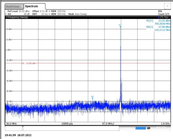
Band12-5MHz-QPSK-23155-1RB#0-Range1:30~1000MHz
