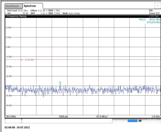
Band25-5MHz-16QAM-26065-1RB#0-Range1:30~1000MHz
