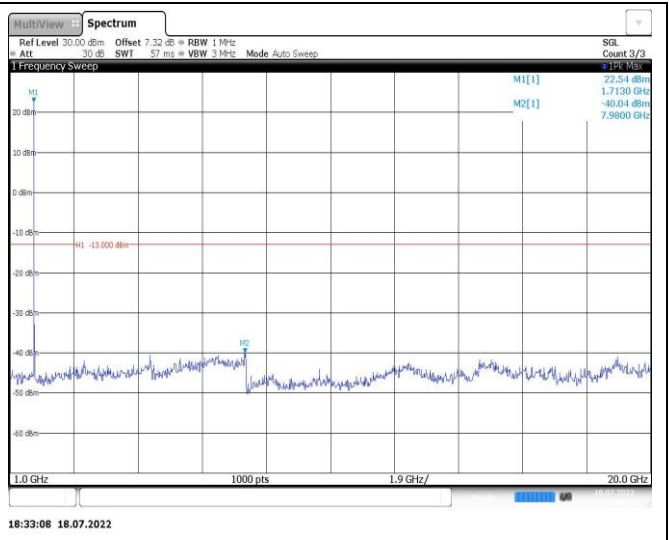
Band4-15MHz-QPSK-20175-1RB#0-Range2:1000~20000MHz
