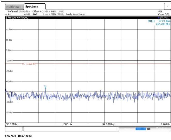
Band2-20MHz-16QAM-18900-1RB#0-Range1:30~1000MHz
