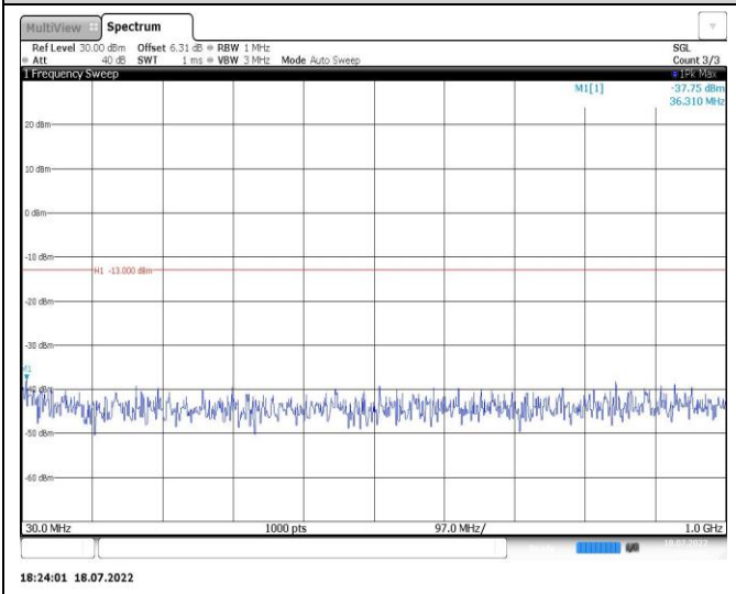
Band4-3MHz-16QAM-20385-1RB#0-Range1:30~1000MHz
