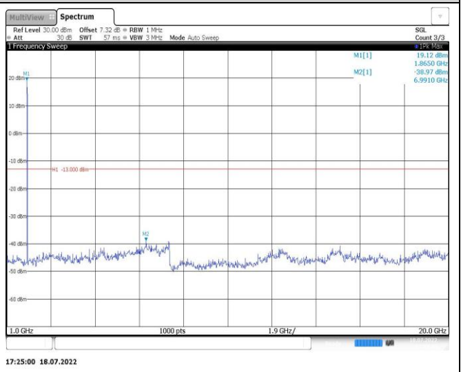
Band2-15MHz-16QAM-19125-1RB#0-Range2:1000~20000MHz
