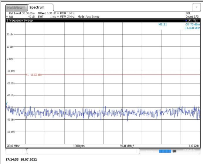
Band2-15MHz-16QAM-19125-1RB#0-Range1:30~1000MHz
