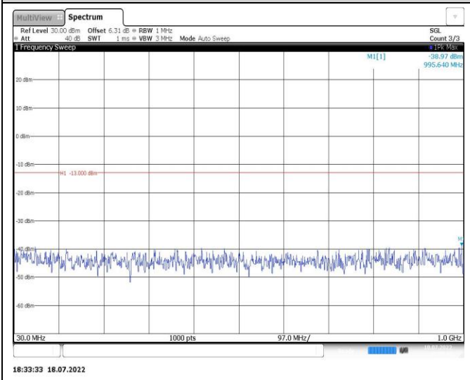
Band4-15MHz-QPSK-20325-1RB#0-Range1:30~1000MHz
