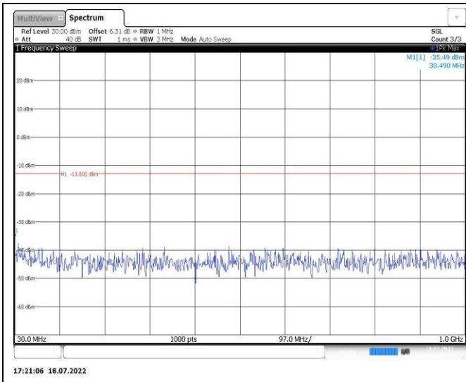
Band2-10MHz-16QAM-18900-1RB#0-Range1:30~1000MHz
