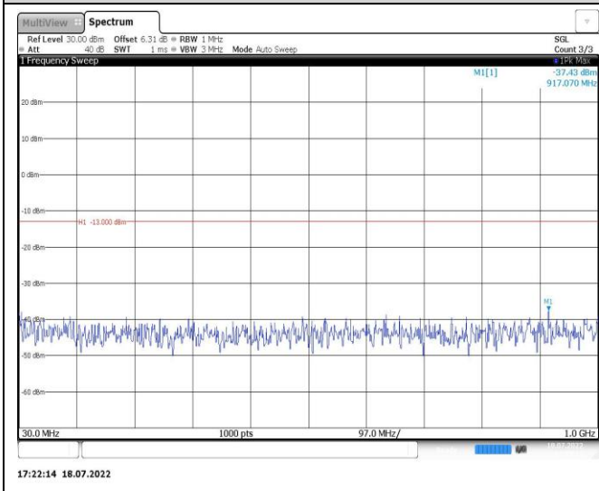
Band2-15MHz-QPSK-18675-1RB#0-Range1:30~1000MHz
