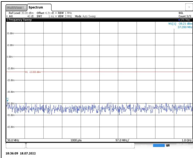
Band4-20MHz-QPSK-20175-1RB#0-Range1:30~1000MHz
