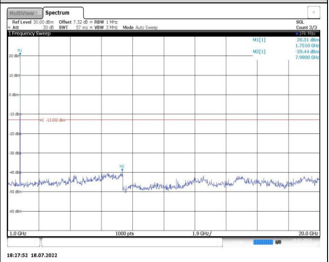
Band4-5MHz-16QAM-19975-1RB#0-Range2:1000~20000MHz
