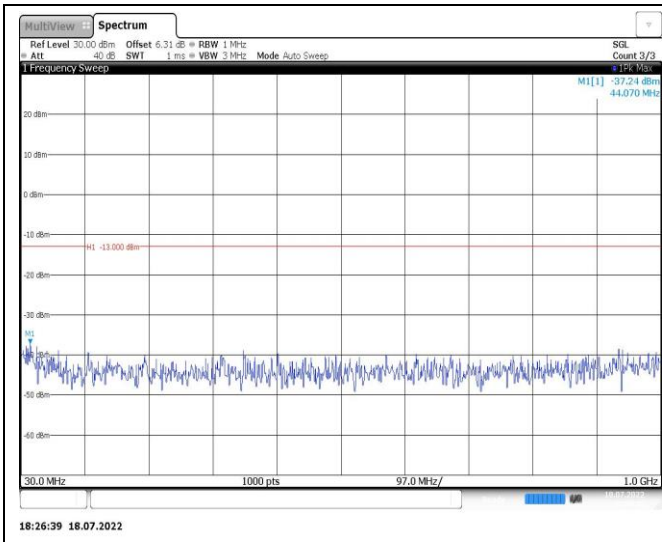
Band4-5MHz-QPSK-20175-1RB#0-Range1:30~1000MHz
