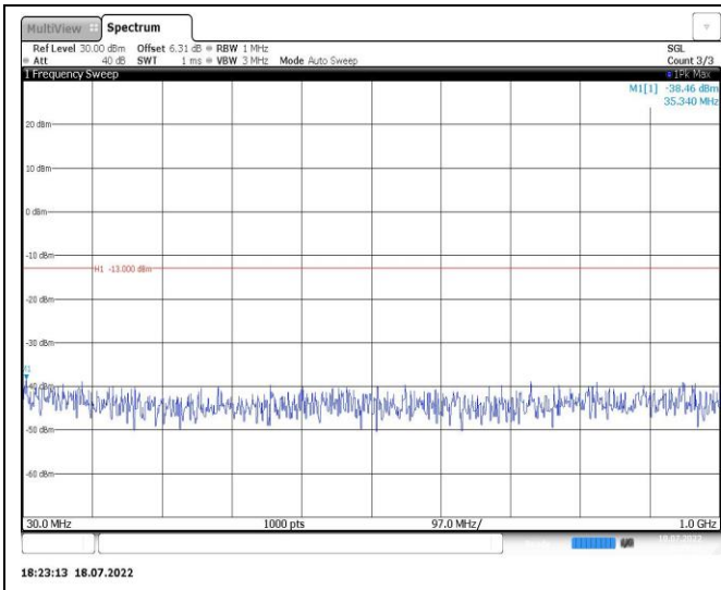
Band4-3MHz-QPSK-20175-1RB#0-Range1:30~1000MHz
