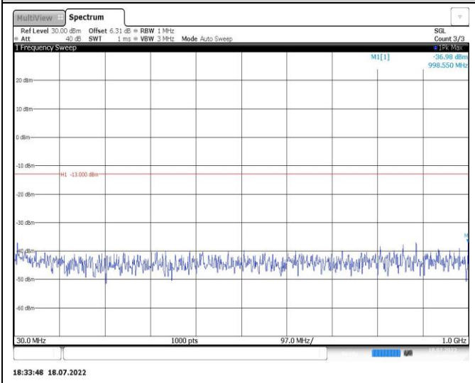
Band4-15MHz-16QAM-20325-1RB#0-Range1:30~1000MHz
