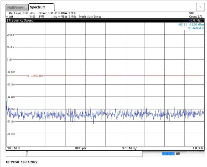
Band4-10MHz-QPSK-20175-1RB#0-Range1:30~1000MHz
