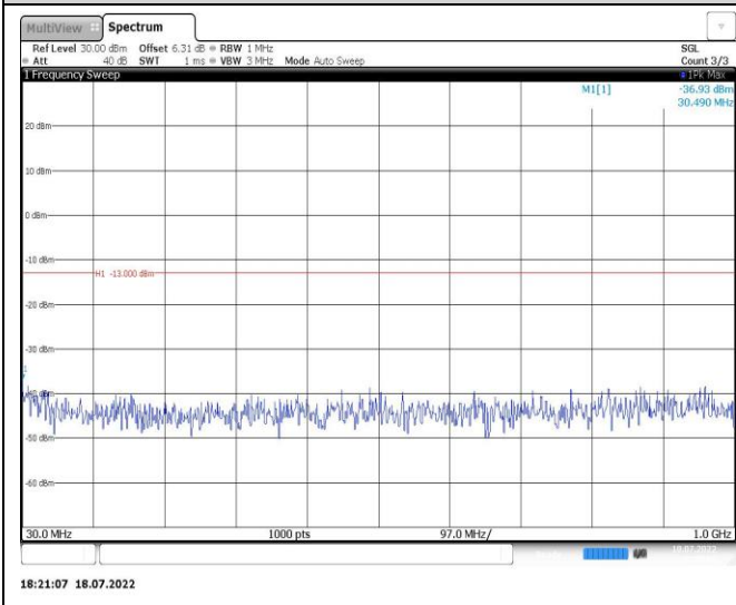
Band4-1.4MHz-16QAM-19957-1RB#0-Range1:30~1000MHz
