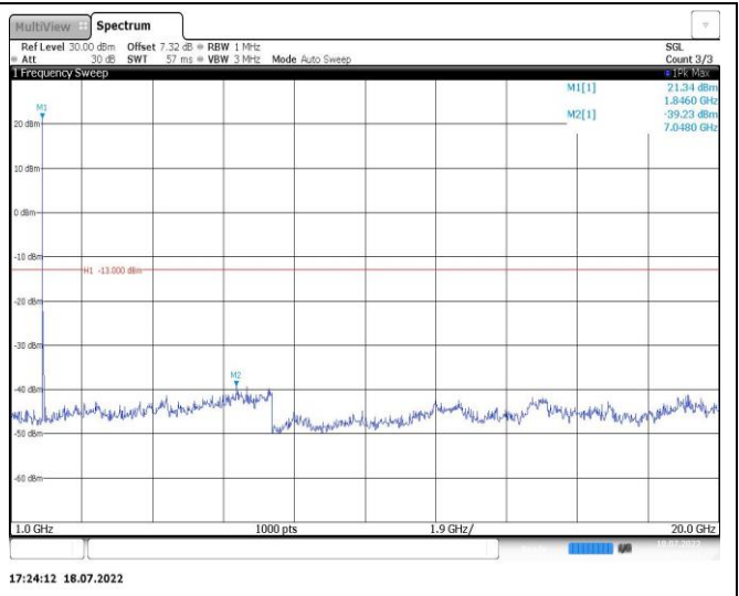
Band2-15MHz-QPSK-18900-1RB#0-Range2:1000~20000MHz
