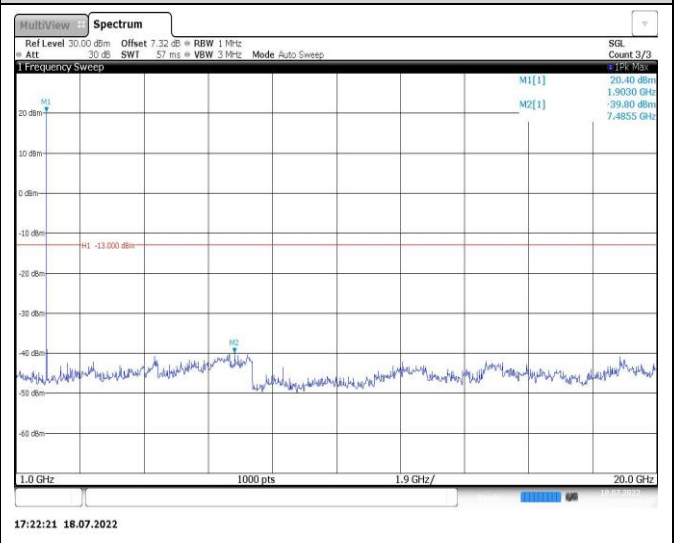
Band2-15MHz-QPSK-18675-1RB#0-Range2:1000~20000MHz
