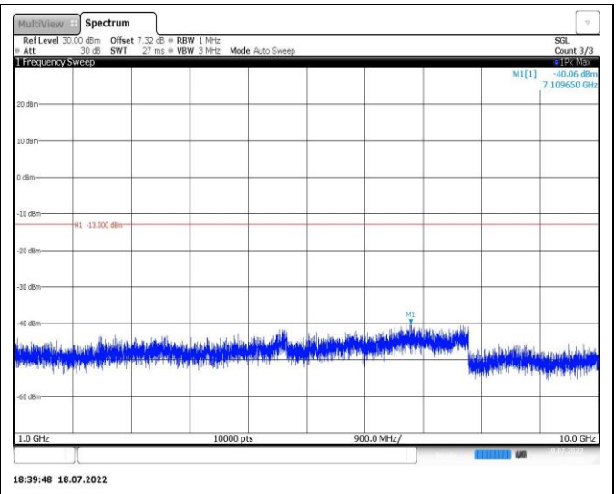
Band5-1.4MHz-QPSK-20525-1RB#0-Range2:1000~10000MHz
