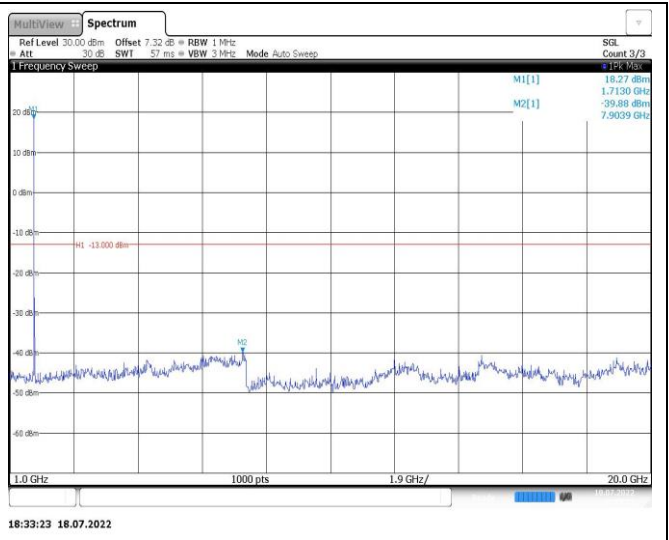
Band4-15MHz-16QAM-20175-1RB#0-Range2:1000~20000MHz
