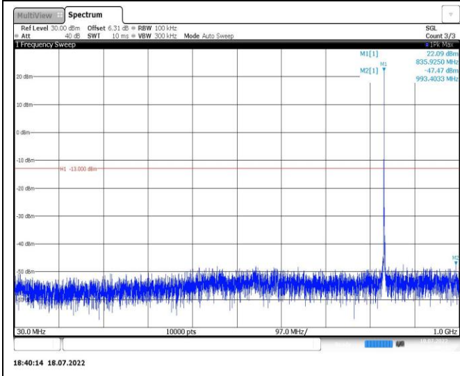
Band5-1.4MHz-QPSK-20643-1RB#0-Range1:30~1000MHz
