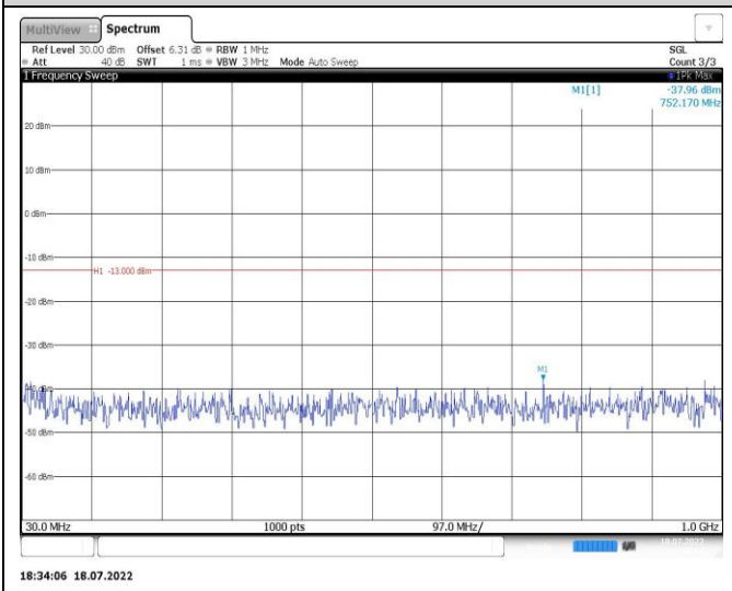
Band4-15MHz-16QAM-20025-1RB#0-Range1:30~1000MHz
