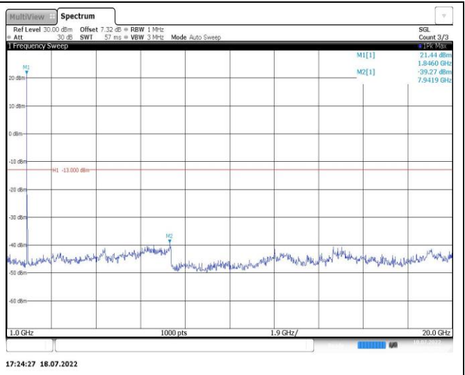
Band2-15MHz-16QAM-18900-1RB#0-Range2:1000~20000MHz
