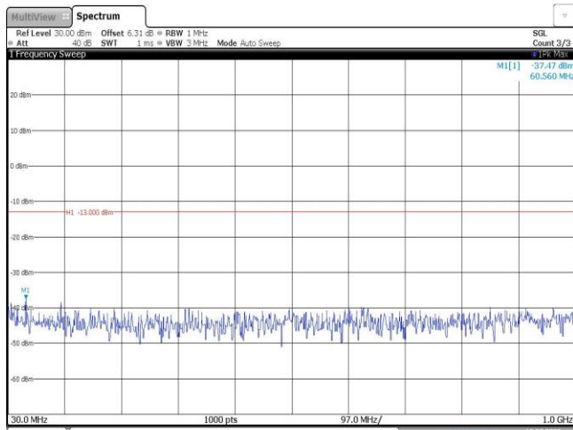
Band2-1.4MHz-16QAM-18900-1RB#0-Range1:30~1000MHz
