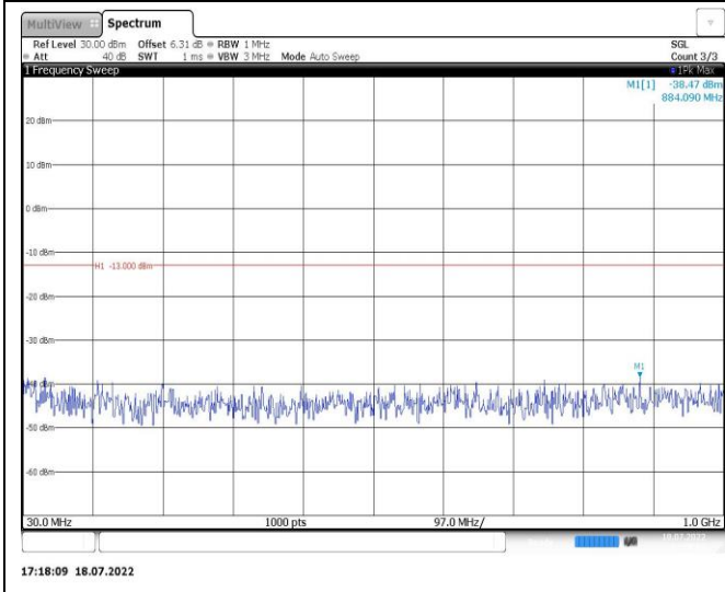
Band2-5MHz-QPSK-19175-1RB#0-Range1:30~1000MHz
