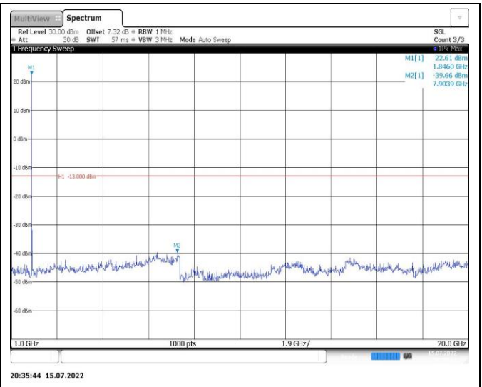
Band2-3MHz-16QAM-18900-1RB#0-Range2:1000~20000MHz
