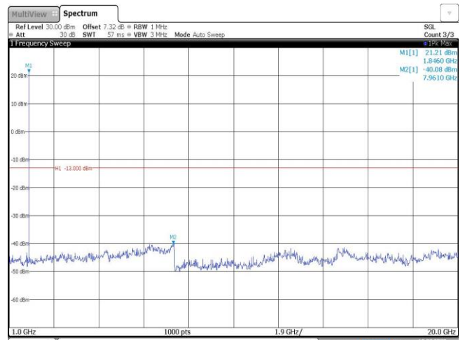
Band2-1.4MHz-QPSK-18607-1RB#0-Range2:1000~20000MHz
