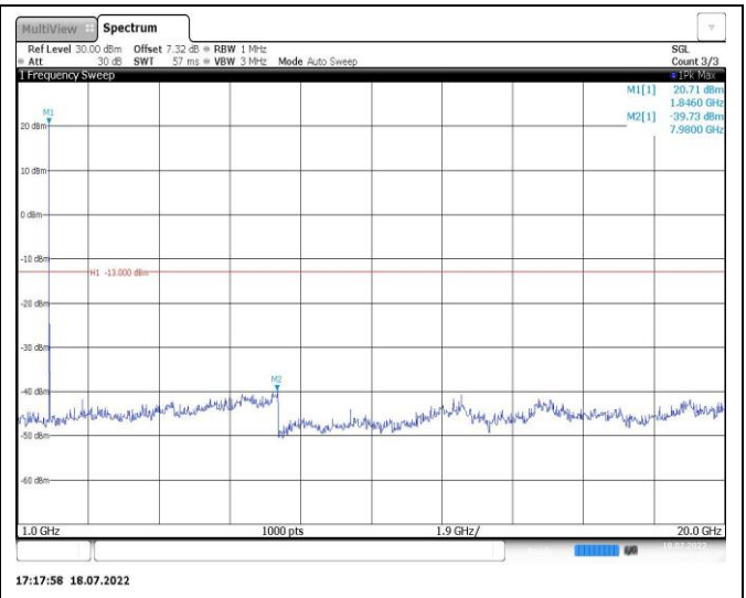
Band2-5MHz-16QAM-18900-1RB#0-Range2:1000~20000MHz
