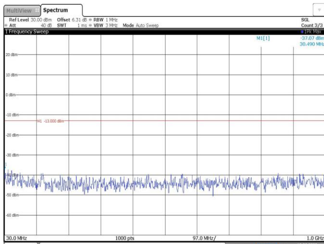
Band2-1.4MHz-16QAM-19193-1RB#0-Range1:30~1000MHz
