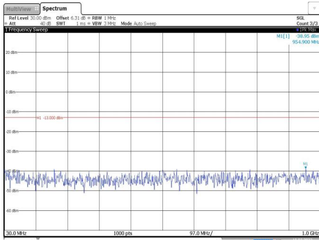
Band2-1.4MHz-16QAM-18607-1RB#0-Range1:30~1000MHz
