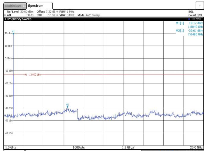
Band2-1.4MHz-16QAM-18900-1RB#0-Range2:1000~20000MHz
