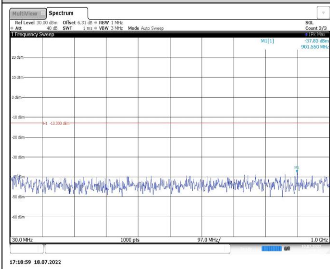
Band2-10MHz-QPSK-18650-1RB#0-Range1:30~1000MHz
