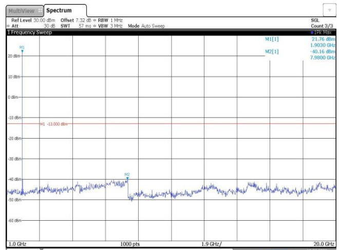
Band2-1.4MHz-16QAM-19193-1RB#0-Range2:1000~20000MHz
