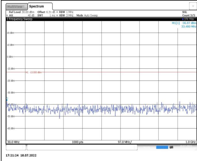
Band2-10MHz-QPSK-19150-1RB#0-Range1:30~1000MHz
