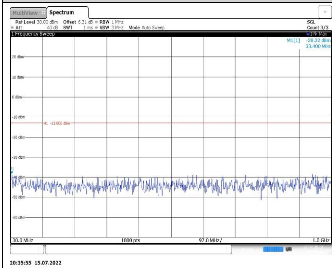
Band2-3MHz-QPSK-19185-1RB#0-Range1:30~1000MHz
