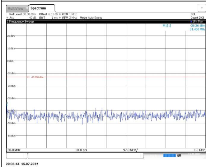
Band2-5MHz-QPSK-18625-1RB#0-Range1:30~1000MHz
