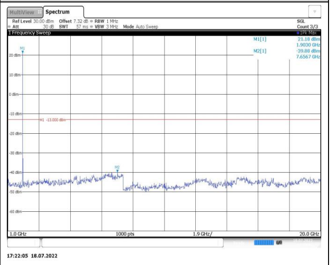
Band2-10MHz-16QAM-18650-1RB#0-Range2:1000~20000MHz
