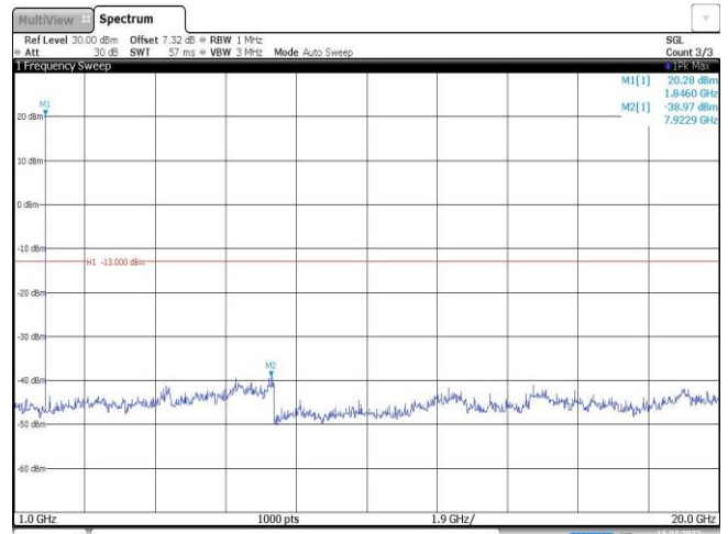
Band2-1.4MHz-16QAM-18607-1RB#0-Range2:1000~20000MHz
