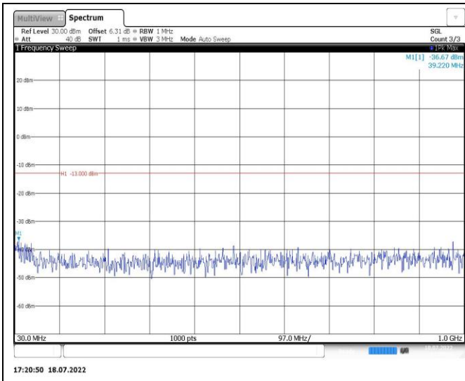
Band2-10MHz-QPSK-18900-1RB#0-Range1:30~1000MHz
