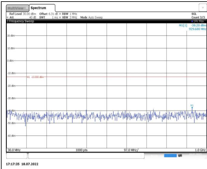
Band2-5MHz-QPSK-18900-1RB#0-Range1:30~1000MHz
