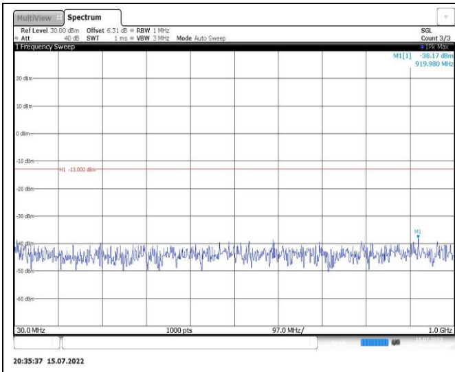
Band2-3MHz-16QAM-18900-1RB#0-Range1:30~1000MHz
