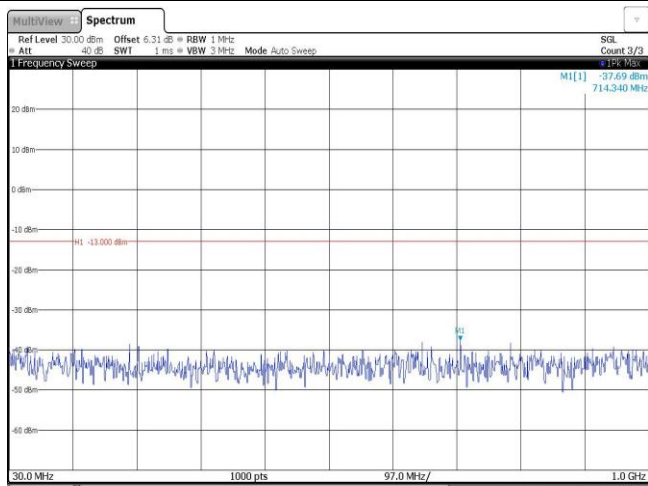
Band2-1.4MHz-QPSK-18900-1RB#0-Range1:30~1000MHz
