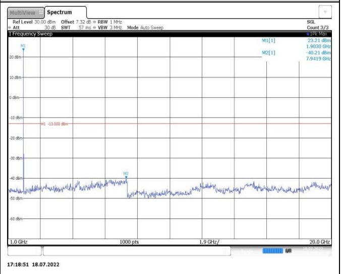
Band2-5MHz-16QAM-18625-1RB#0-Range2:1000~20000MHz
