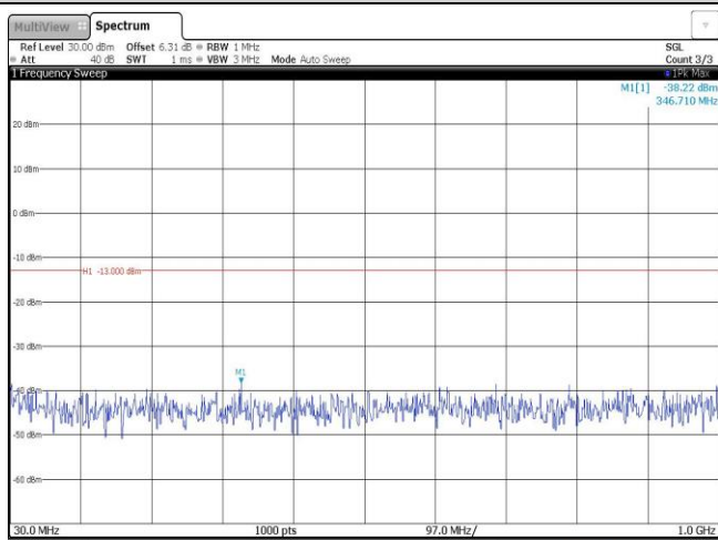
Band2-1.4MHz-QPSK-19193-1RB#0-Range1:30~1000MHz
