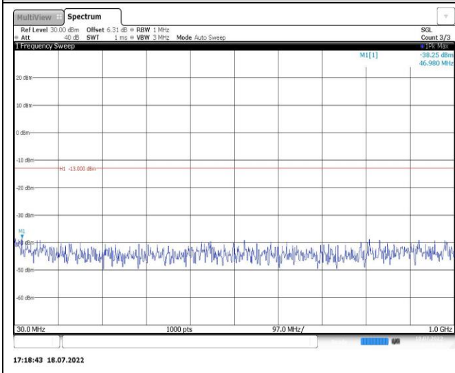
Band2-5MHz-16QAM-18625-1RB#0-Range1:30~1000MHz
