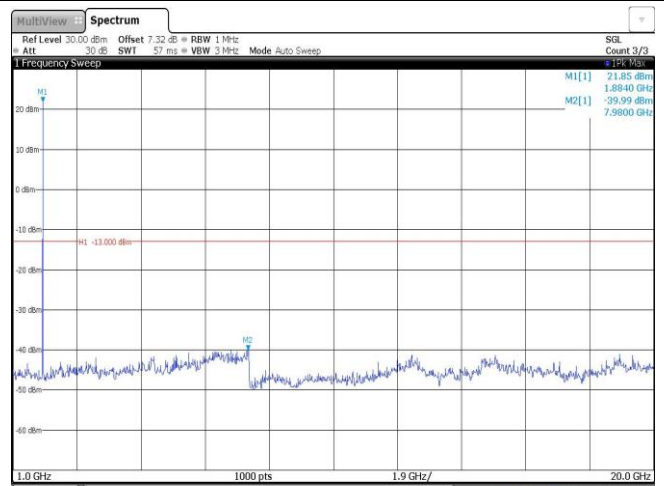
Band2-1.4MHz-QPSK-18900-1RB#0-Range2:1000~20000MHz
