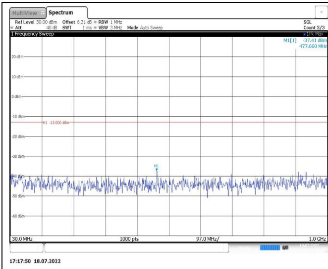
Band2-5MHz-16QAM-18900-1RB#0-Range1:30~1000MHz
