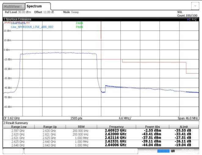
Band38-20MHz-16QAM-38150-100RB#0
