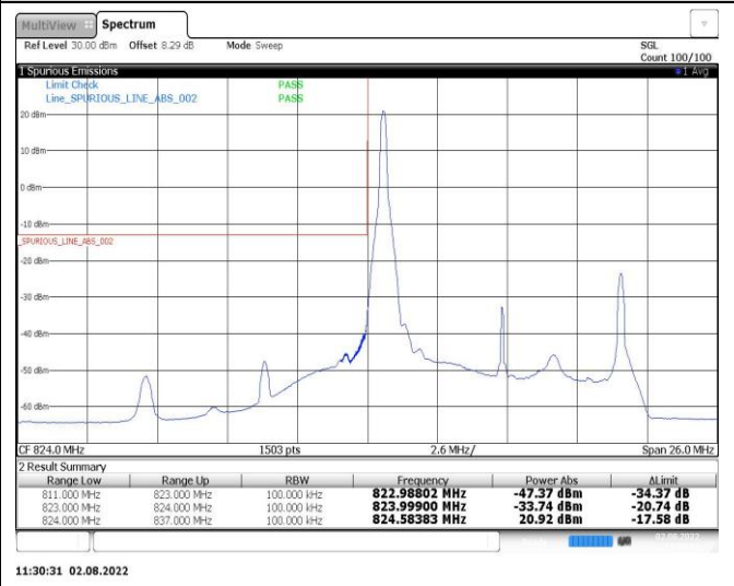
Band26-10MHz-16QAM-26740-1RB#0
