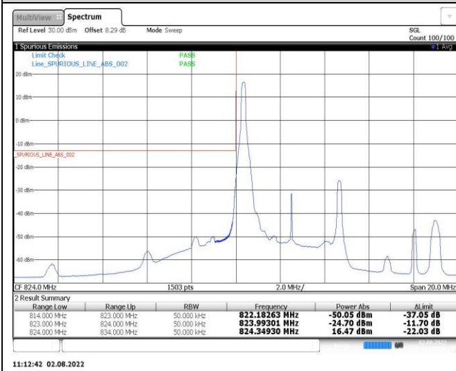
Band26-5MHz-16QAM-27015-1RB#24
