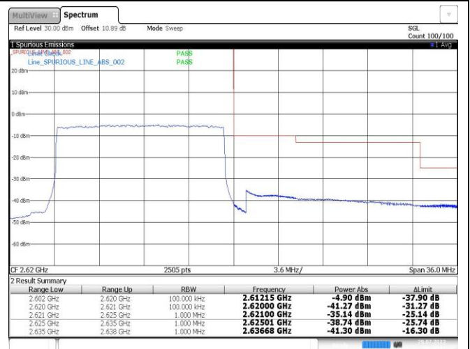
Band38-15MHz-16QAM-38175-75RB#0
