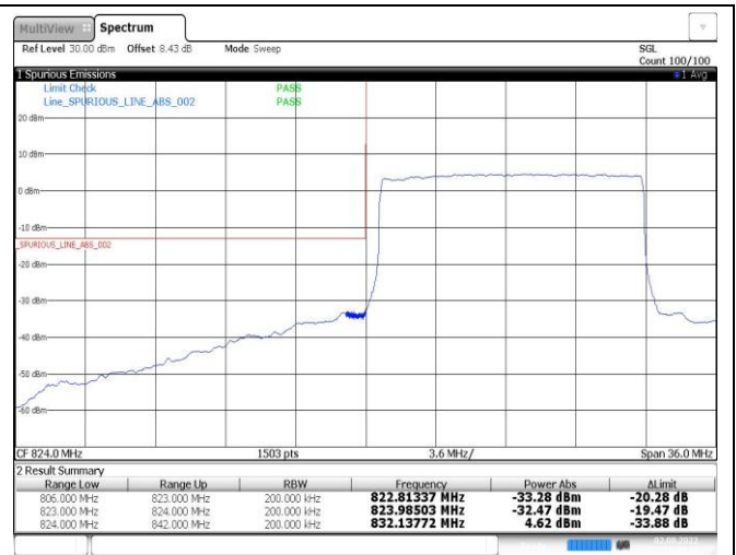
Band26-15MHz-16QAM-26865-75RB#0
