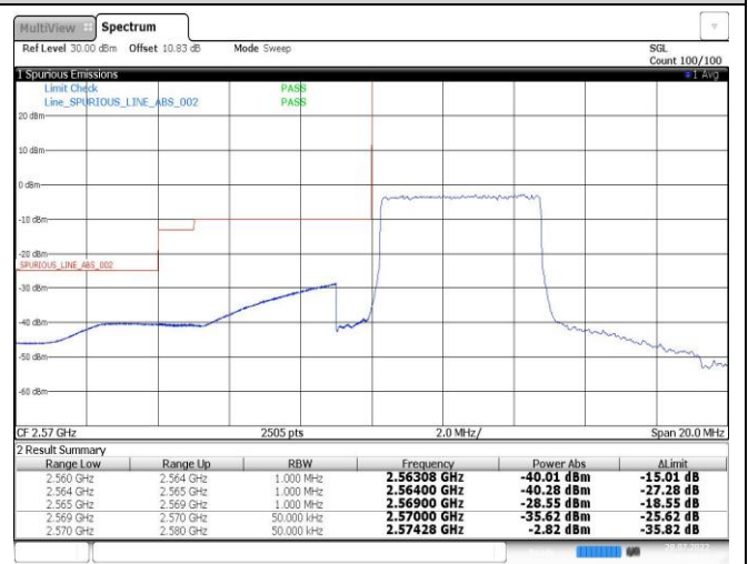
Band38-5MHz-QPSK-37775-25RB#0
