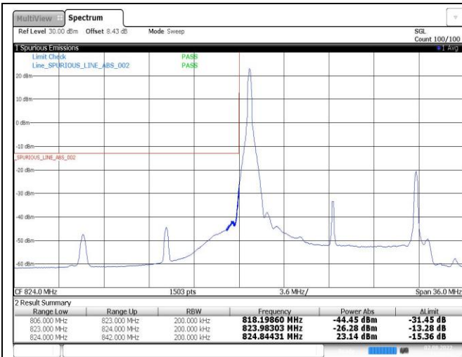
Band26-15MHz-16QAM-26865-1RB#0
