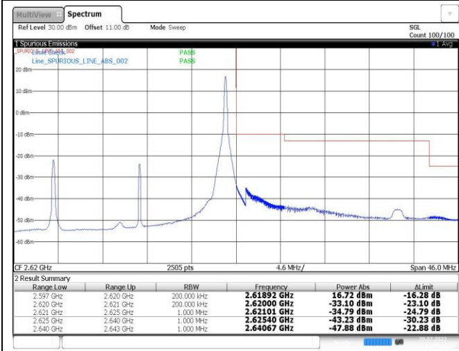
Band38-20MHz-16QAM-38150-1RB#99
