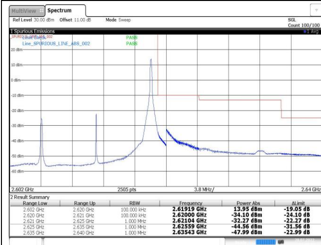
Band38-15MHz-16QAM-38175-1RB#74
