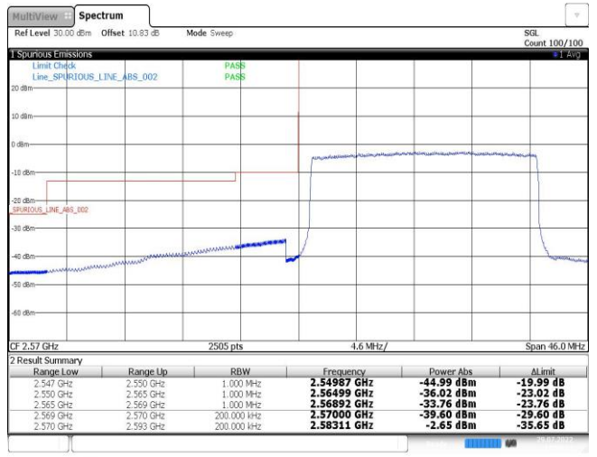
Band38-20MHz-16QAM-37850-100RB#0
