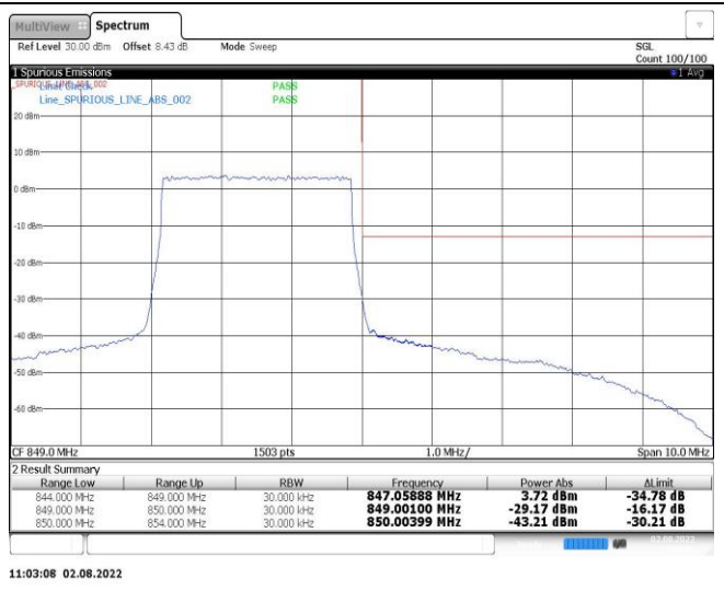
Band26-3MHz-16QAM-26705-15RB#0
