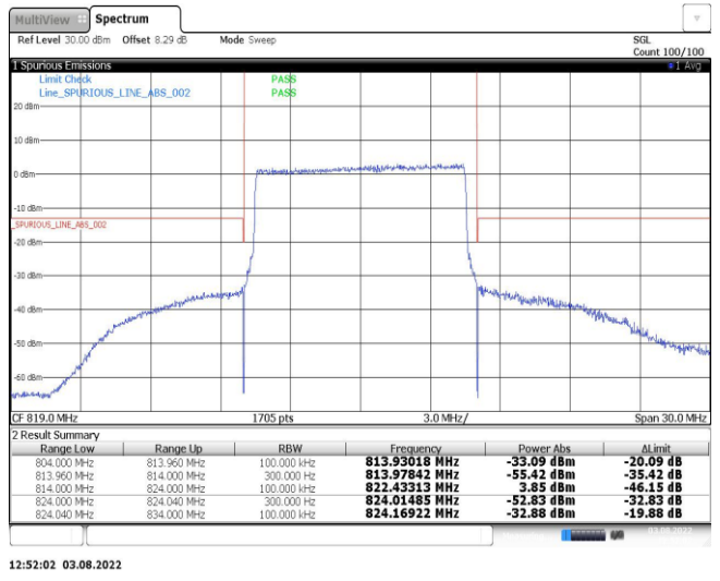
Band26-10MHz-16QAM-26840-50RB#0
