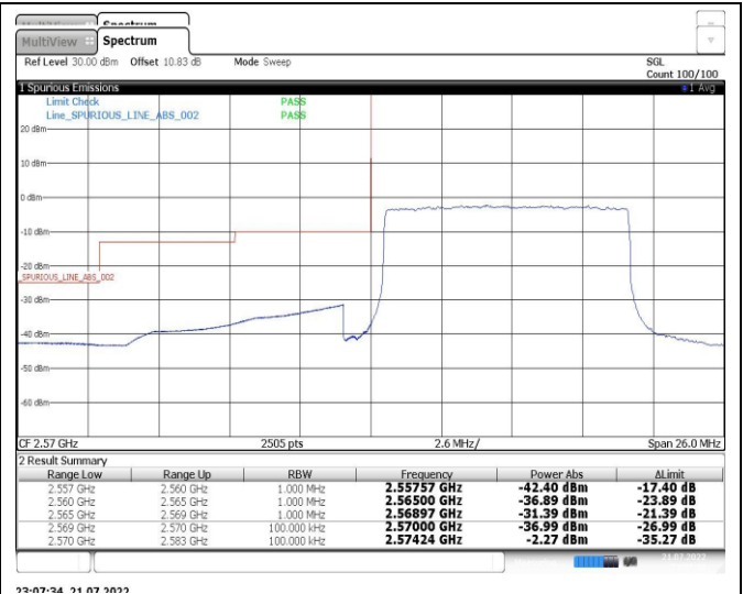
Band38-10MHz-QPSK-38200-50RB#0
