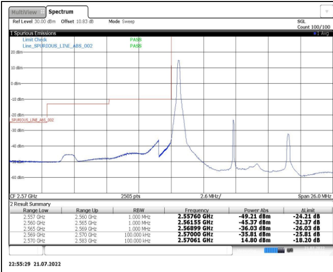
Band38-10MHz-QPSK-38200-1RB#49
