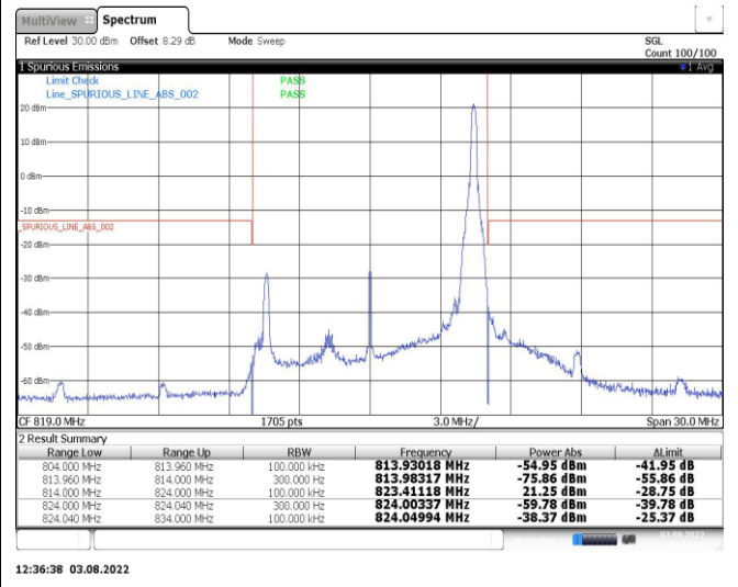
Band26-10MHz-QPSK-26840-1RB#0
