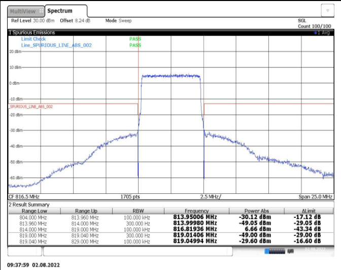
Band26-5MHz-16QAM-26815-25RB#0
