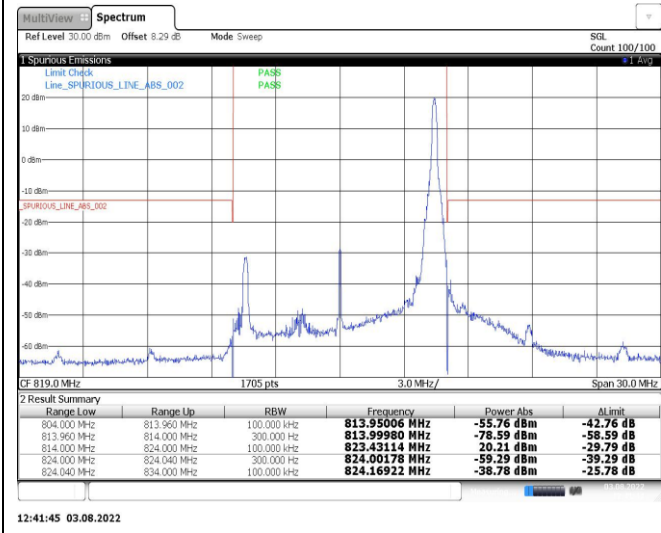
Band26-10MHz-16QAM-26840-1RB#0
