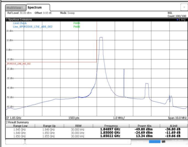
Band25-3MHz-16QAM-26055-1RB#0
