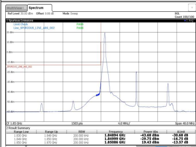
Band25-15MHz-16QAM-26115-1RB#0
