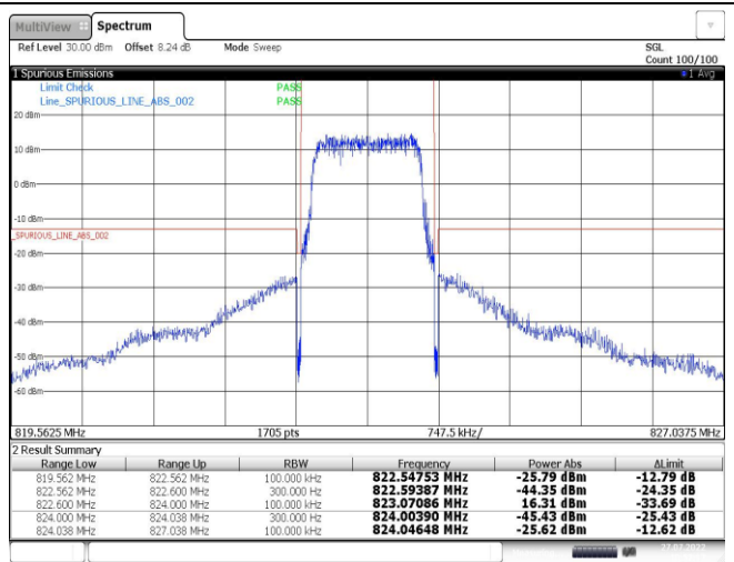
Band26-1.4MHz-QPSK-26797-6RB#0
