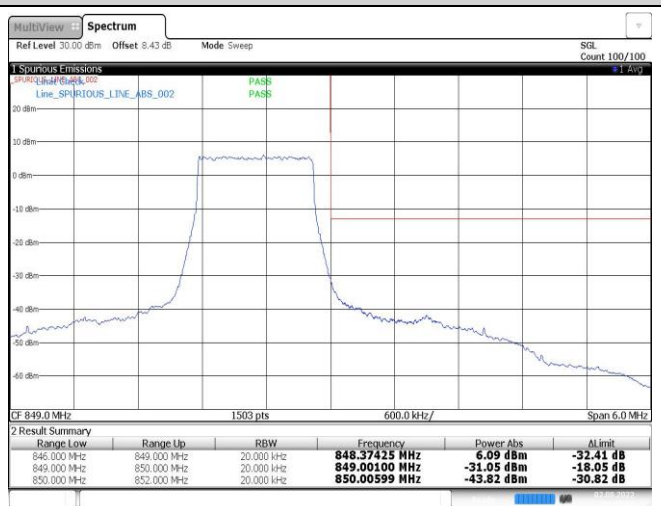
Band26-1.4MHz-QPSK-27033-6RB#0
