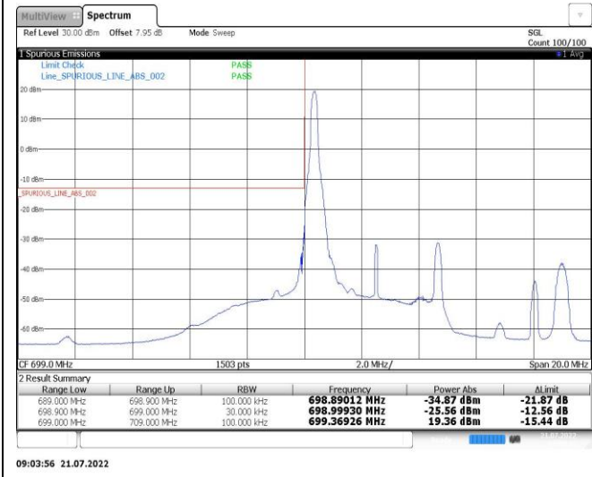
Band12-10MHz-QPSK-23060-1RB#0
