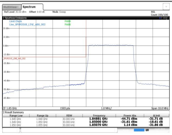
Band25-3MHz-16QAM-26055-15RB#0
