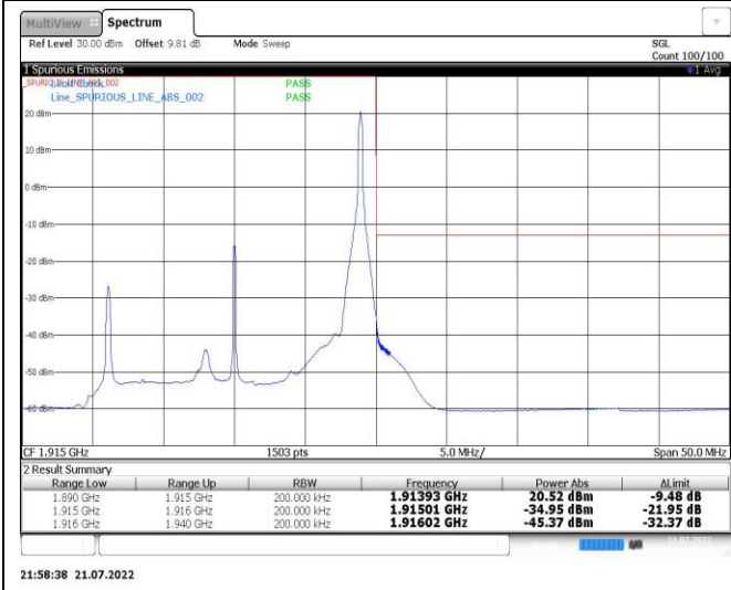
Band25-20MHz-16QAM-26140-1RB#0
