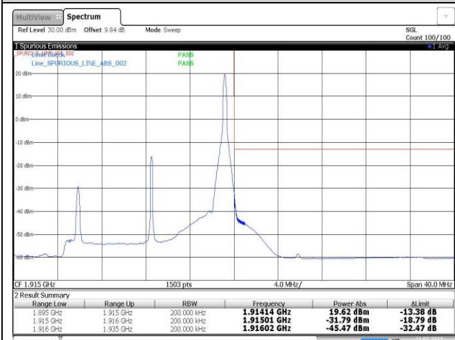
Band25-15MHz-QPSK-26615-1RB#74
