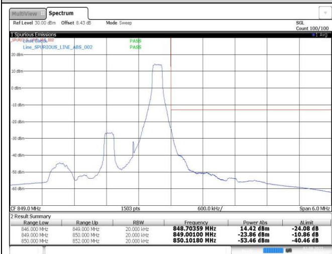
Band26-1.4MHz-QPSK-27033-1RB#5
