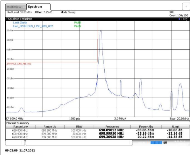
Band12-5MHz-16QAM-23035-1RB#0
