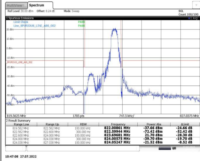
Band26-1.4MHz-16QAM-26797-1RB#0
