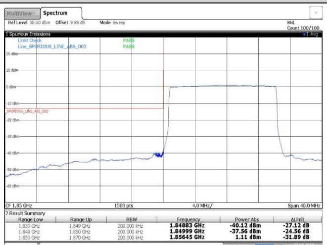
Band25-15MHz-16QAM-26115-75RB#0
