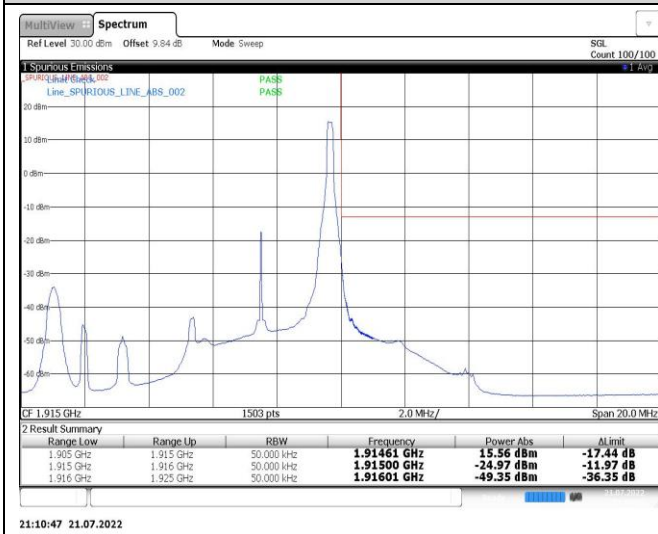
Band25-5MHz-16QAM-26065-1RB#0
