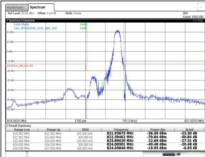
Band26-1.4MHz-QPSK-26797-1RB#0
