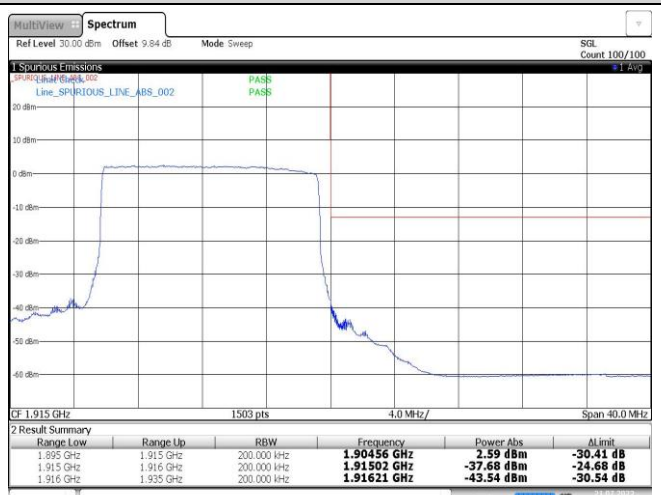
Band25-15MHz-QPSK-26615-75RB#0
