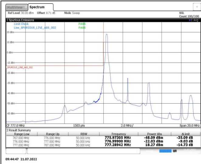
Band13-5MHz-16QAM-23205-1RB#0
