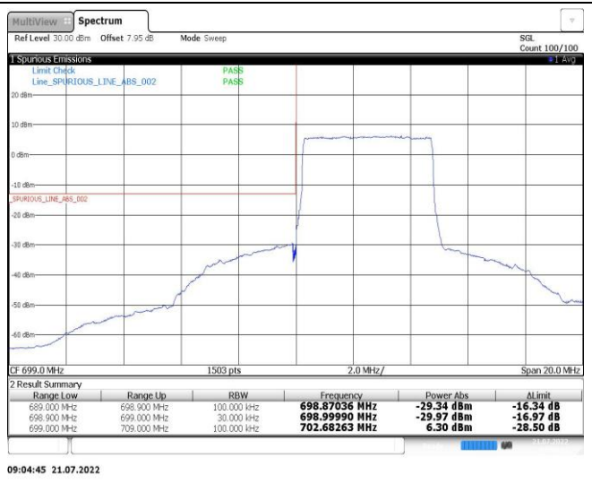
Band12-5MHz-16QAM-23035-25RB#0
