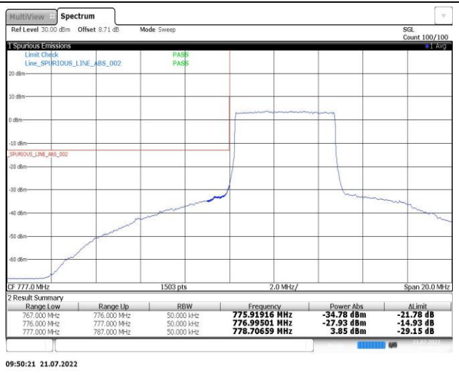
Band13-5MHz-16QAM-23205-25RB#0
