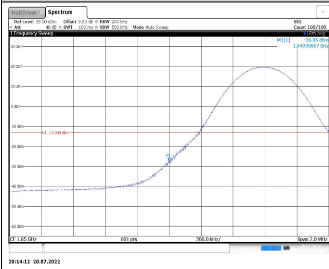
Band2-10MHz-16QAM-18650-50RB#0
