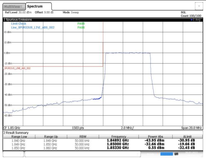
Band2-5MHz-16QAM-18625-25RB#0
