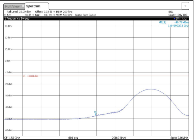
Band2-10MHz-QPSK-18650-1RB#49
