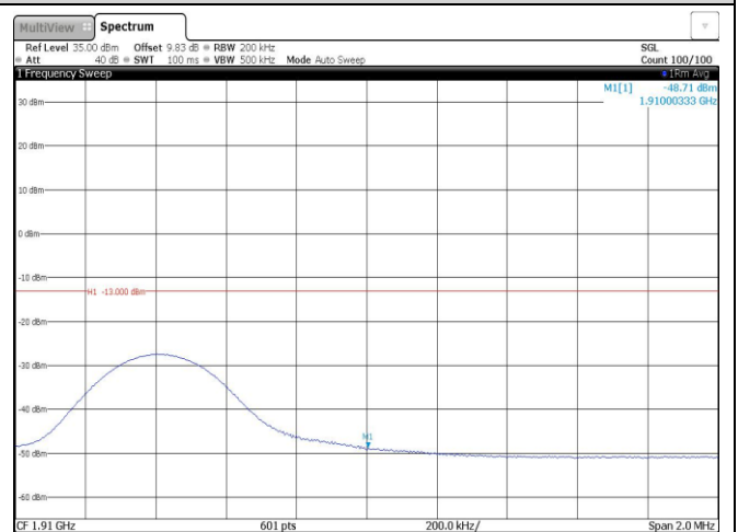
Band2-10MHz-QPSK-19150-1RB#0
