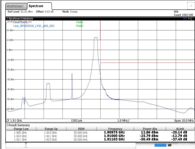
Band2-3MHz-16QAM-19185-1RB#14
