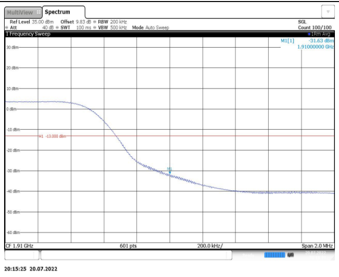
Band2-10MHz-16QAM-18650-1RB#49
