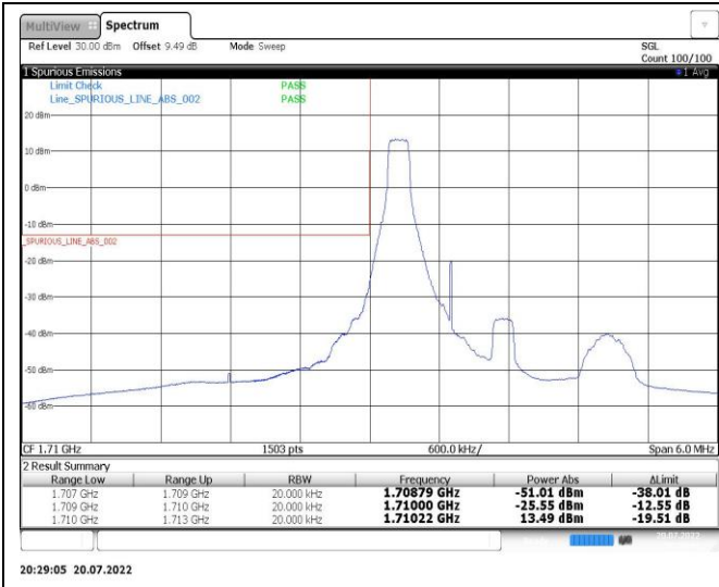
Band4-1.4MHz-QPSK-20393-1RB#5
