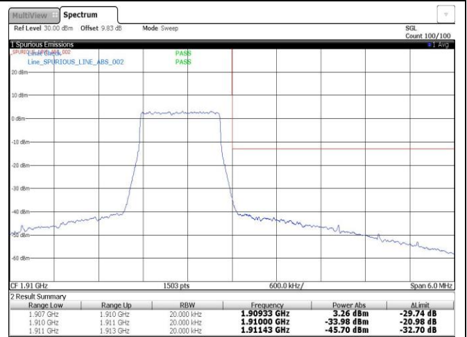
Band2-1.4MHz-16QAM-19193-6RB#0
