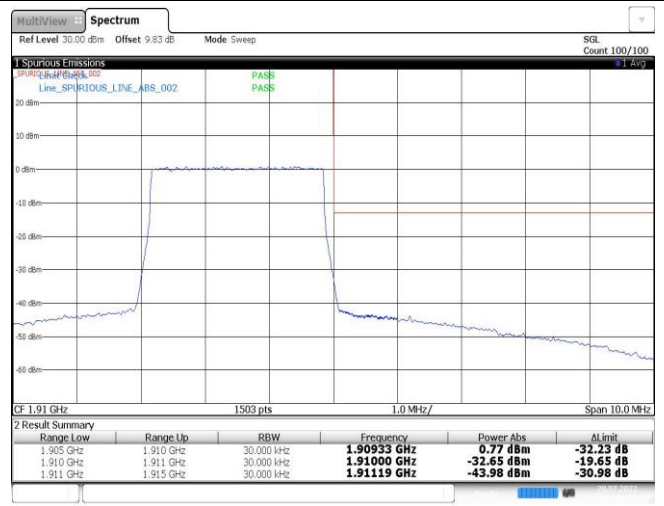
Band2-3MHz-16QAM-19185-15RB#0
