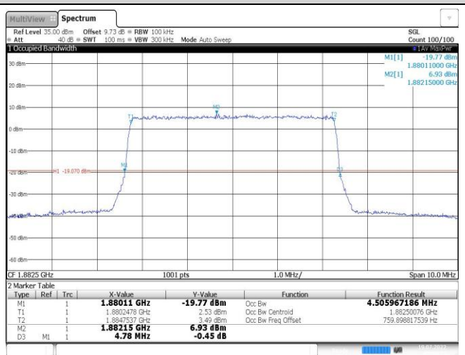
Band25-5MHz-16QAM-26365-25RB#0
