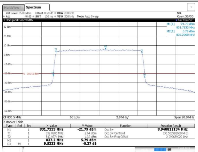
Band26-10MHz-16QAM-26915-50RB#0
