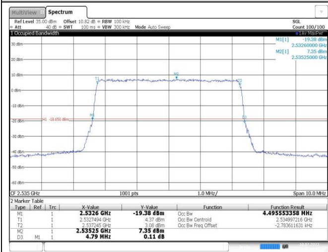
Band7-5MHz-QPSK-21100-25RB#0
