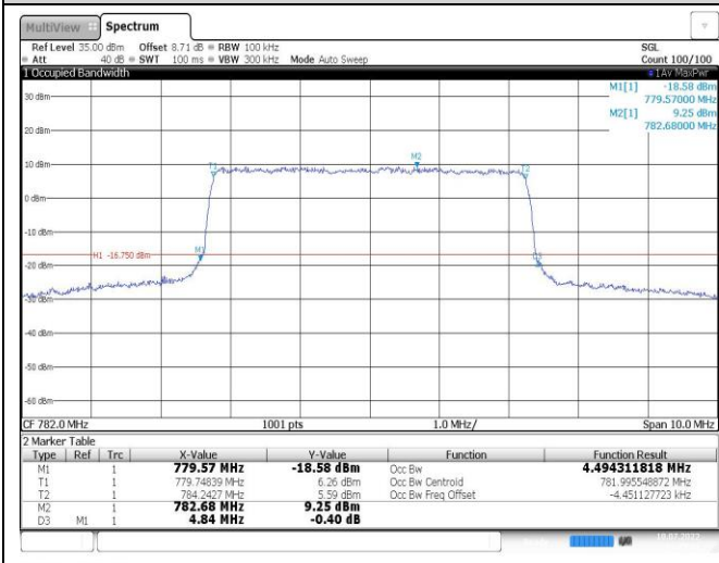
Band13-5MHz-QPSK-23230-25RB#0
