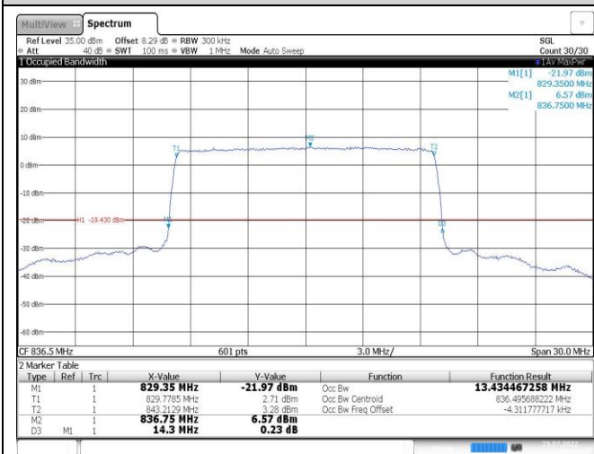
Band26-15MHz-QPSK-26915-75RB#0
