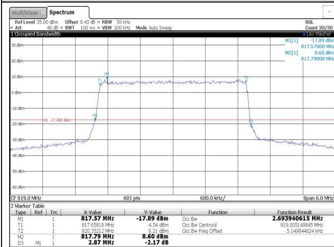
Band26-3MHz-QPSK-26740-15RB#0
