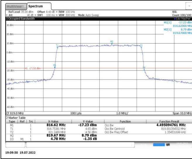
Band26-5MHz-16QAM-26740-25RB#0
