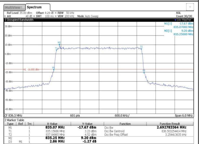
Band26-3MHz-QPSK-26915-15RB#0
