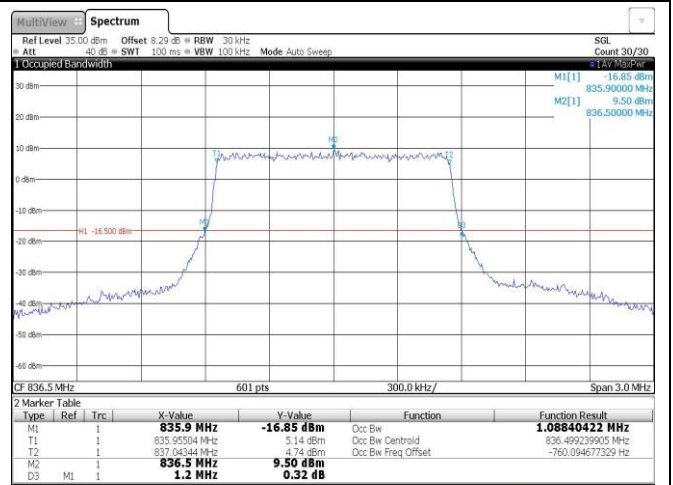
Band5-1.4MHz-16QAM-20525-6RB#0
