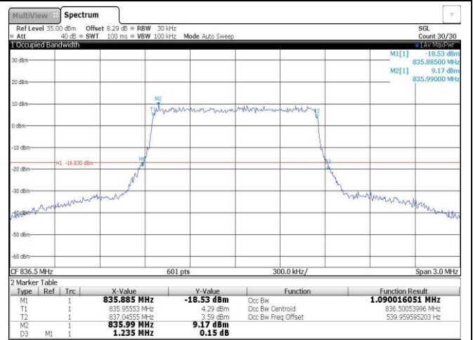
Band26-1.4MHz-16QAM-26915-6RB#0
