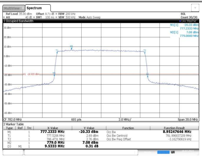
Band13-10MHz-16QAM-23230-50RB#0
