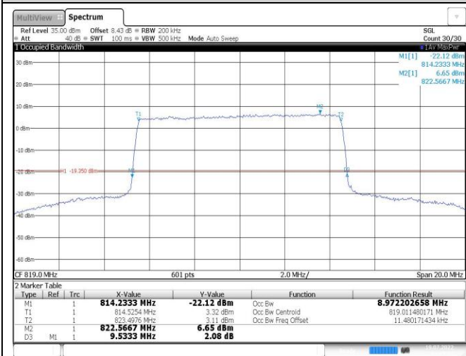
Band26-10MHz-16QAM-26740-50RB#0
