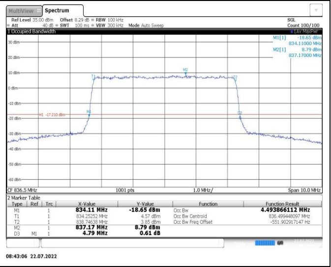
Band26-5MHz-16QAM-26915-25RB#0
