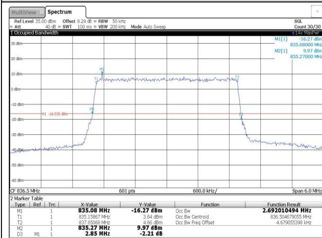
Band5-3MHz-QPSK-20525-15RB#0
