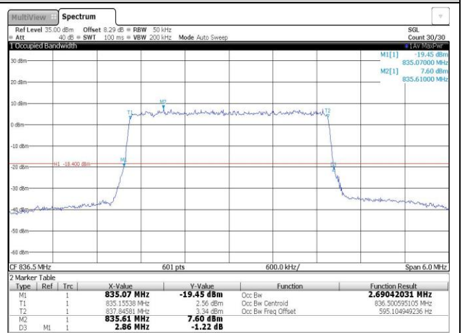
Band5-3MHz-16QAM-20525-15RB#0
