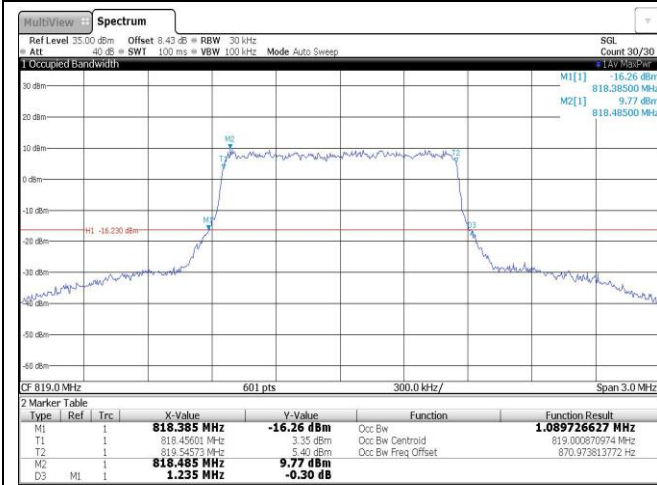
Band26-1.4MHz-16QAM-26740-6RB#0
