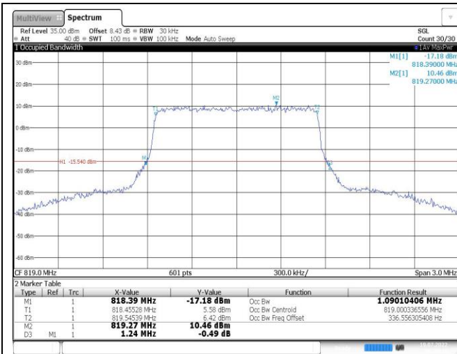
Band26-1.4MHz-16QAM-26740-6RB#0
