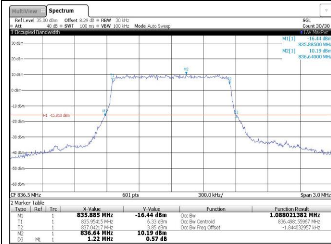
Band5-1.4MHz-QPSK-20525-6RB#0
