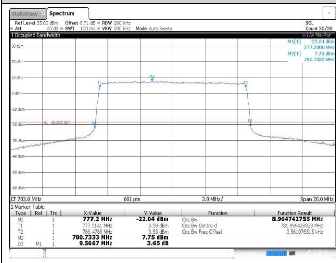
Band13-10MHz-QPSK-23230-50RB#0
