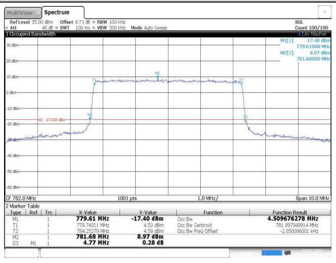
Band13-5MHz-16QAM-23230-25RB#0
