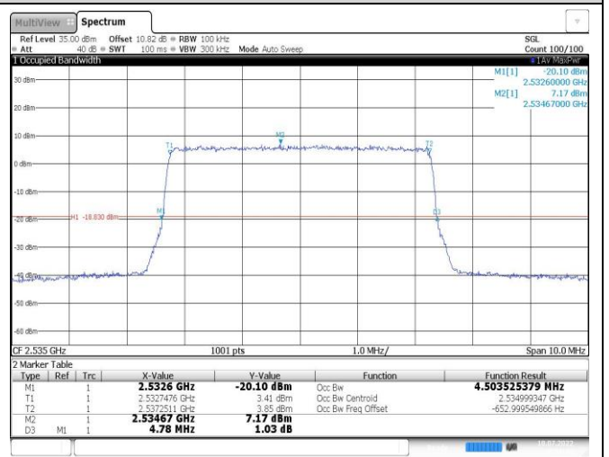
Band7-5MHz-16QAM-21100-25RB#0
