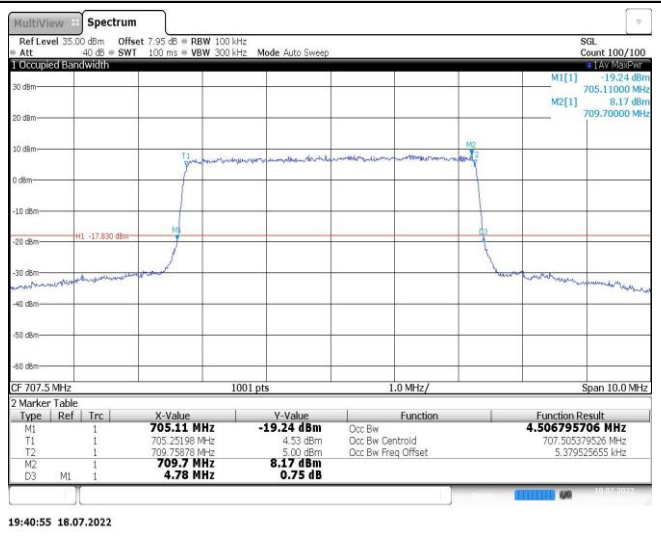
Band12-10MHz-16QAM-23095-50RB#0
