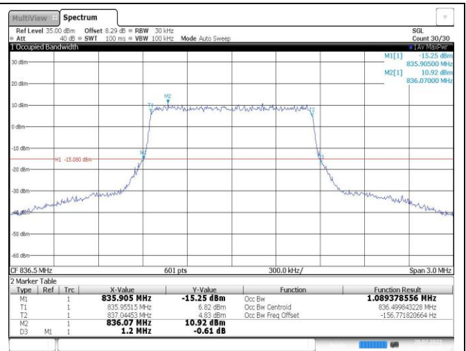
Band26-1.4MHz-16QAM-26915-6RB#0
