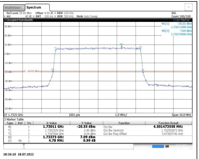
Band4-10MHz-16QAM-20175-50RB#0
