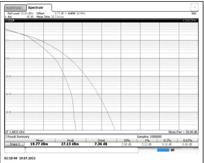
Band25-15MHz-16QAM-26365-75RB#0
