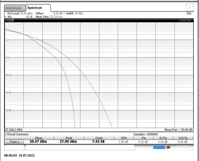
Band26-10MHz-QPSK-26915-50RB#0
