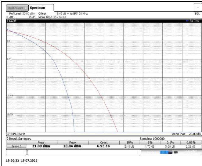
Band26-10MHz-16QAM-26740-50RB#0
