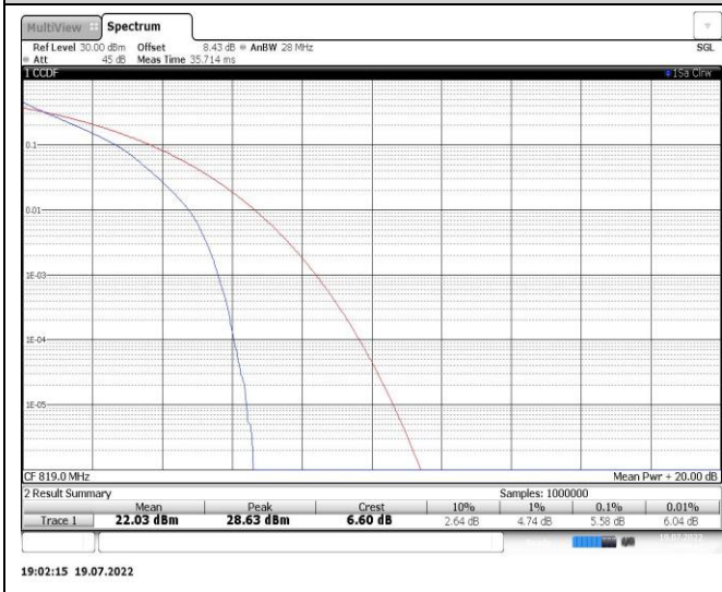
Band26-3MHz-16QAM-26740-15RB#0
