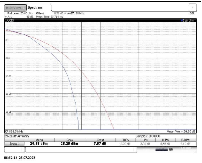
Band26-5MHz-QPSK-26915-25RB#0
