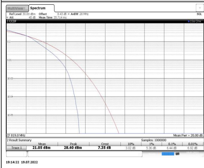
Band26-10MHz-QPSK-26740-50RB#0
