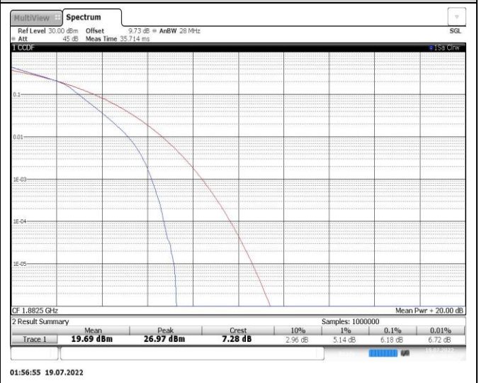
Band25-5MHz-16QAM-26365-25RB#0
