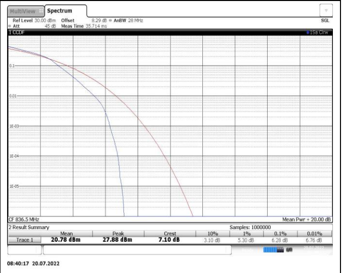
Band26-3MHz-QPSK-26915-15RB#0
