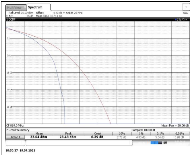
Band26-1.4MHz-16QAM-26740-6RB#0
