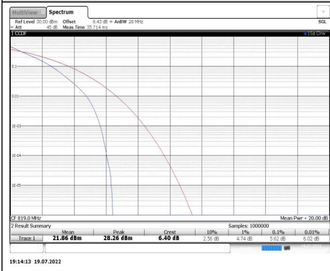
Band26-5MHz-16QAM-26740-25RB#0
