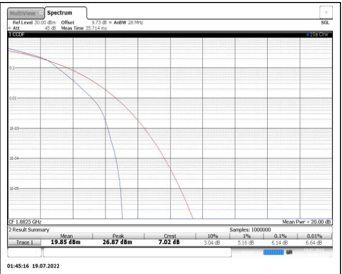
Band25-3MHz-16QAM-26365-15RB#0
