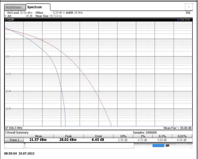
Band26-5MHz-16QAM-26915-25RB#0
