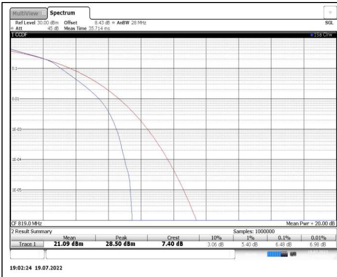
Band26-5MHz-QPSK-26740-25RB#0
