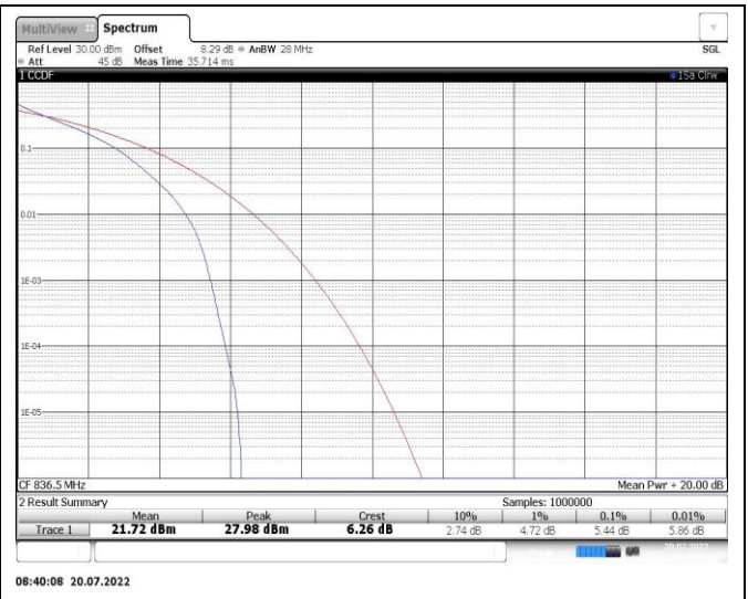
Band26-1.4MHz-16QAM-26915-6RB#0
