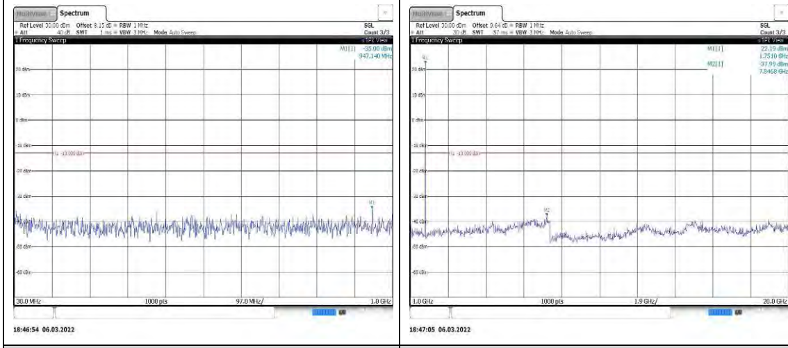
Band4-1.4MHz-QPSK-20393-1RB#0-Range1 :30~1000MHz Band4-1.4MHz-QPSK-20393-1RB#0-Range2 :1000~20000MHz
