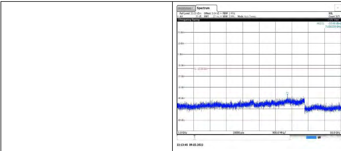
Band12-1.4MHz-QPSK-23017-1RB#0-Range 2:1000~10000MHz
