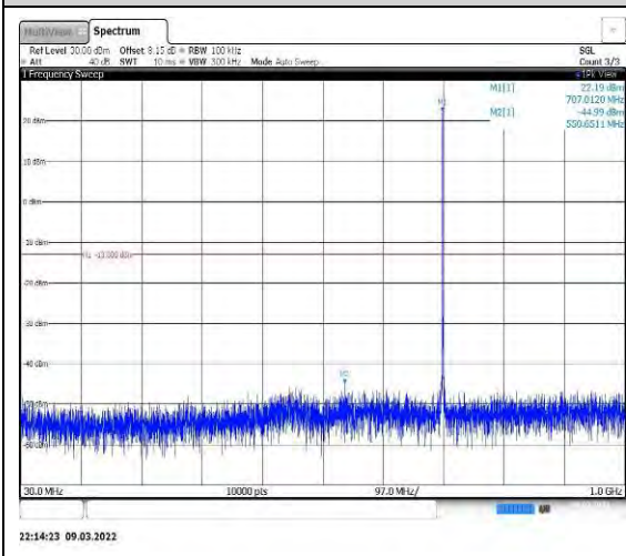
Band12-1.4MHz-QPSK-23095-1RB#0-Range 1:30~1000MHz
