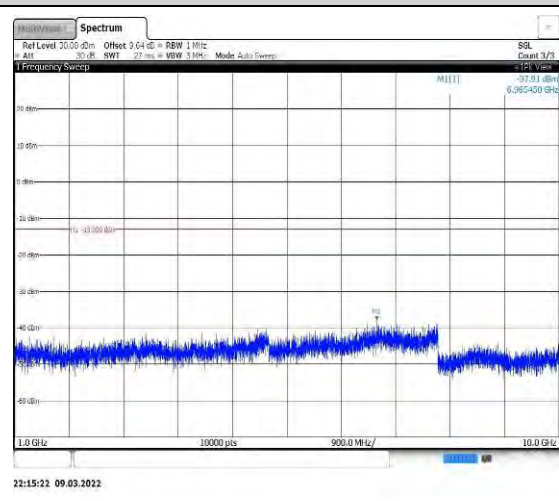
Band12-1.4MHz-QPSK-23173-1RB#0-Range 2:1000~10000MHz
