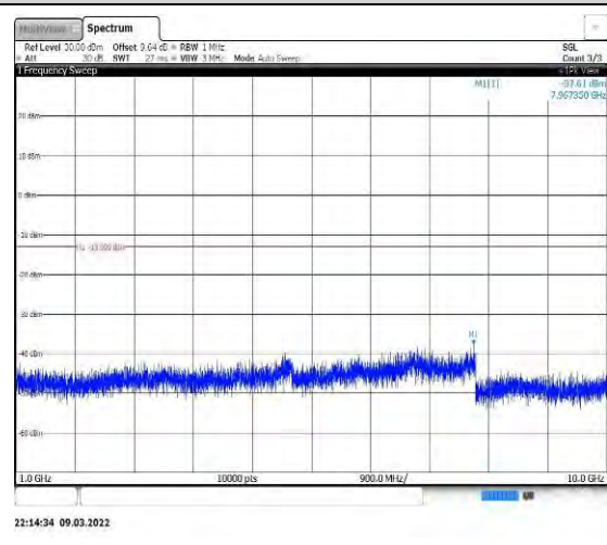
Band12-1.4MHz-QPSK-23095-1RB#0-Range 2:1000~10000MHz
