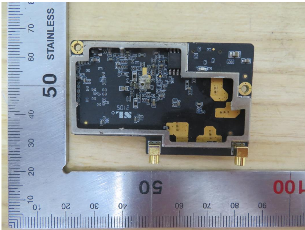
Internal View of EUT-15 (WIFI Module)
