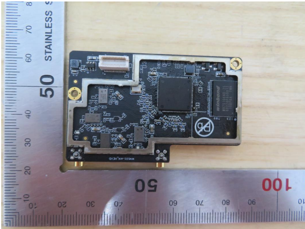
Internal View of EUT-18 (Terrain Radar)
