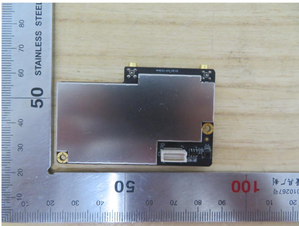
Internal View of EUT-16 (WIFI Module)
