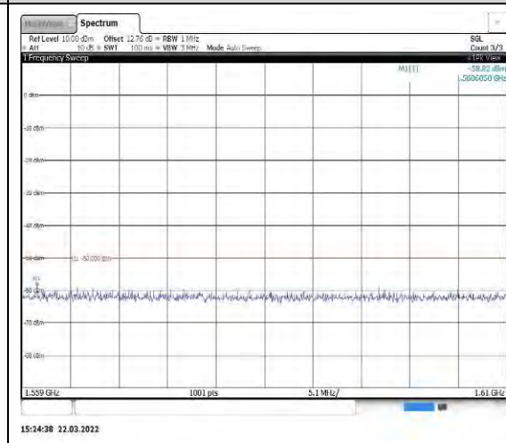
Band13-10MHz-16QAM-23230-1RB#0-Rang e3:1559~1610MHz
