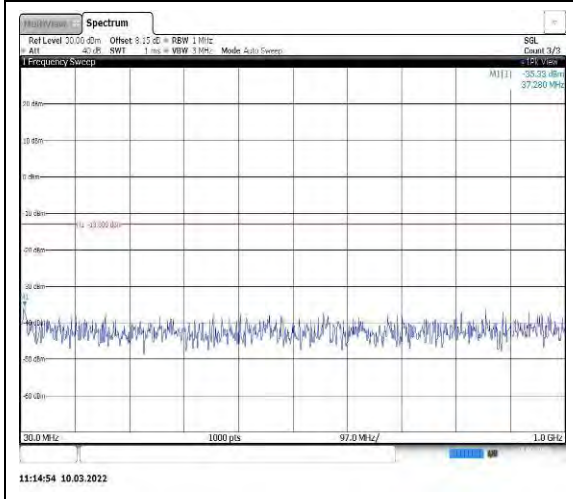
Band25-15MHz-16QAM-26115-1RB#0-Rang e1:30~1000MHz
