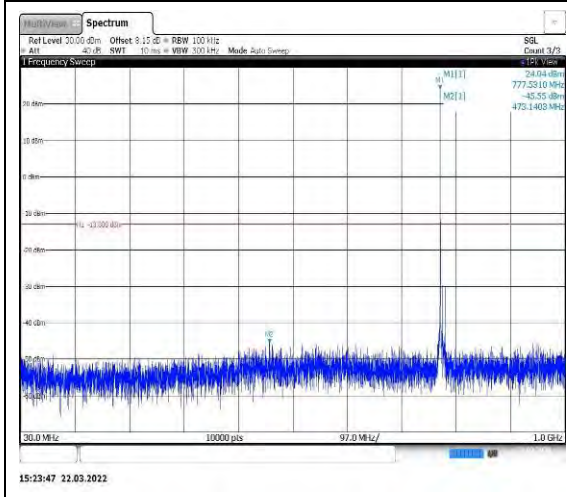
Band13-10MHz-QPSK-23230-1RB#0-Range 1:30~1000MHz
