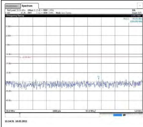
Band25-15MHz-QPSK-26115-1RB#0-Range 1:30~1000MHz
