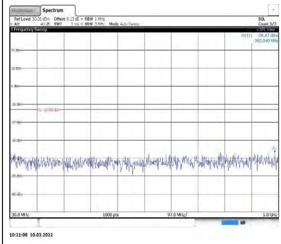
Band25-3MHz-QPSK-26055-1RB#0-Range1: 30~1000MHz
