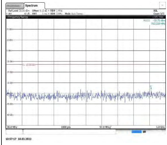
Band25-10MHz-QPSK-26090-1RB#0-Range 1:30~1000MHz
