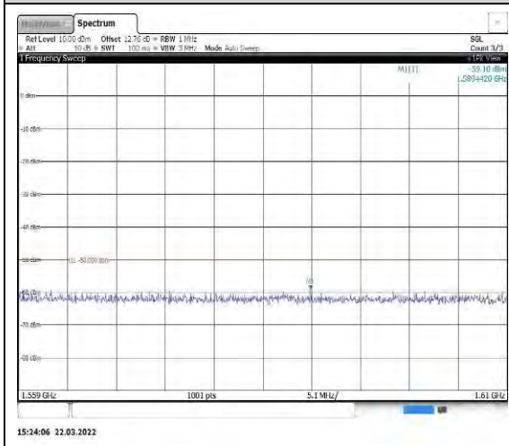
Band13-10MHz-QPSK-23230-1RB#0-Range 3:1559~1610MHz
