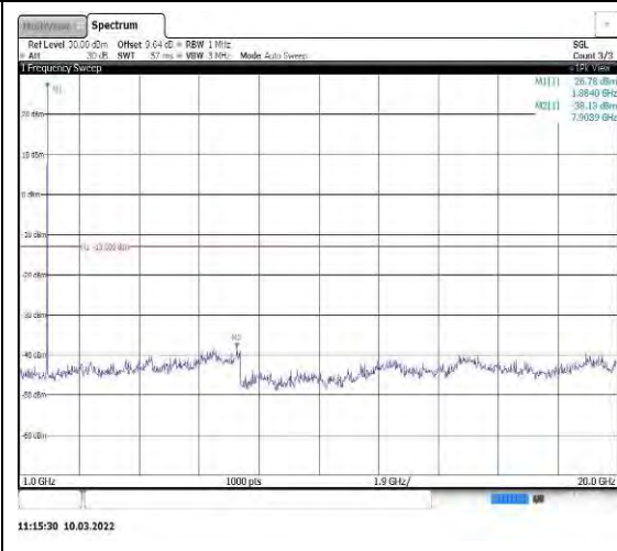
Band25-15MHz-QPSK-26365-1RB#0-Range 2:1000~20000MHz
