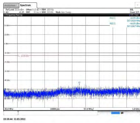
Band13-5MHz-16QAM-23205-1RB#0-Range 1:30~1000MHz
