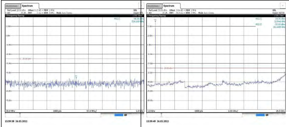
Band38-15MHz-QPSK-38175-1RB#0-Rang e1:30~1000MHz
