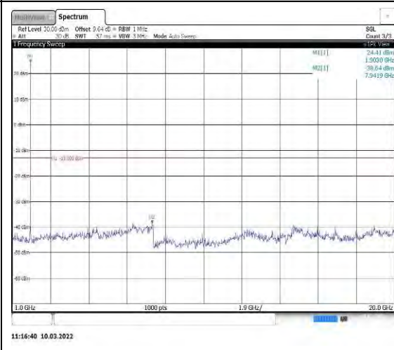
Band25-15MHz-16QAM-26615-1RB#0-Rang e2:1000~20000MHz
