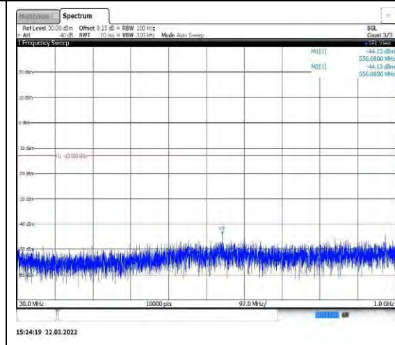
Band13-10MHz-16QAM-23230-1RB#0-Rang e1:30~1000MHz
