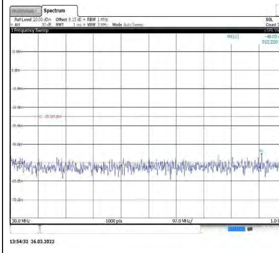
Band38-5MHz-16QAM-38225-1RB#0-Rang e1:30~1000MHz
