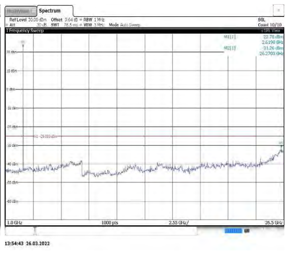
Band38-5MHz-16QAM-38225-1RB#0-Range2: 1000~26500MHz
