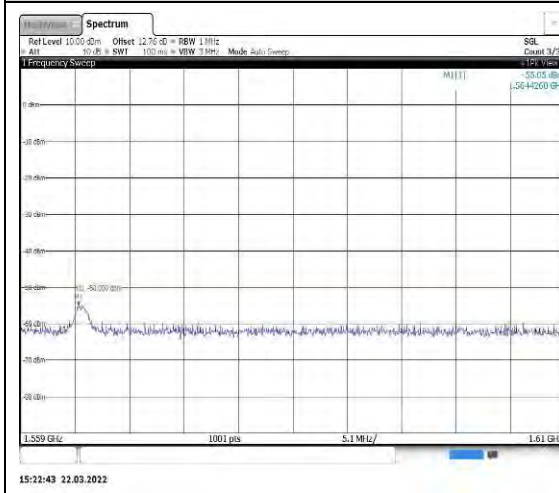
Band13-5MHz-QPSK-23255-1RB#0-Range3: 1559~1610MHz
