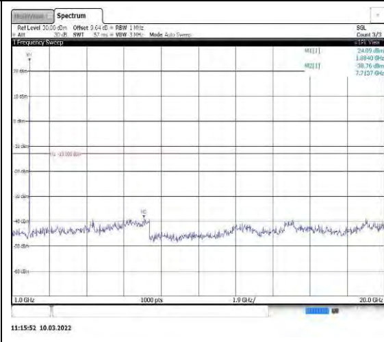
Band25-15MHz-16QAM-26365-1RB#0-Rang e2:1000~20000MHz
