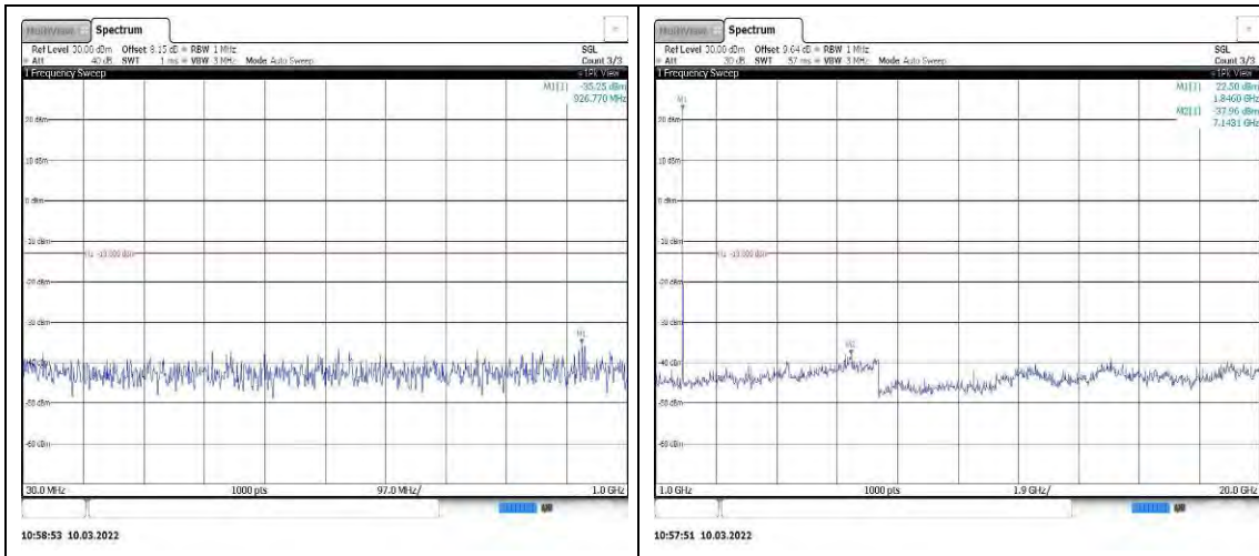
Band25-10MHz-QPSK-26640-1RB#0-Range 1:30~1000MHz Band25-10MHz-16QAM-26090-1RB#0-Rang e2:1000~20000MHz
