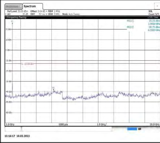
Band25-15MHz-QPSK-26615-1RB#0-Range 2:1000~20000MHz
