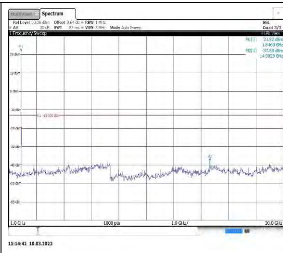
Band25-15MHz-QPSK-26115-1RB#0-Range 2:1000~20000MHz
