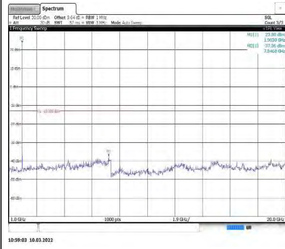
Band25-10MHz-QPSK-26640-1RB#0-Range 2:1000~20000MHz
