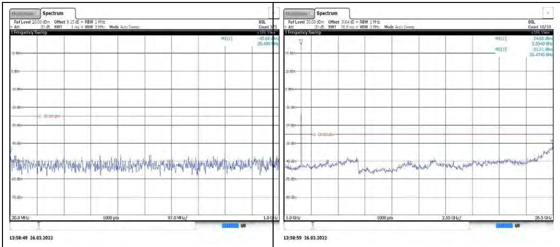
Band38-15MHz-QPSK-38000-1RB#0-Rang e1:30~1000MHz
