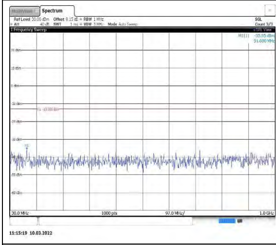
Band25-15MHz-QPSK-26365-1RB#0-Range 1:30~1000MHz
