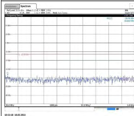
Band25-3MHz-16QAM-26365-1RB#0-Range 1:30~1000MHz
