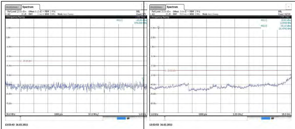
Band38-5MHz-16QAM-38000-1RB#0-Rang e1:30~1000MHz
