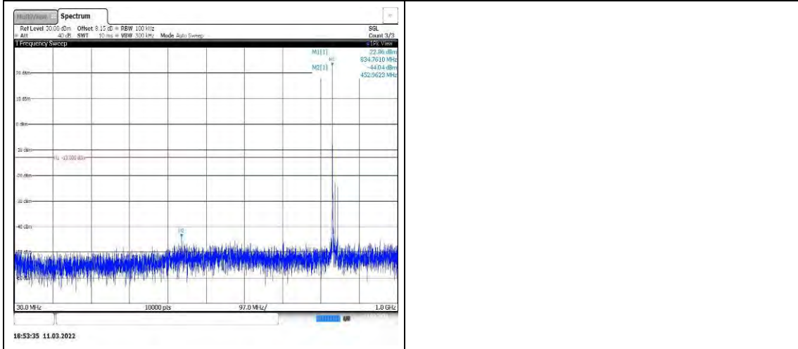
Band26-15MHz-16QAM-26965-1RB#0-Rang e1:30~1000MHz
