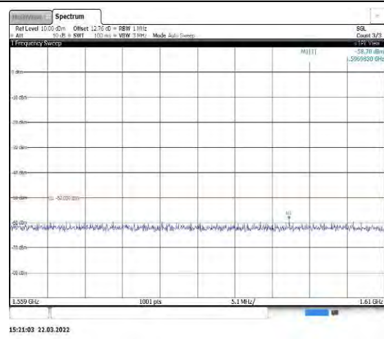
Band13-5MHz-16QAM-23205-1RB#0-Range 3:1559~1610MHz
