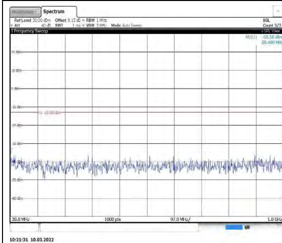
Band25-3MHz-16QAM-26055-1RB#0-Range 1:30~1000MHz
