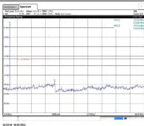
Band25-3MHz-16QAM-26675-1RB#0-Range 2:1000~20000MHz
