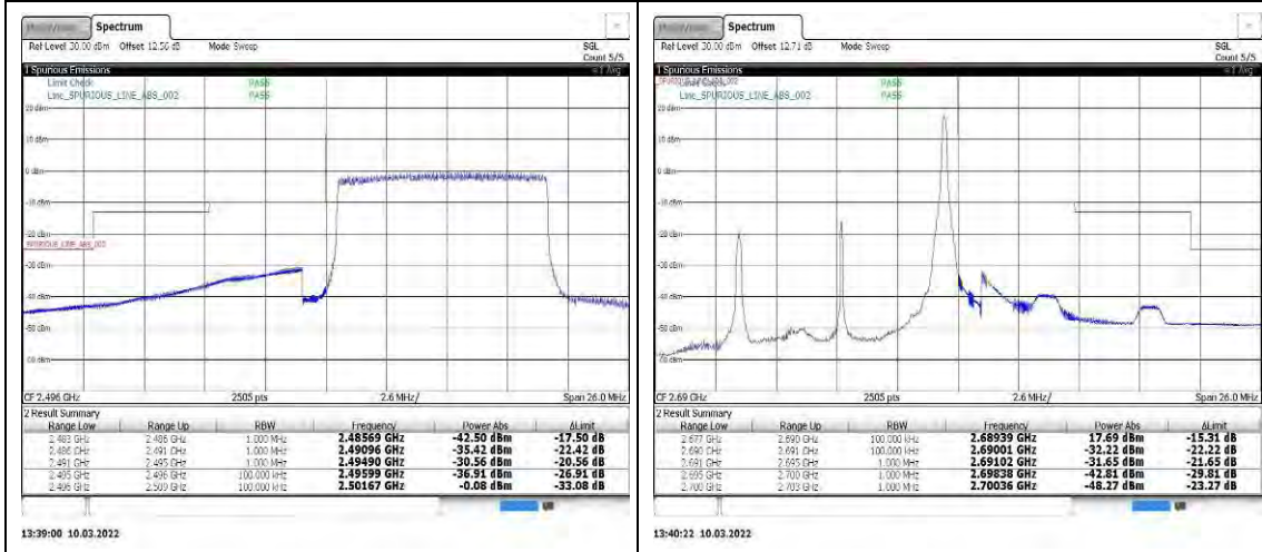
Band41-10MHz-16QAM-39700-50RB#0
