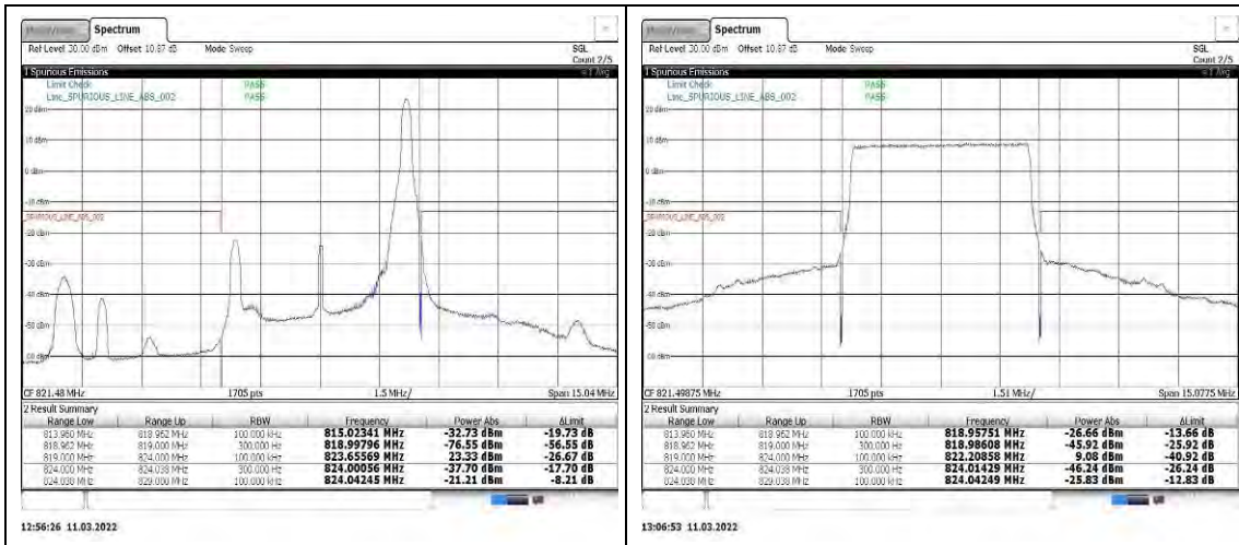
Band26-5MHz-QPSK-26765-1RB#24
