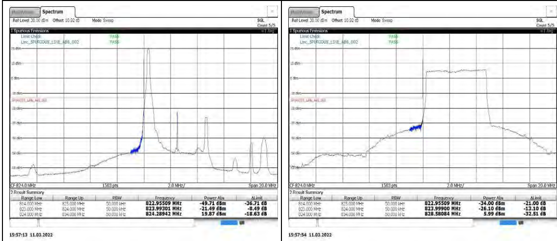
Band26-5MHz-QPSK-26815-1RB#0
