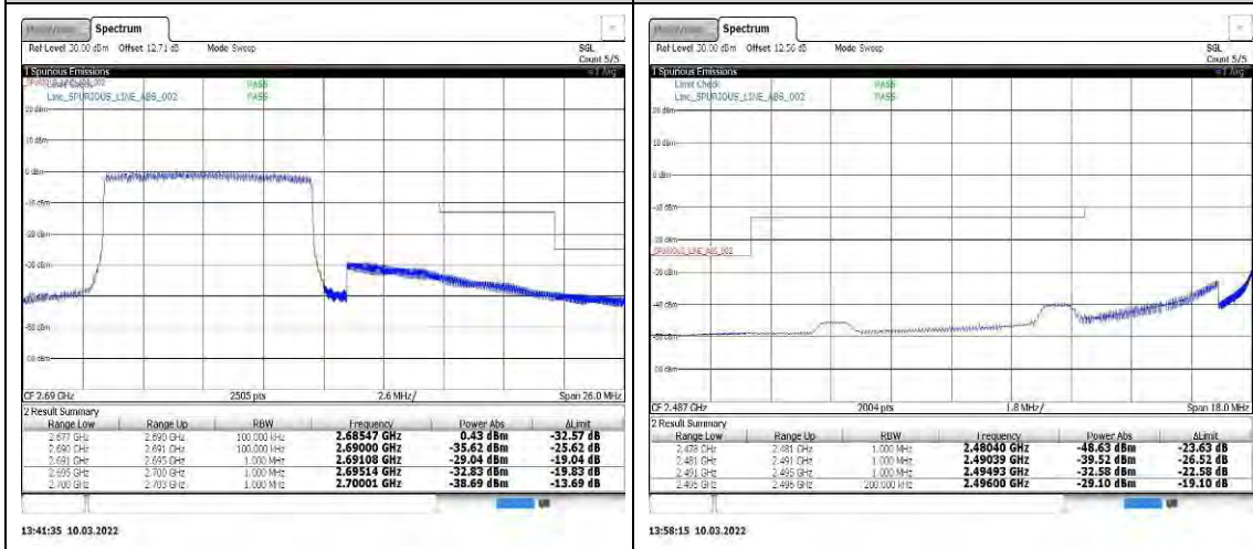
Band41-10MHz-16QAM-41540-50RB#0
