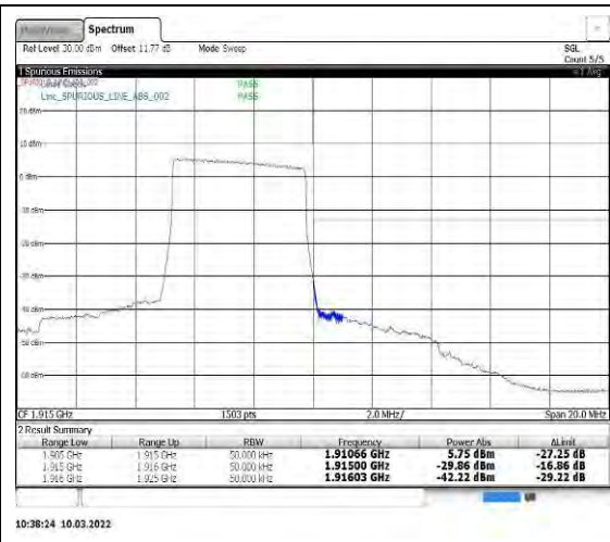
Band25-5MHz-QPSK-26665-25RB#0
