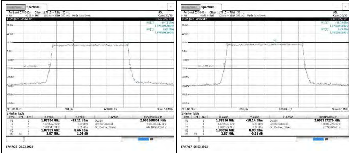
Band2-3MHz-16QAM-18900-15RB#0
