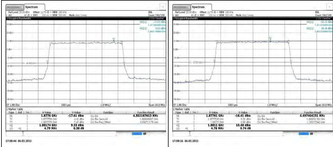
Band2-5MHz-16QAM-18900-25RB#0
