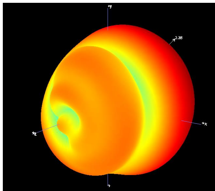
B1.3 3D Pattern for 2500MHz
