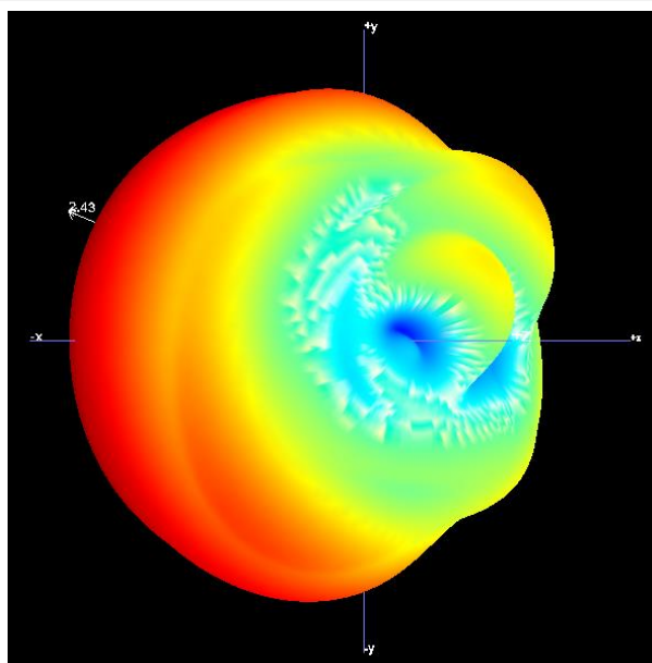
B1.2 3D Pattern for 2450MHz
