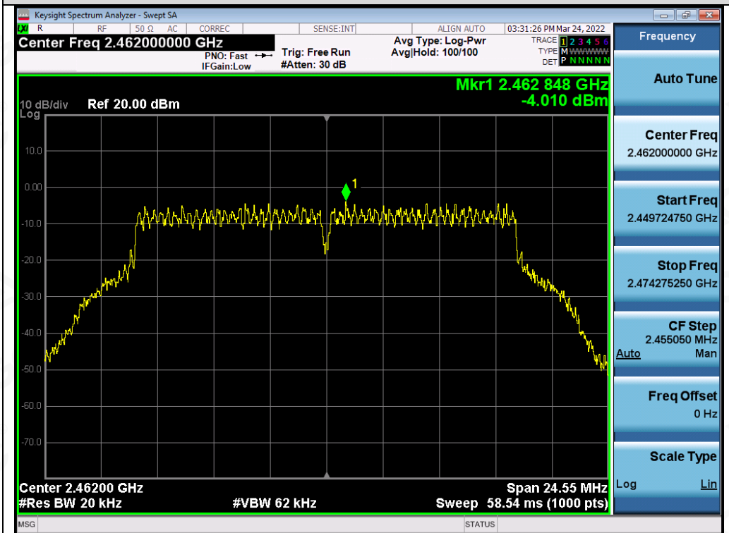
Test_Graph_802.11g_ANT1_2462_6Mbps_PSD
