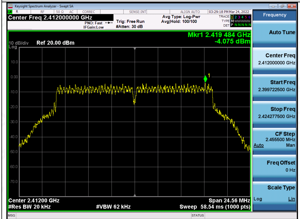
Test_Graph_802.11g_ANT1_2412_6Mbps_PSD
