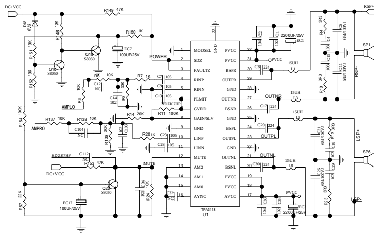
Amplifier Section
