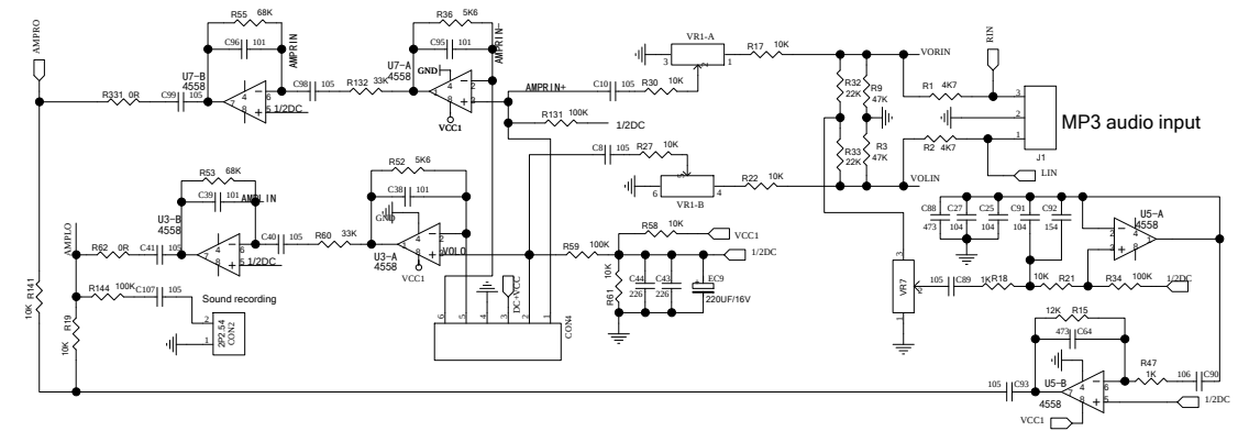
Audio amplifier
