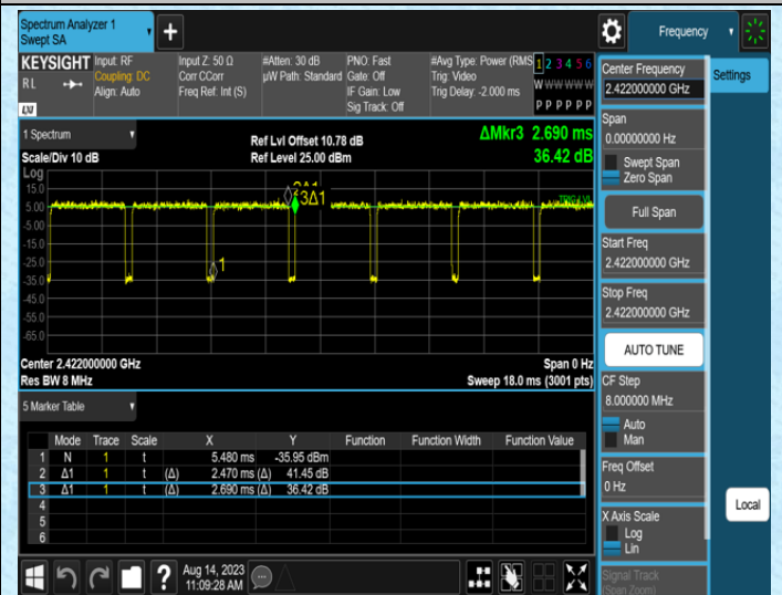
NTNV-11N40SISO-Ant1-2422
