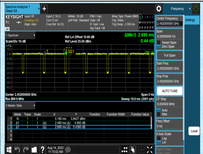
NTNV-11N40SISO-Ant1-2452
