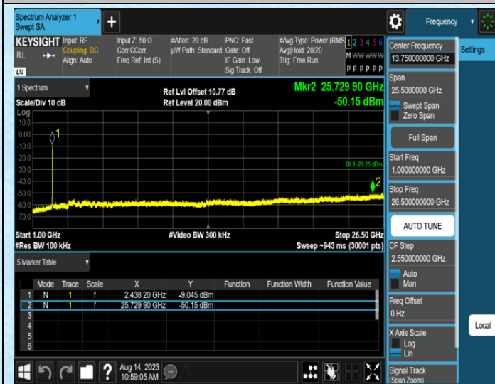
11N20SISO-Ant1-2437-1000~26500
