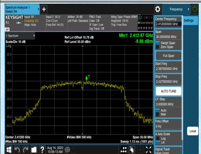
11N20SISO-Ant1-2412-0-Reference
