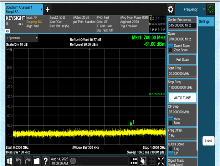
11N20SISO-Ant1-2437-30~1000
