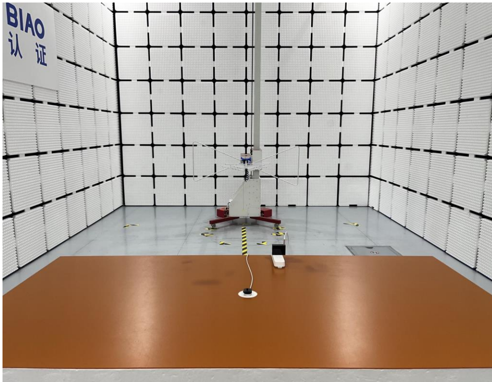
Radiated Emission Above 30MHz
