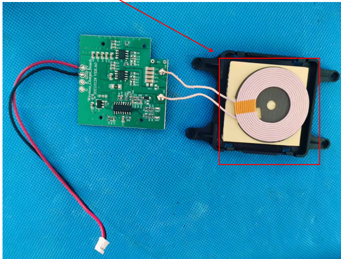
Coil Antenna
