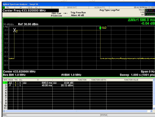
T on1
