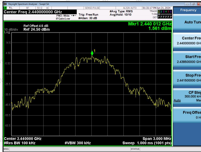
BLE_1M-Ant1-2440-0~Reference-PASS
