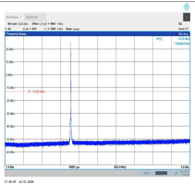
Band66_3MHz_QPSK_131987_1RB#0_1000~3000_1000~3000 3000
