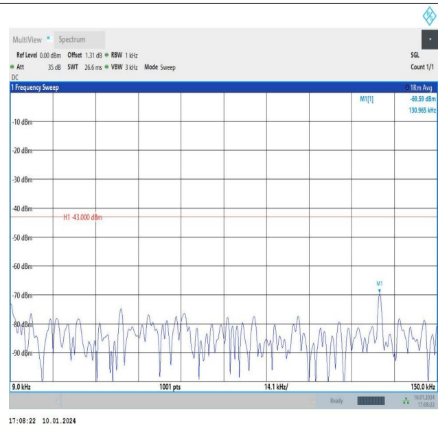
Band66_3MHz_16QAM_132322_1RB#0_0.009~0.15_0.00 9~0.15
