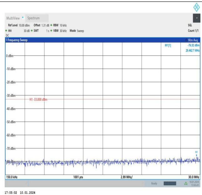
Band66_1.4MHz_QPSK_132665_1RB#0_0.15~30_0.15~30
