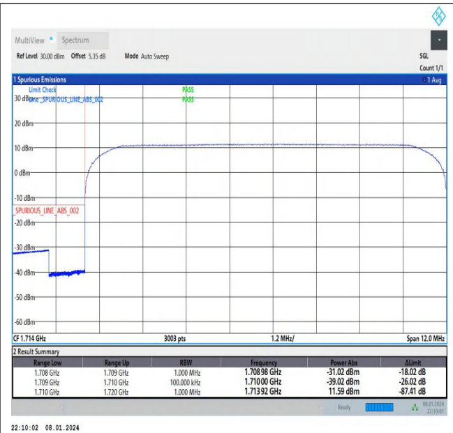
Band66_10MHz_16QAM_132022_50RB#0
