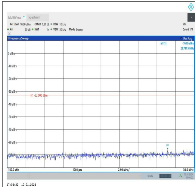
Band66_1.4MHz_16QAM_132322_1RB#0_0.15~30_0.15 ~30
