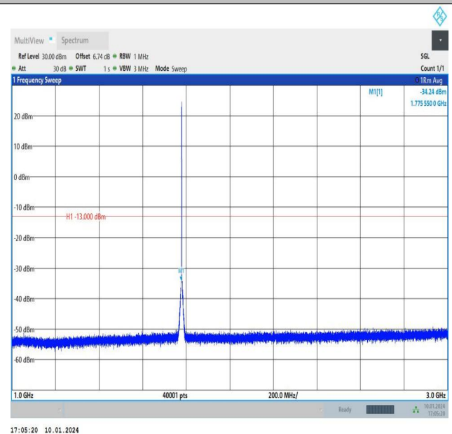
Band66_1.4MHz_QPSK_132665_1RB#0_1000~3000_1000~3000
