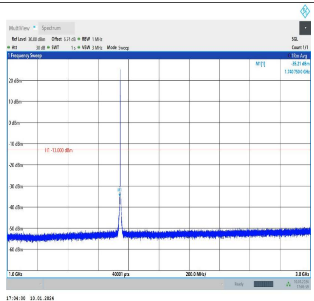
Band66_1.4MHz_QPSK_132322_1RB#0_1000~3000_1000~3000
