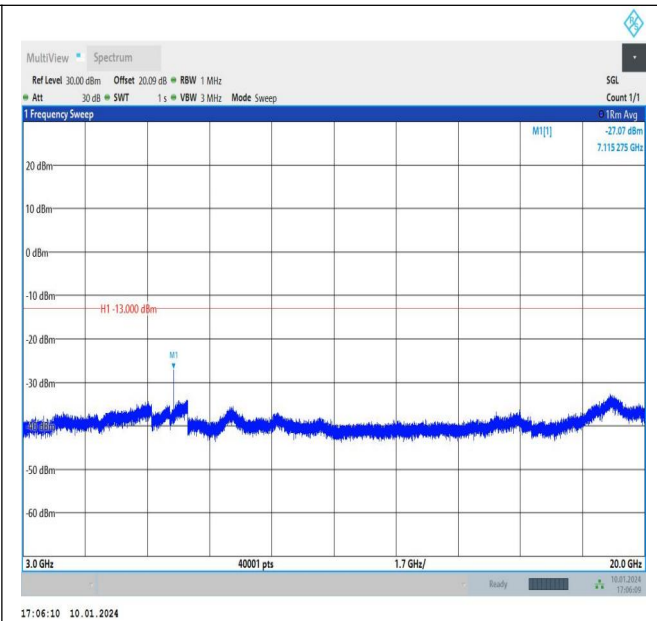
Band66_1.4MHz_16QAM_132665_1RB#0_3000~20000_3000~20000
