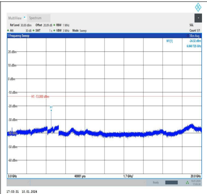
Band66_1.4MHz_16QAM_131979_1RB#0_3000~20000_3000~20000
