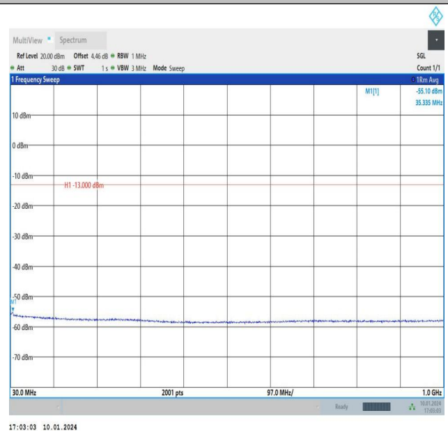
Band66_1.4MHz_16QAM_131979_1RB#0_30~1000_30~1 000
