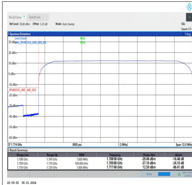
Band66_10MHz_QPSK_132022_50RB#0
