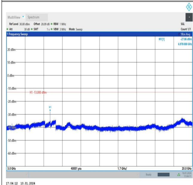
Band66_1.4MHz_QPSK_132322_1RB#0_3000~20000_3000~20000
