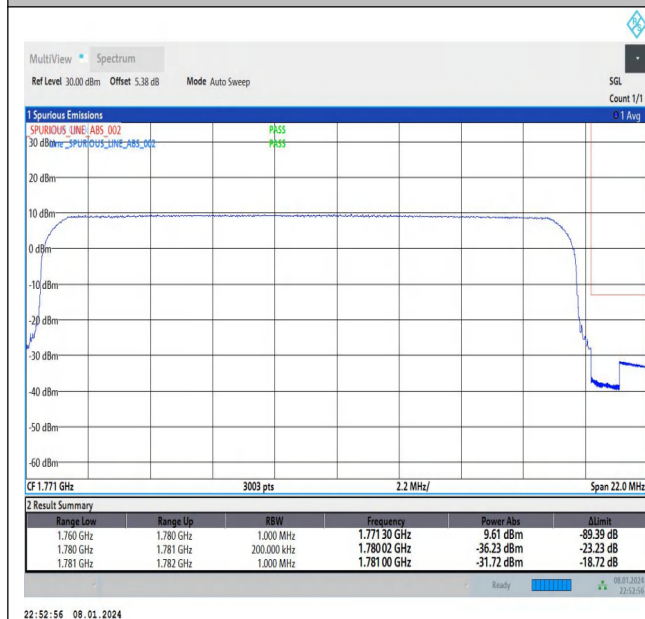
Band66_20MHz_QPSK_132572_100RB#0
