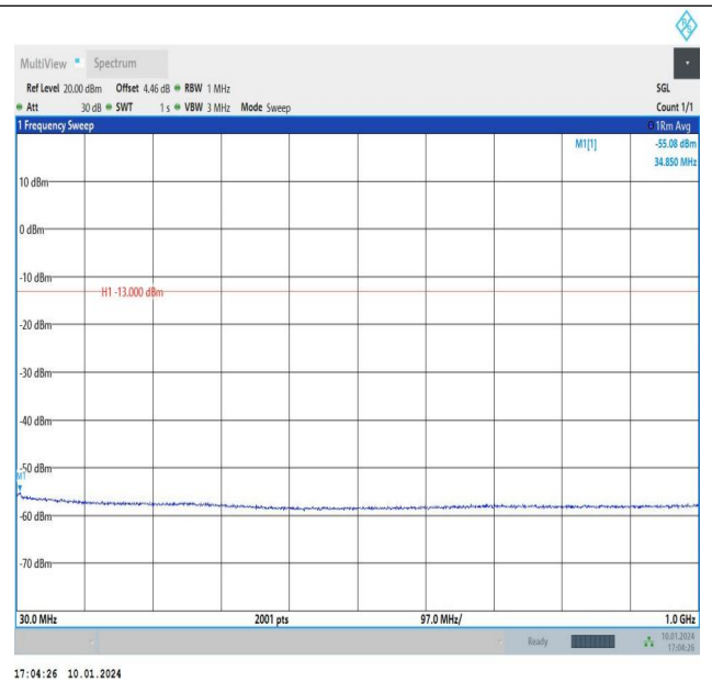
Band66_1.4MHz_16QAM_132322_1RB#0_30~1000_30~1 000
