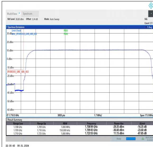
Band66_15MHz_QPSK_132047_75RB#0
