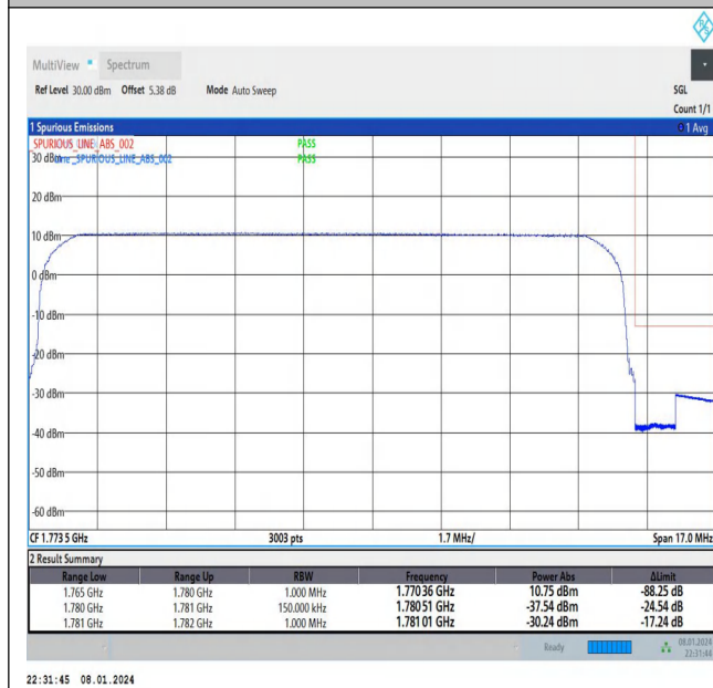
Band66_15MHz_QPSK_132597_75RB#0
