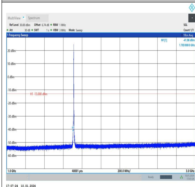
Band66_3MHz_16QAM_131987_1RB#0_1000~3000_100 0~3000
