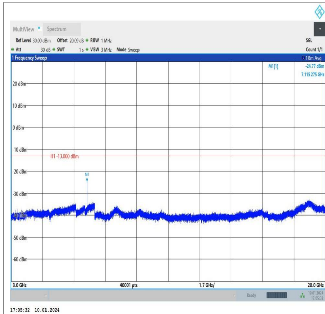
Band66_1.4MHz_QPSK_132665_1RB#0_3000~20000_3000~20000
