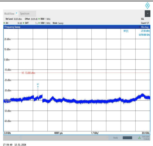
Band66_1.4MHz_16QAM_132322_1RB#0_3000~20000_3 000~20000
