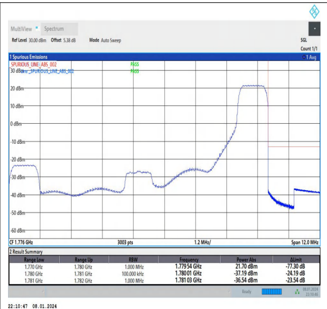
Band66_10MHz_16QAM_132622_1RB#49
