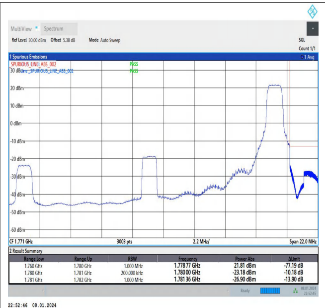
Band66_20MHz_16QAM_132572_1RB#99
