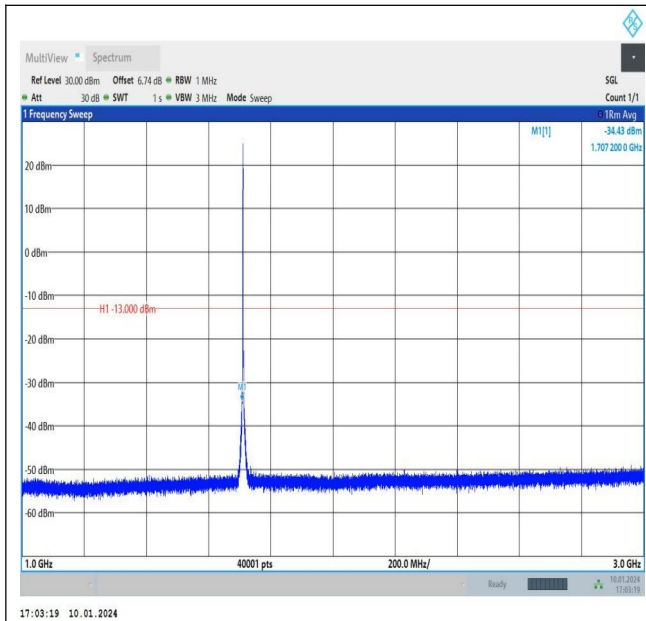
Band66_1.4MHz_16QAM_131979_1RB#0_1000~3000_1000~3000
