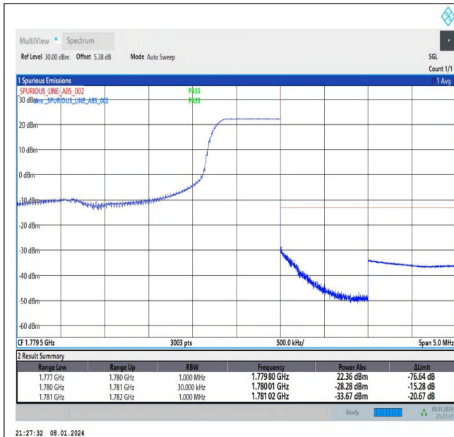
Band66_3MHz_QPSK_132657_1RB#14
