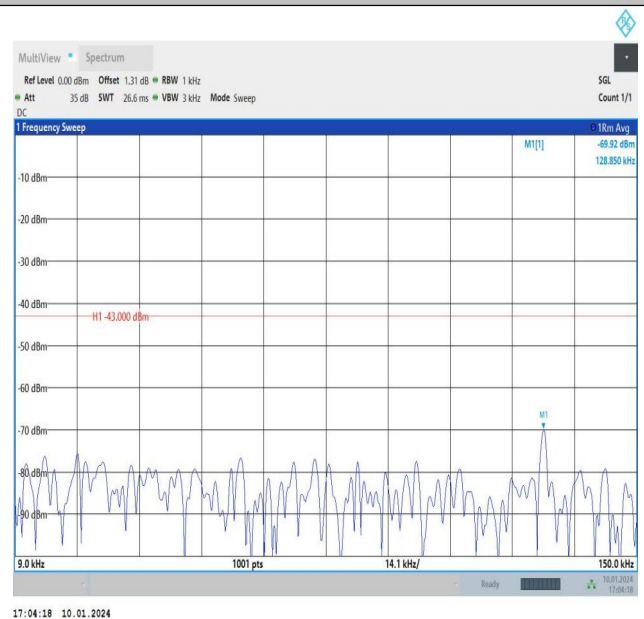
Band66_1.4MHz_16QAM_132322_1RB#0_0.009~0.15_0.009~0.15
