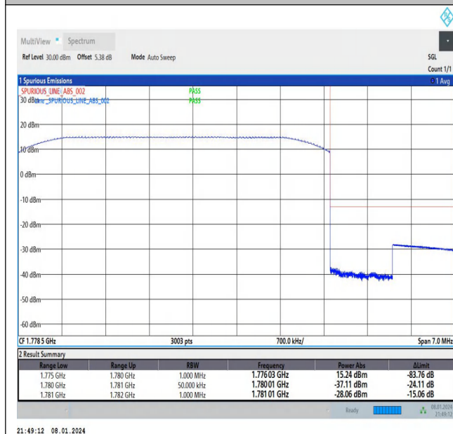
Band66_5MHz_QPSK_132647_25RB#0
