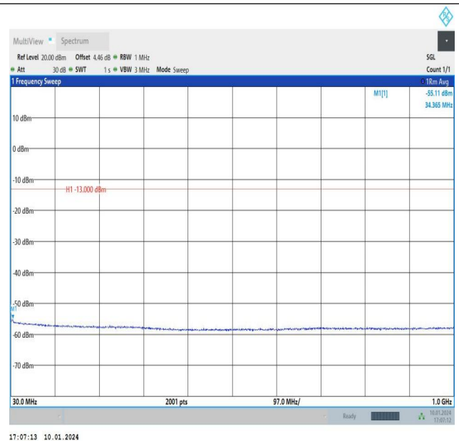
Band66_3MHz_16QAM_131987_1RB#0_30~1000_30~10 00
