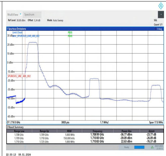
Band66_15MHz_16QAM_132047_1RB#0
