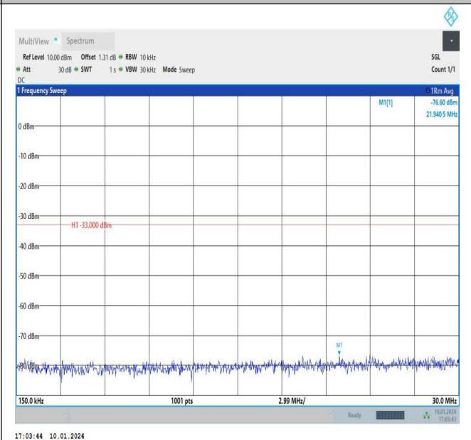
Band66_1.4MHz_QPSK_132322_1RB#0_0.15~30_0.15~30
