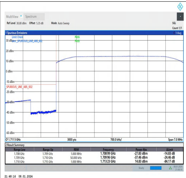
Band66_5MHz_16QAM_131997_25RB#0
