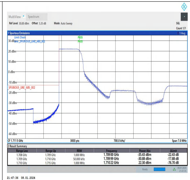
Band66_5MHz_16QAM_131997_1RB#0
