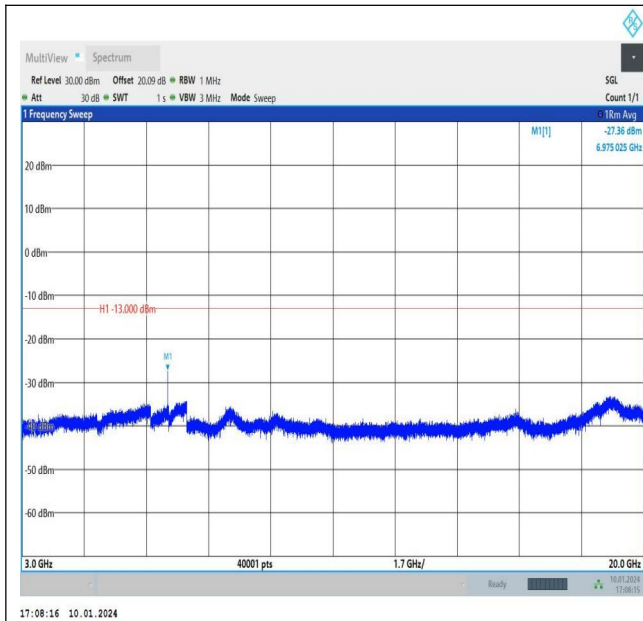
Band66_3MHz_QPSK_132322_1RB#0_3000~20000_300 0~20000
