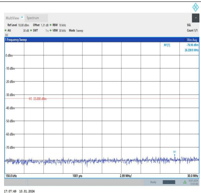
Band66_3MHz_QPSK_132322_1RB#0_0.15~30_0.15~30
