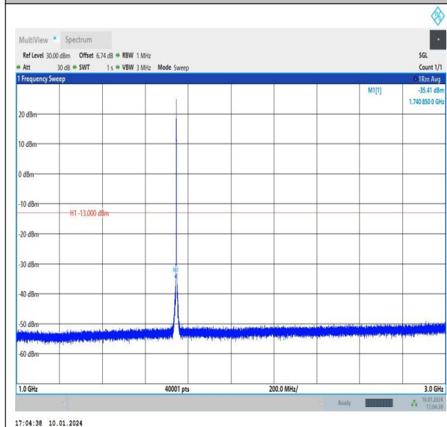
Band66_1.4MHz_16QAM_132322_1RB#0_1000~3000_1 000~3000
