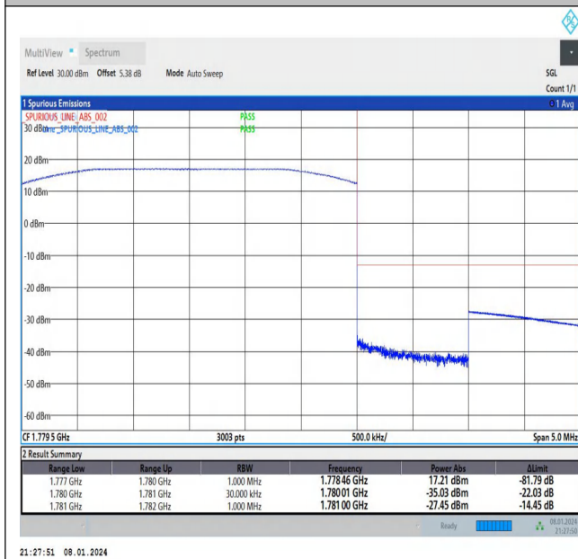
Band66_3MHz_QPSK_132657_15RB#0
