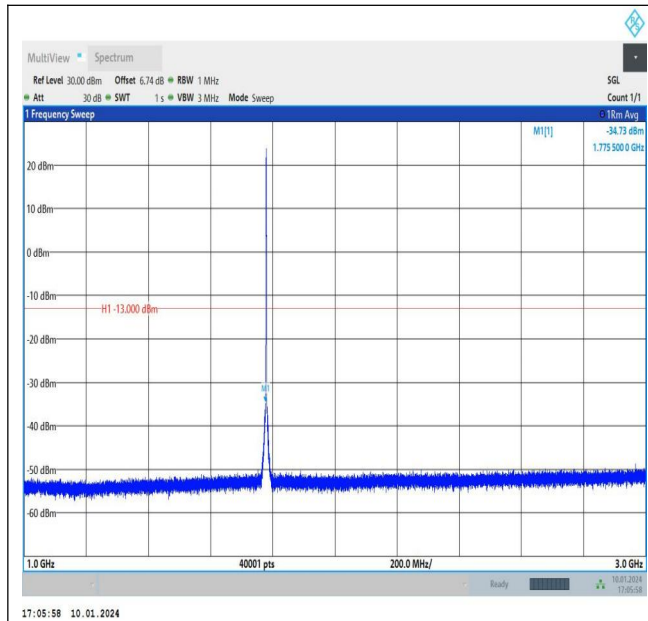
Band66_1.4MHz_16QAM_132665_1RB#0_1000~3000_1000~3000
