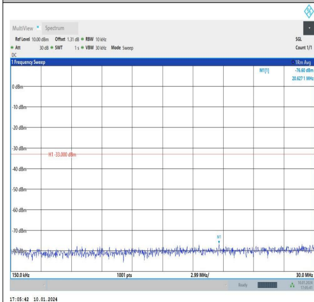
Band66_1.4MHz_16QAM_132665_1RB#0_0.15~30_0.15~30
