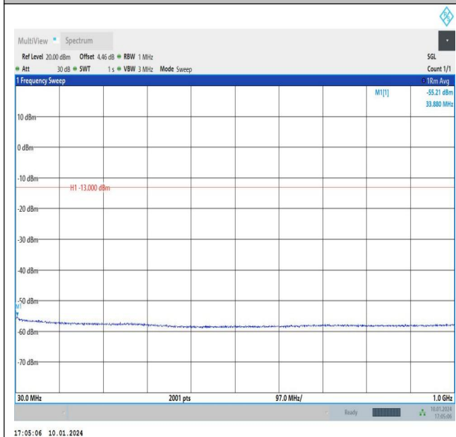
Band66_1.4MHz_QPSK_132665_1RB#0_30~1000_30~1000
