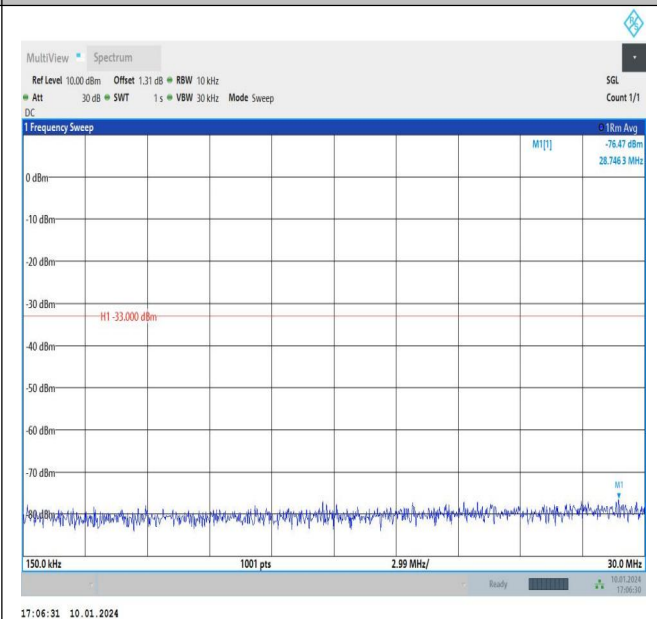
Band66_3MHz_QPSK_131987_1RB#0_0.15~30_0.15~30
