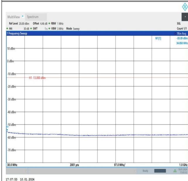
Band66_3MHz_QPSK_132322_1RB#0_30~1000_30~100 0
