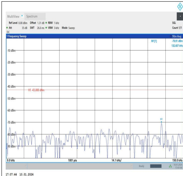
Band66_3MHz_QPSK_132322_1RB#0_0.009~0.15_0.00 9~0.15
