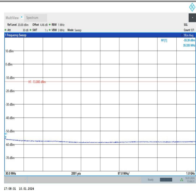
Band66_3MHz_16QAM_132322_1RB#0_30~1000_30~10 00
