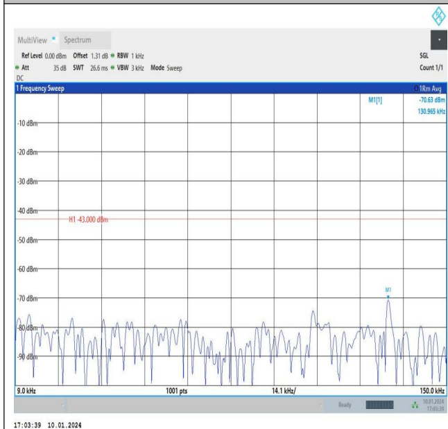
Band66_1.4MHz_QPSK_132322_1RB#0_0.009~0.15_0.009~0.15
