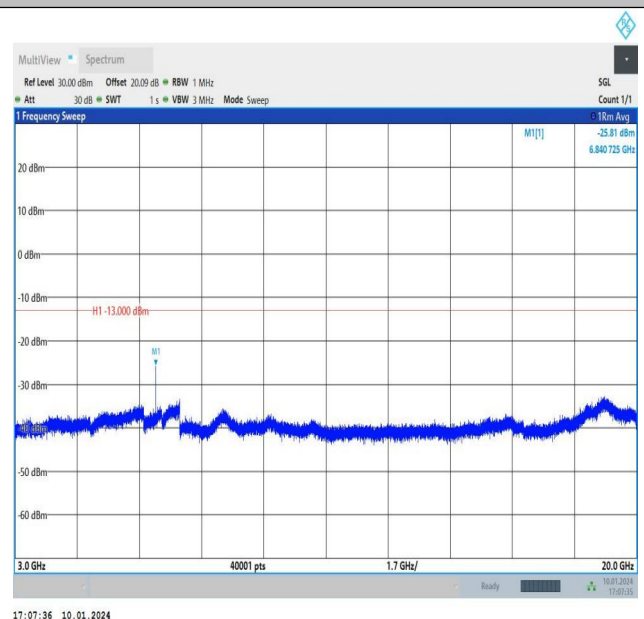
Band66_3MHz_16QAM_131987_1RB#0_3000~20000_30 00~20000
