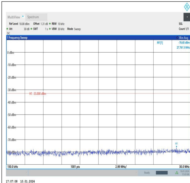
Band66_3MHz_16QAM_131987_1RB#0_0.15~30_0.15~3 0
