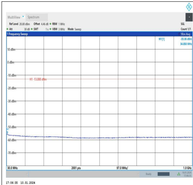
Band66_3MHz_QPSK_131987_1RB#0_30~1000_30~100 0
