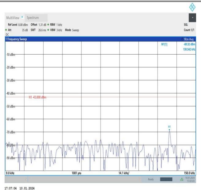
Band66_3MHz_16QAM_131987_1RB#0_0.009~0.15_0.009~0.15 9~0.15
