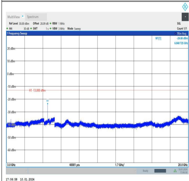
Band66_3MHz_QPSK_131987_1RB#0_3000~20000_3000~20000 0~20000
