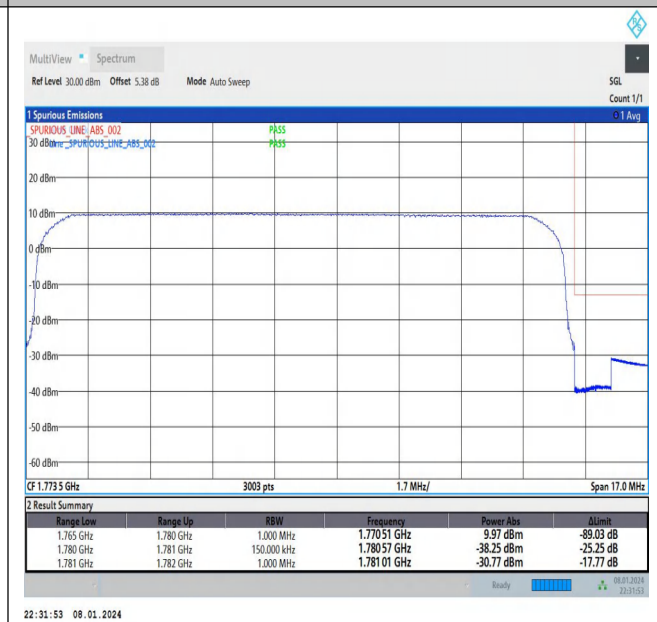
Band66_15MHz_16QAM_132597_75RB#0
