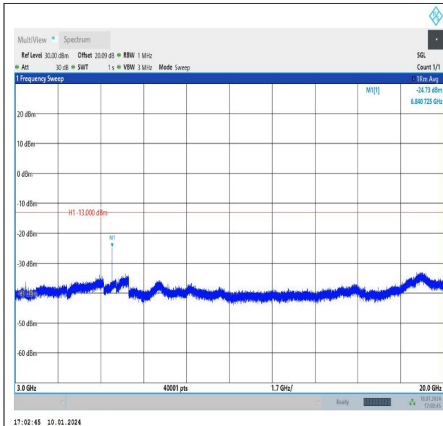
Band66_1.4MHz_QPSK_131979_1RB#0_3000~20000_3 000~20000
