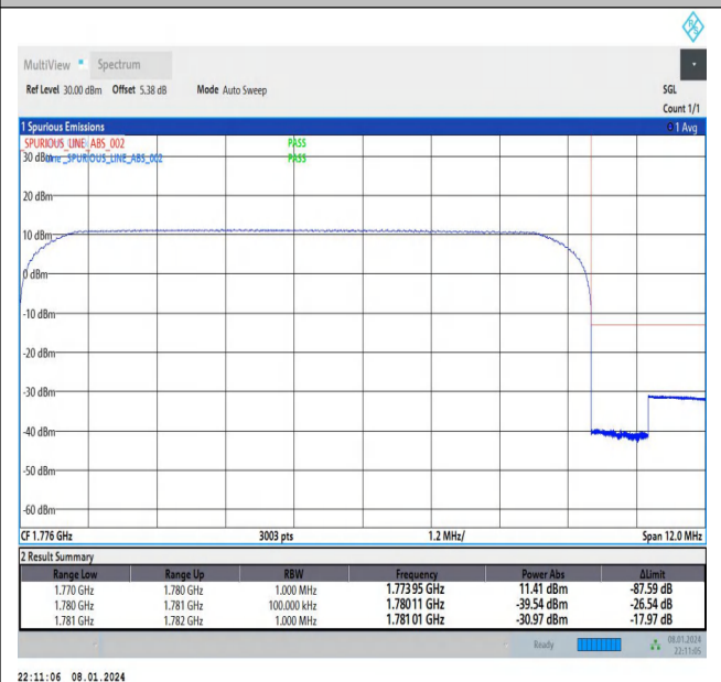
Band66_10MHz_16QAM_132622_50RB#0
