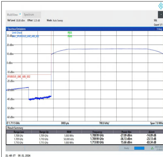
Band66_5MHz_QPSK_131997_25RB#0
