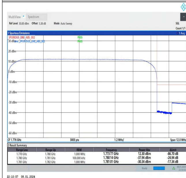
Band66_10MHz_QPSK_132622_50RB#0
