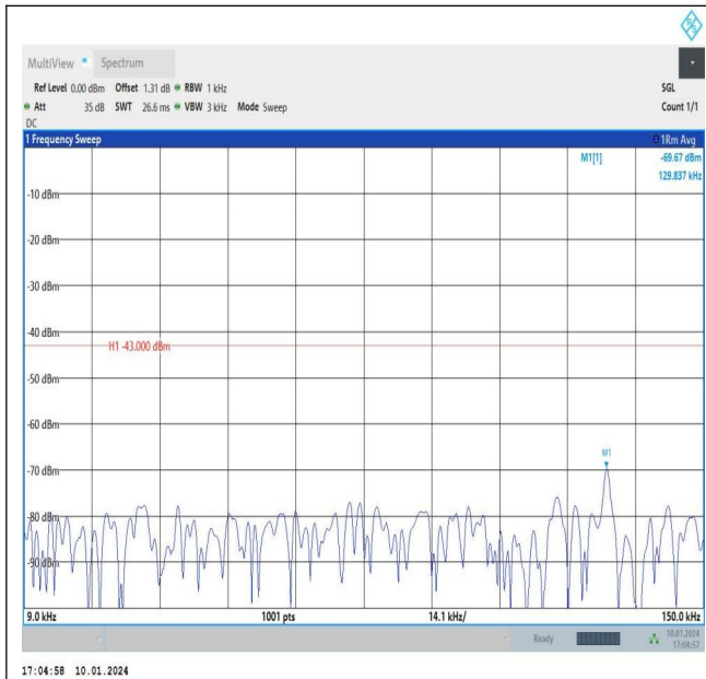
Band66_1.4MHz_QPSK_132665_1RB#0_0.009~0.15_0.09~0.15
