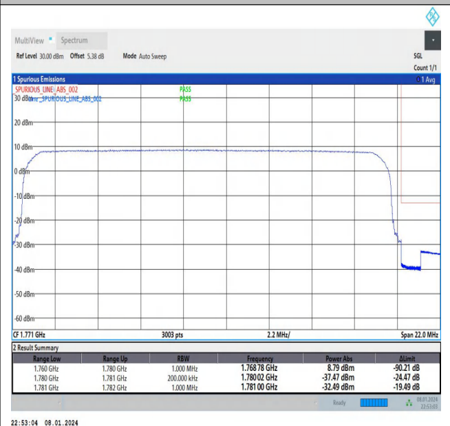
Band66_20MHz_16QAM_132572_100RB#0
