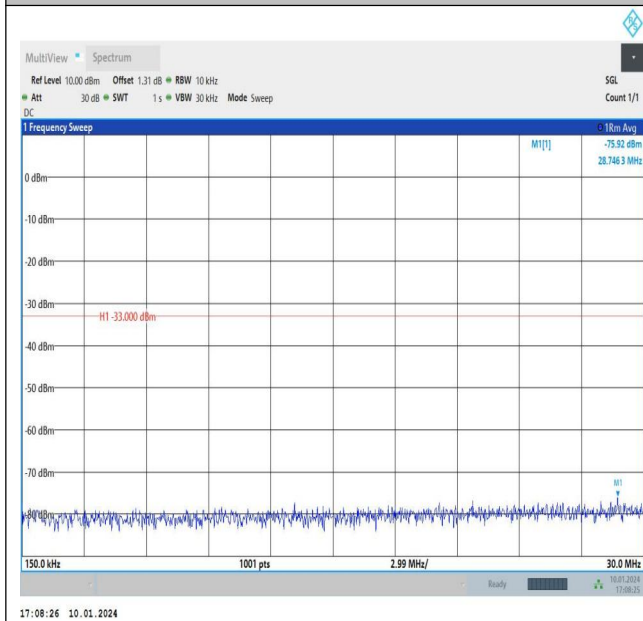
Band66_3MHz_16QAM_132322_1RB#0_0.15~30_0.15~3 0
