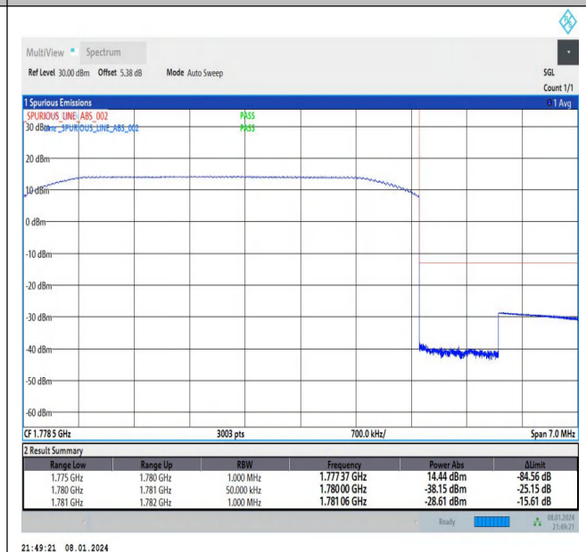
Band66_5MHz_16QAM_132647_25RB#0
