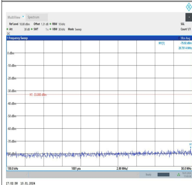
Band66_1.4MHz_16QAM_131979_1RB#0_0.15~30_0.15 ~30
