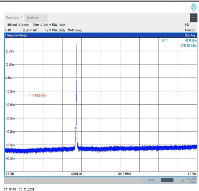
Band66_3MHz_QPSK_132322_1RB#0_1000~3000_1000~3000
