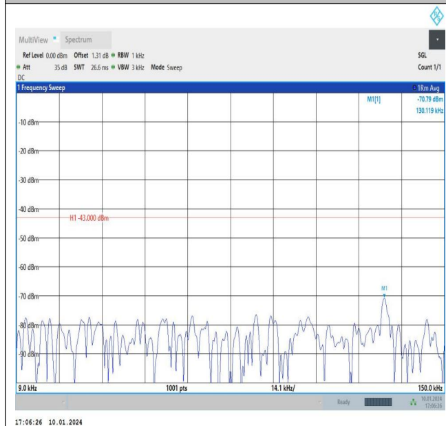
Band66_3MHz_QPSK_131987_1RB#0_0.009~0.15_0.009~0.15
