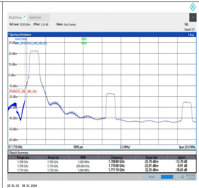
Band66_20MHz_16QAM_132072_1RB#0
