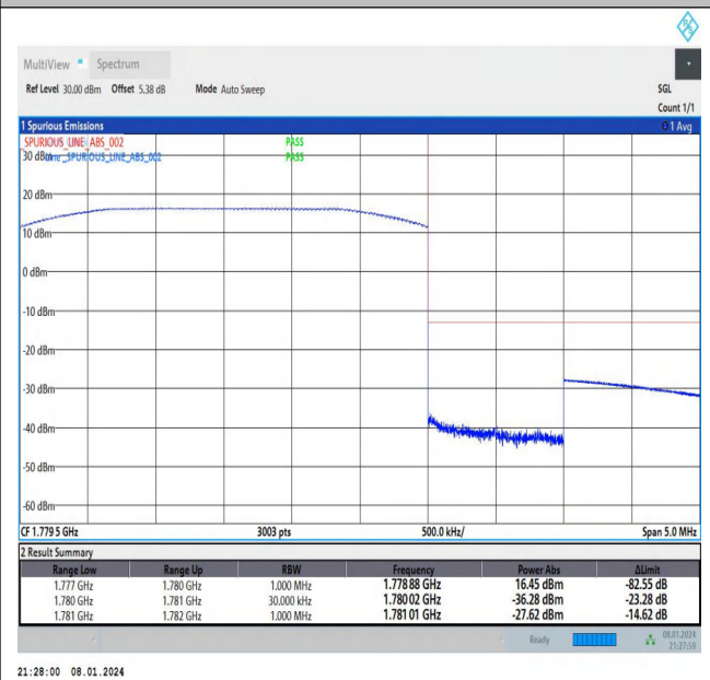
Band66_3MHz_16QAM_132657_15RB#0
