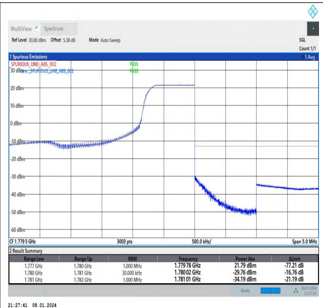
Band66_3MHz_16QAM_132657_1RB#14
