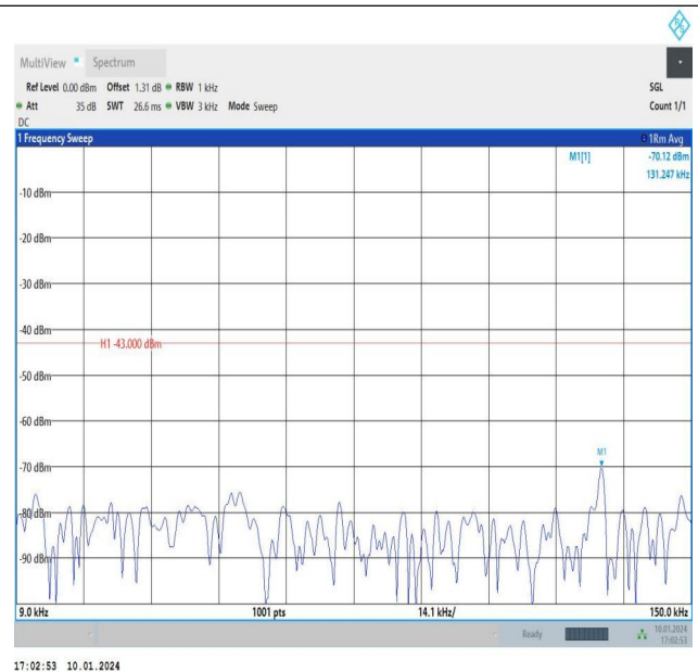
Band66_1.4MHz_16QAM_131979_1RB#0_0.009~0.15_0. 009~0.15
