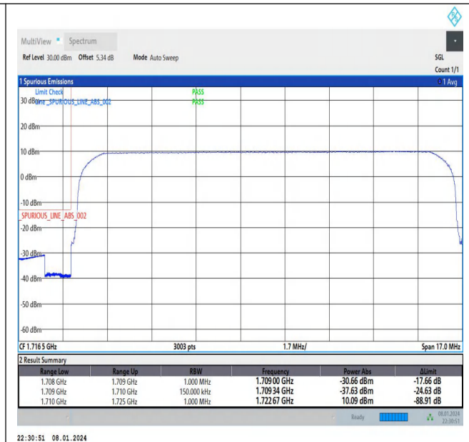
Band66_15MHz_16QAM_132047_75RB#0
