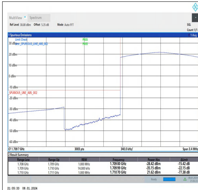
Band66_1.4MHz_QPSK_131979_6RB#0
