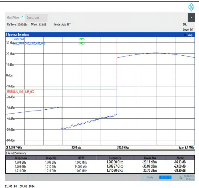
Band66_1.4MHz_16QAM_131979_6RB#0
