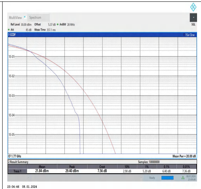
Band66-20MHz-16QAM-132572-1RB#0-PASS
