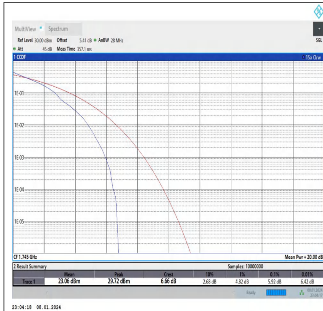
Band66-20MHz-QPSK-132322-1RB#0-PASS
