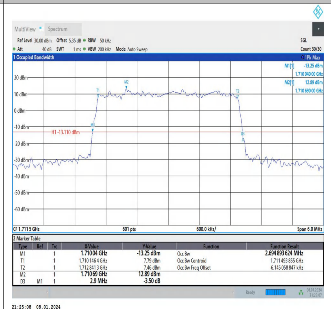
Band66-3MHz-16QAM-131987-15RB#0-PASS
