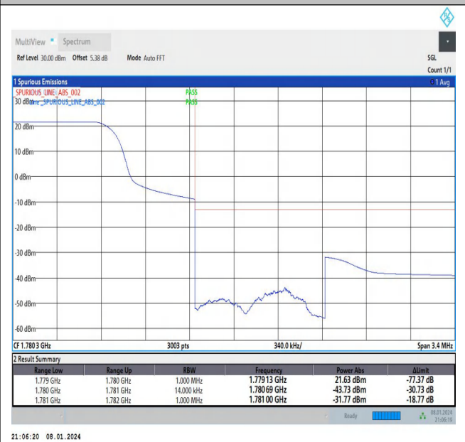
Band66_1.4MHz_16QAM_132665_1RB#0
