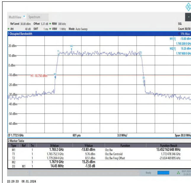
Band66-15MHz-QPSK-132597-75RB#0-PASS
