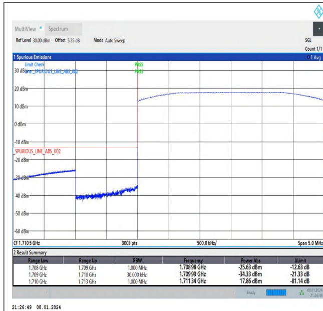
Band66_3MHz_QPSK_131987_15RB#0
