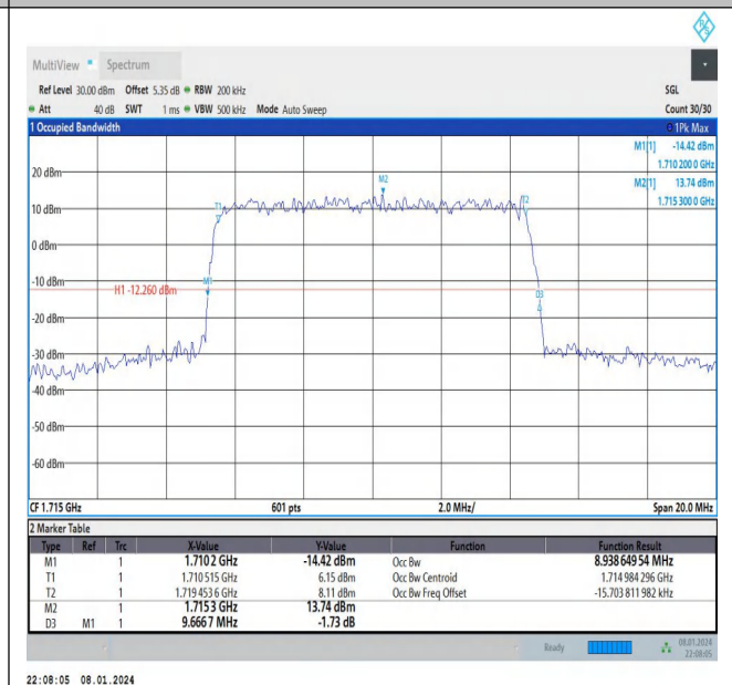
Band66-10MHz-16QAM-132022-50RB#0-PASS
