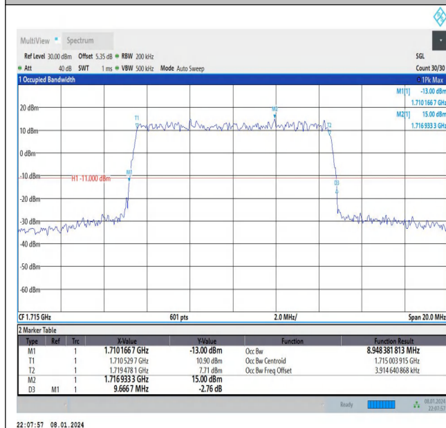
Band66-10MHz-QPSK-132022-50RB#0-PASS
