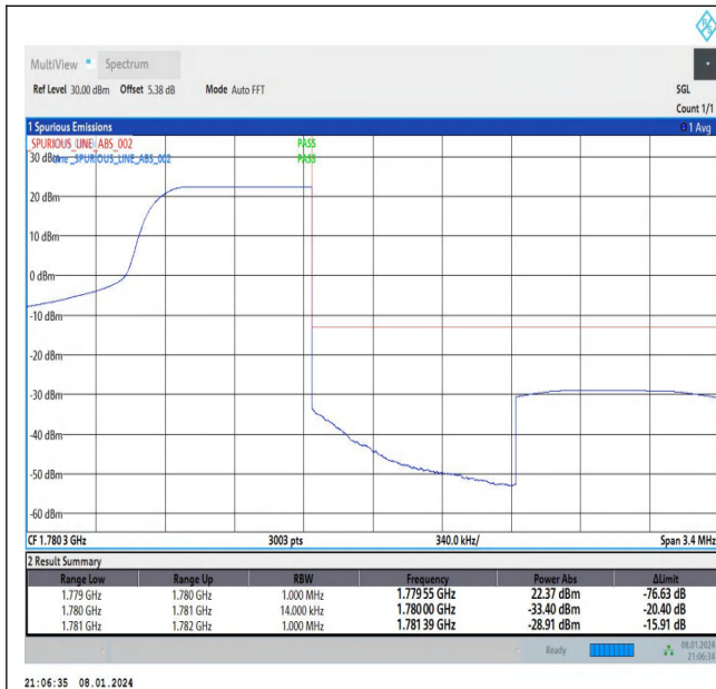
Band66_1.4MHz_QPSK_132665_1RB#5
