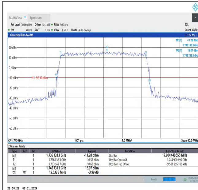
Band66-20MHz-QPSK-132322-100RB#0-PASS
