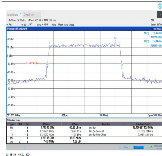
Band66-15MHz-QPSK-132047-75RB#0-PASS
