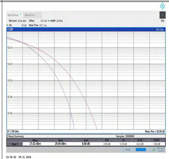
Band66-20MHz-16QAM-132322-100RB#0-PASS
