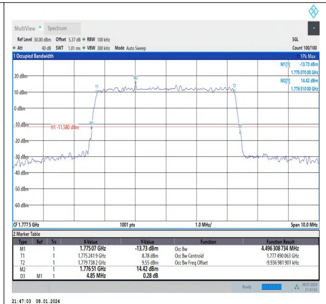
Band66-5MHz-16QAM-132647-25RB#0-PASS
