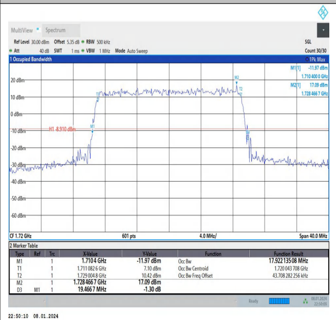
Band66-20MHz-16QAM-132072-100RB#0-PASS
