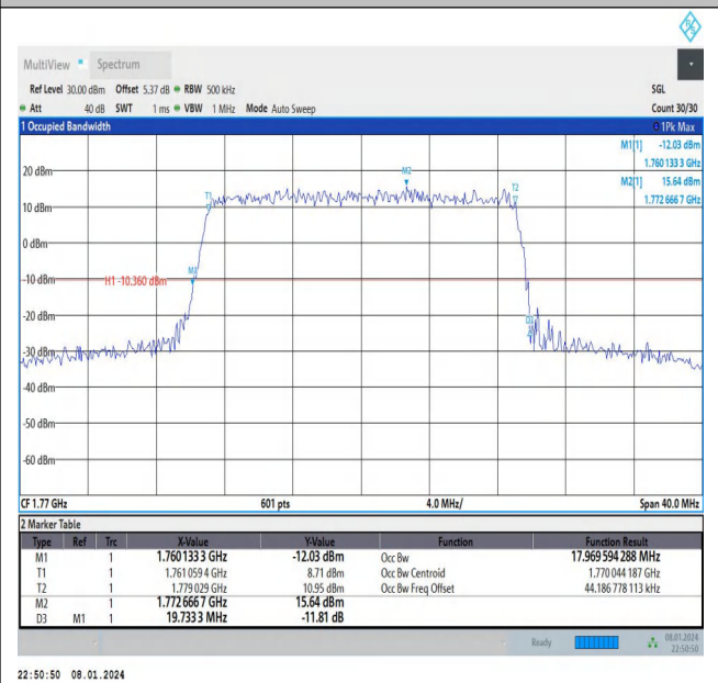
Band66-20MHz-16QAM-132572-100RB#0-PASS
