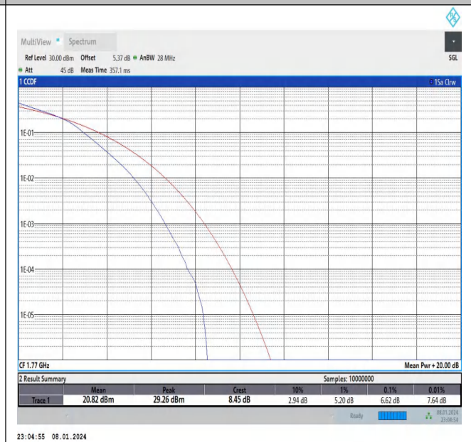
Band66-20MHz-16QAM-132572-100RB#0-PASS
