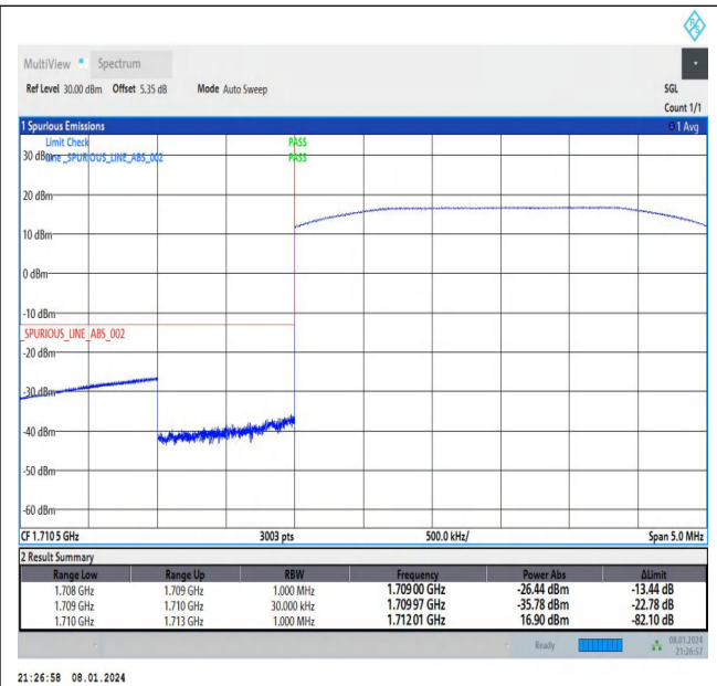
Band66_3MHz_16QAM_131987_15RB#0
