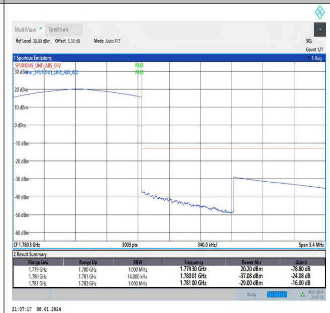
Band66_1.4MHz_16QAM_132665_6RB#0
