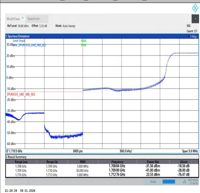
Band66_3MHz_16QAM_131987_1RB#14
