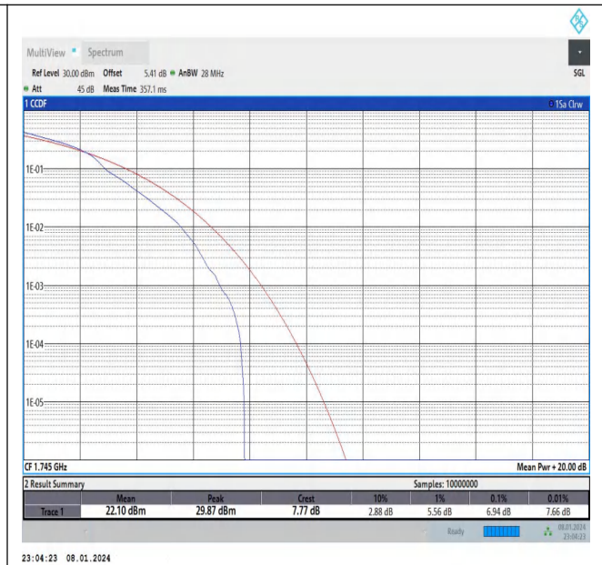
Band66-20MHz-16QAM-132322-1RB#0-PASS
