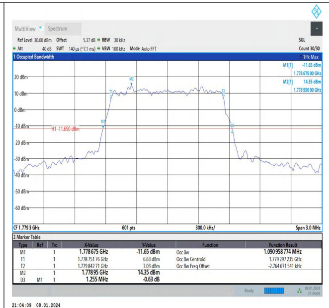
Band66-1.4MHz-16QAM-132665-6RB#0-PASS
