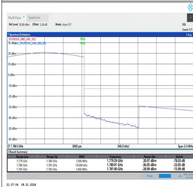
Band66_1.4MHz_QPSK_132665_6RB#0
