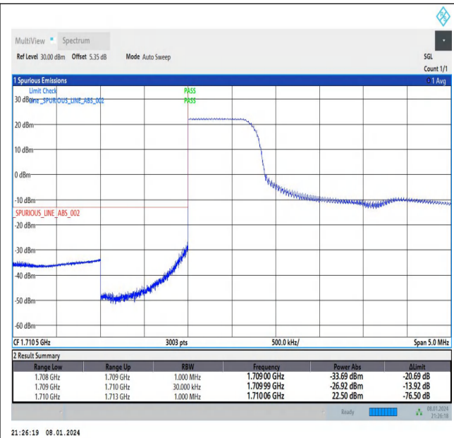
Band66_3MHz_16QAM_131987_1RB#0
