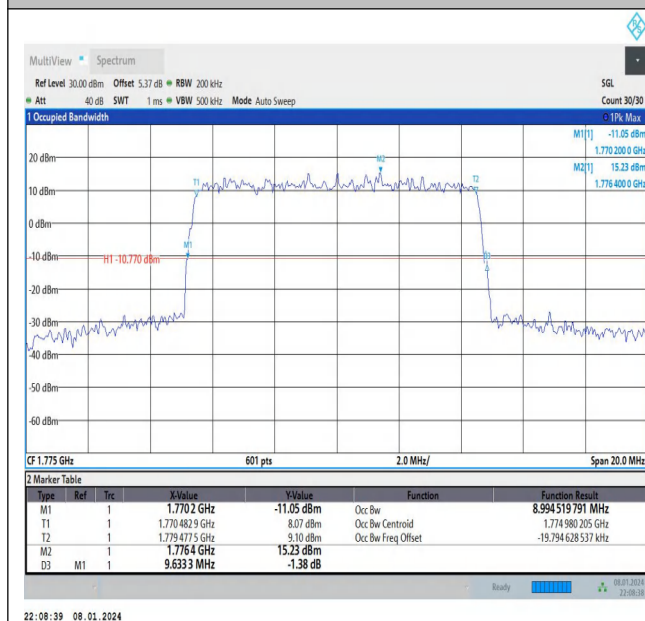
Band66-10MHz-QPSK-132622-50RB#0-PASS
