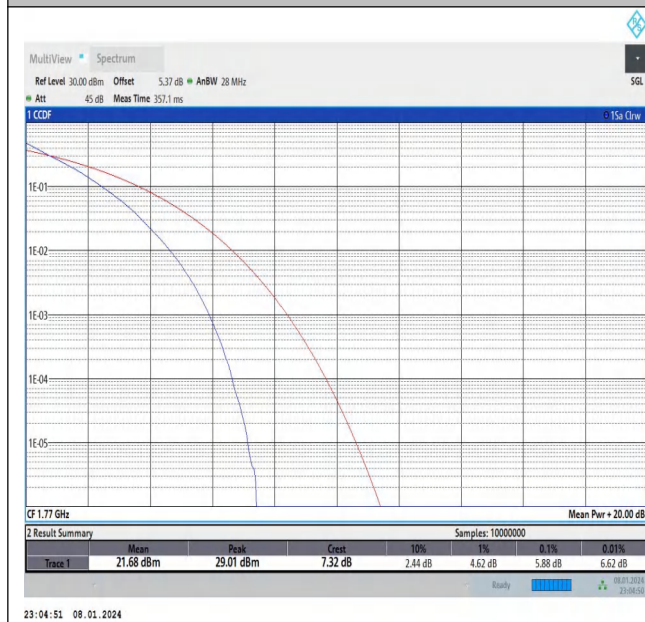
Band66-20MHz-QPSK-132572-100RB#0-PASS
