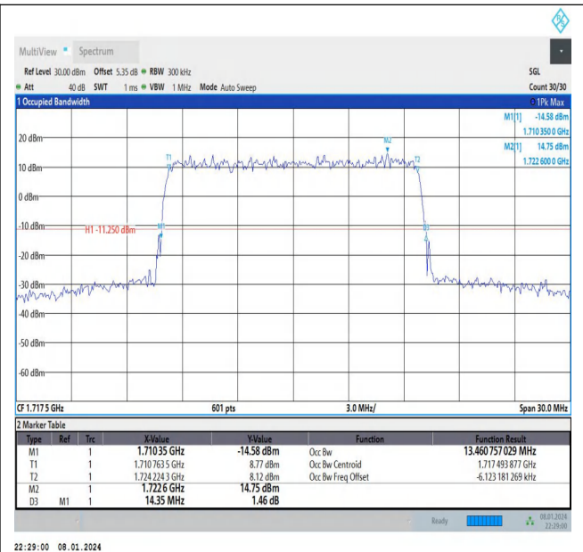
Band66-15MHz-16QAM-132047-75RB#0-PASS
