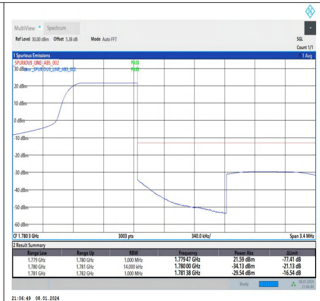
Band66_1.4MHz_16QAM_132665_1RB#5
