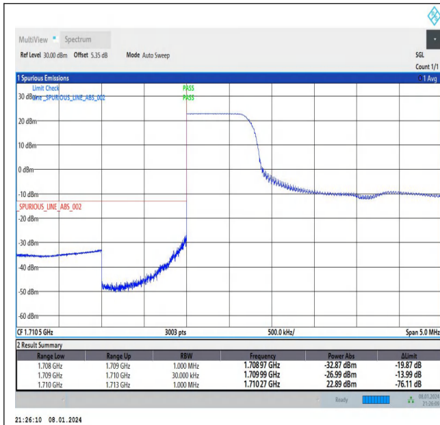
Band66_3MHz_QPSK_131987_1RB#0
