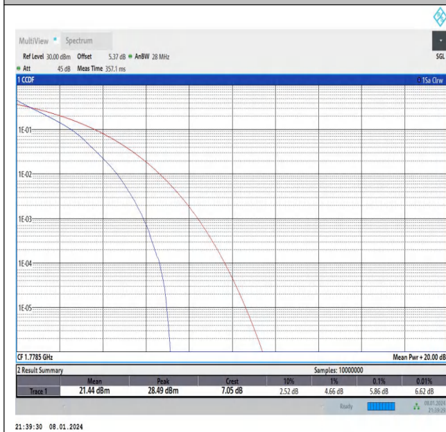
Band66-3MHz-QPSK-132657-15RB#0-PASS
