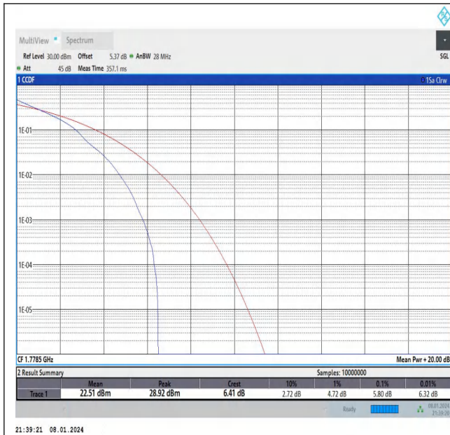
Band66-3MHz-QPSK-132657-1RB#0-PASS
