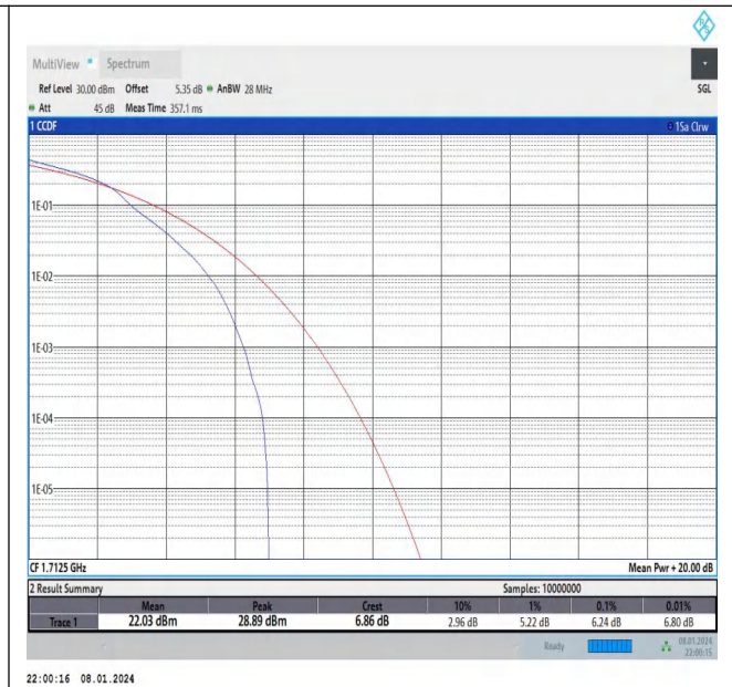
Band66-5MHz-16QAM-131997-1RB#0-PASS
