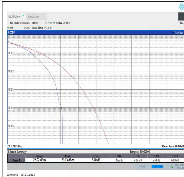
Band66-15MHz-QPSK-132047-1RB#0-PASS
