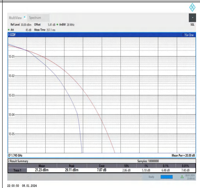
Band66-5MHz-16QAM-132322-25RB#0-PASS
