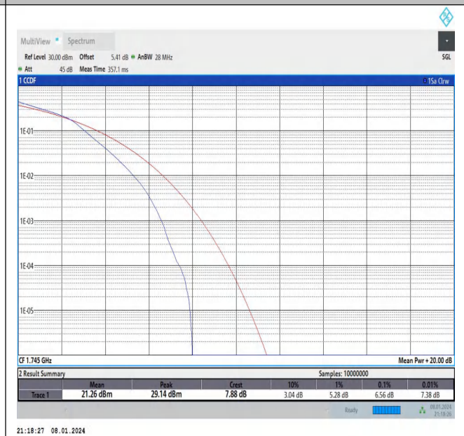
Band66-1.4MHz-16QAM-132322-6RB#0-PASS
