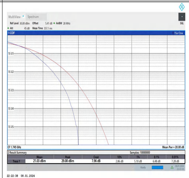
Band66-10MHz-16QAM-132322-50RB#0-PASS
