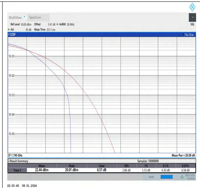
Band66-5MHz-16QAM-132322-1RB#0-PASS
