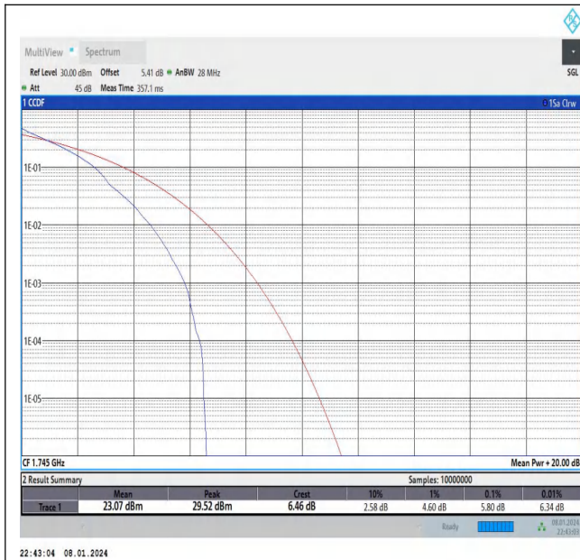
Band66-15MHz-QPSK-132322-1RB#0-PASS
