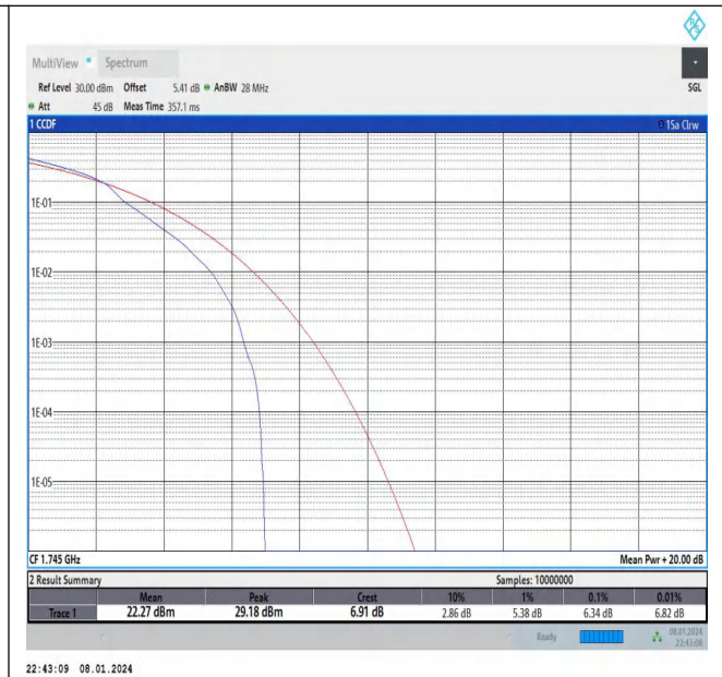
Band66-15MHz-16QAM-132322-1RB#0-PASS
