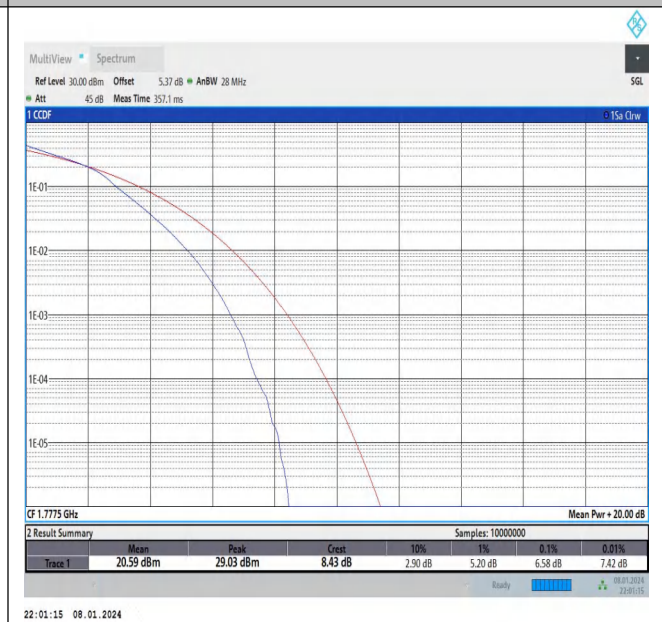
Band66-5MHz-16QAM-132647-25RB#0-PASS
