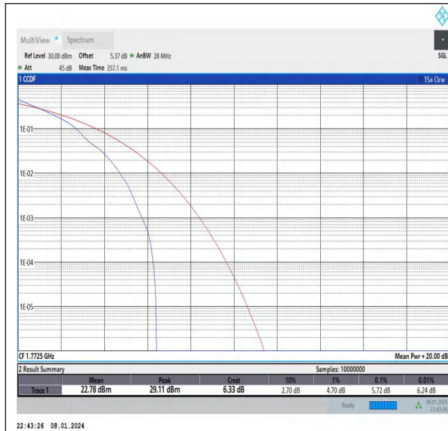
Band66-15MHz-QPSK-132597-1RB#0-PASS
