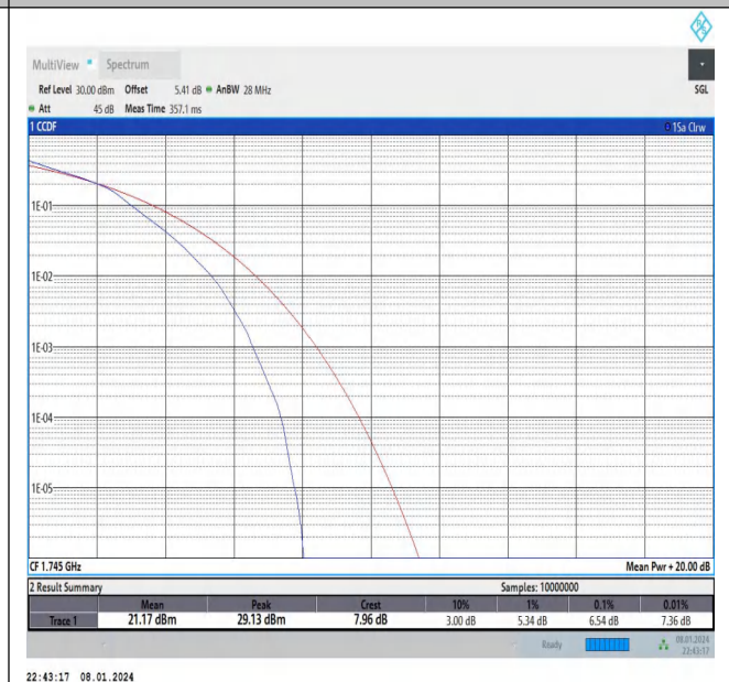
Band66-15MHz-16QAM-132322-75RB#0-PASS
