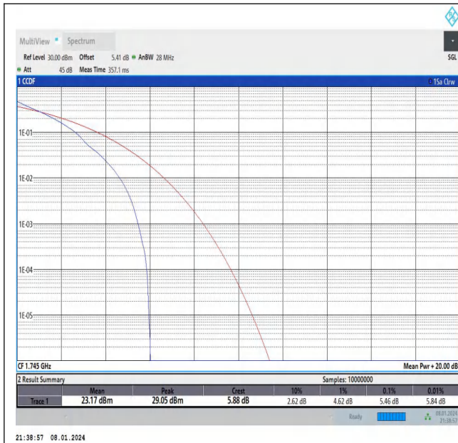
Band66-3MHz-QPSK-132322-1RB#0-PASS
