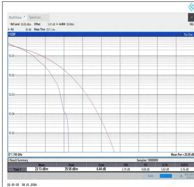
Band66-5MHz-QPSK-132322-1RB#0-PASS
