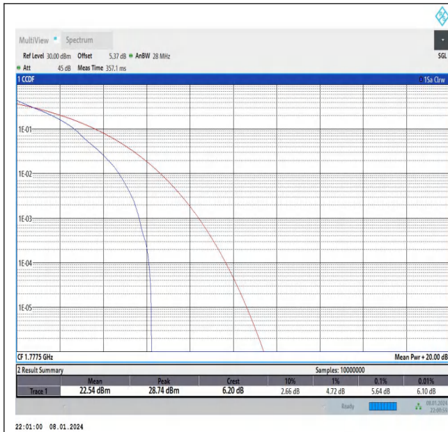
Band66-5MHz-QPSK-132647-1RB#0-PASS
