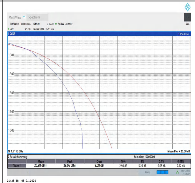
Band66-3MHz-16QAM-131987-15RB#0-PASS
