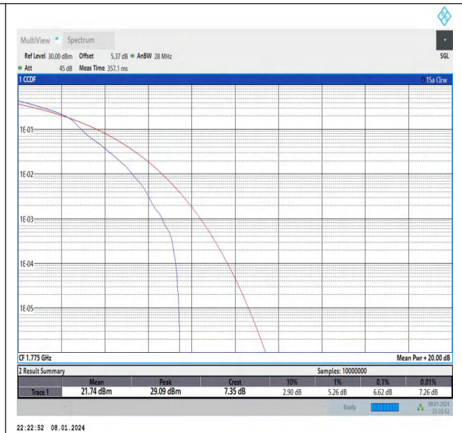
Band66-10MHz-16QAM-132622-1RB#0-PASS
