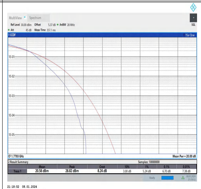
Band66-1.4MHz-16QAM-132665-6RB#0-PASS
