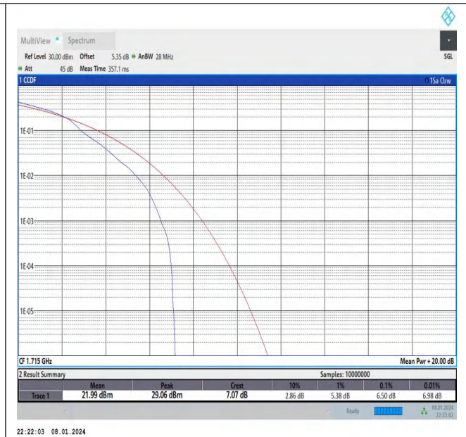
Band66-10MHz-16QAM-132022-1RB#0-PASS
