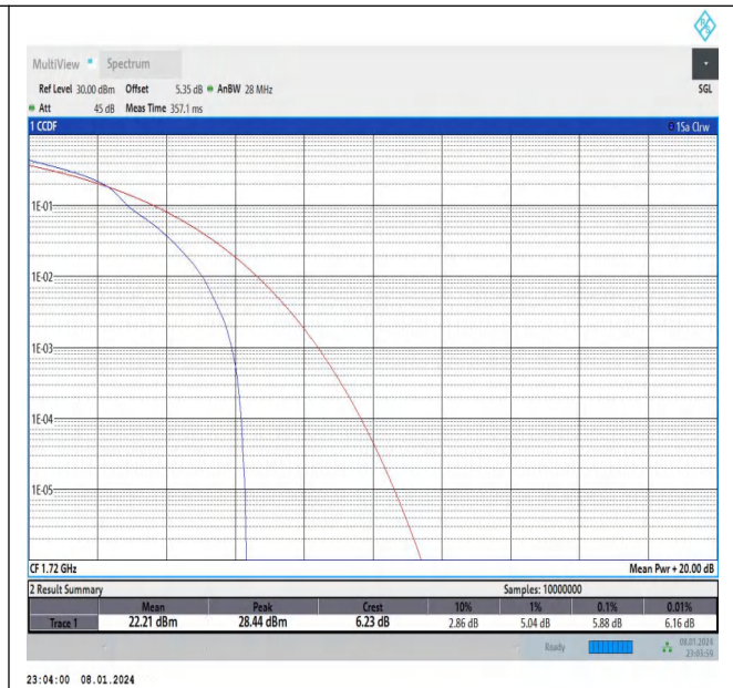
Band66-20MHz-16QAM-132072-1RB#0-PASS
