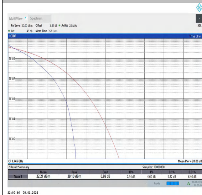
Band66-5MHz-QPSK-132322-25RB#0-PASS
