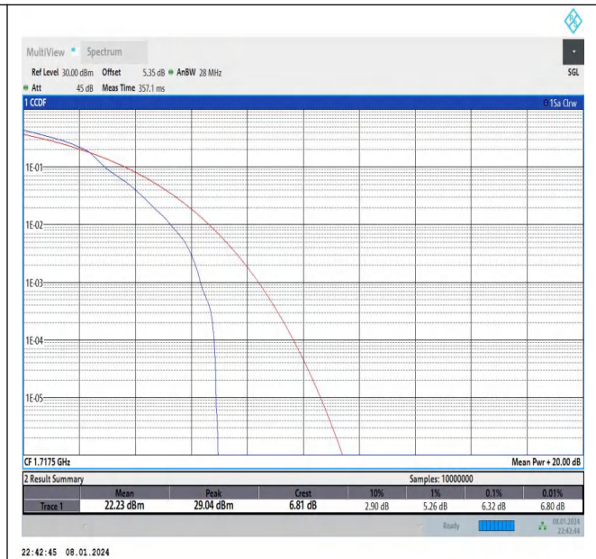
Band66-15MHz-16QAM-132047-1RB#0-PASS
