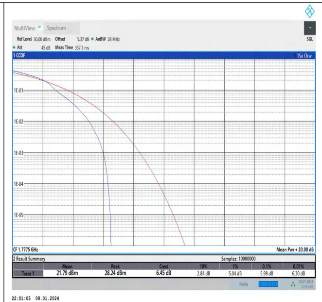
Band66-5MHz-16QAM-132647-1RB#0-PASS
