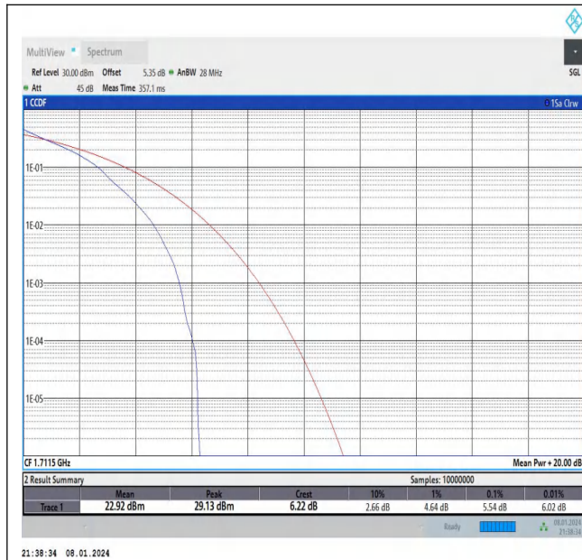
Band66-3MHz-QPSK-131987-1RB#0-PASS
