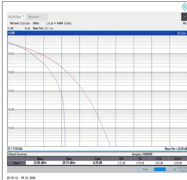
Band66-5MHz-QPSK-131997-1RB#0-PASS
