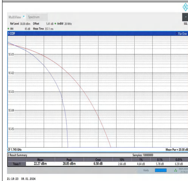
Band66-1.4MHz-QPSK-132322-6RB#0-PASS
