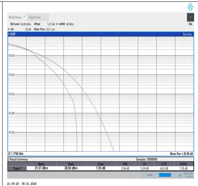
Band66-3MHz-16QAM-132657-1RB#0-PASS
