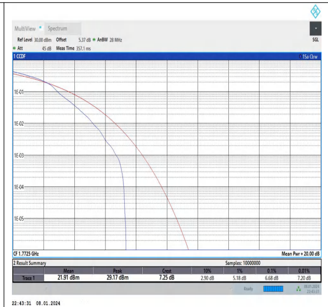
Band66-15MHz-16QAM-132597-1RB#0-PASS
