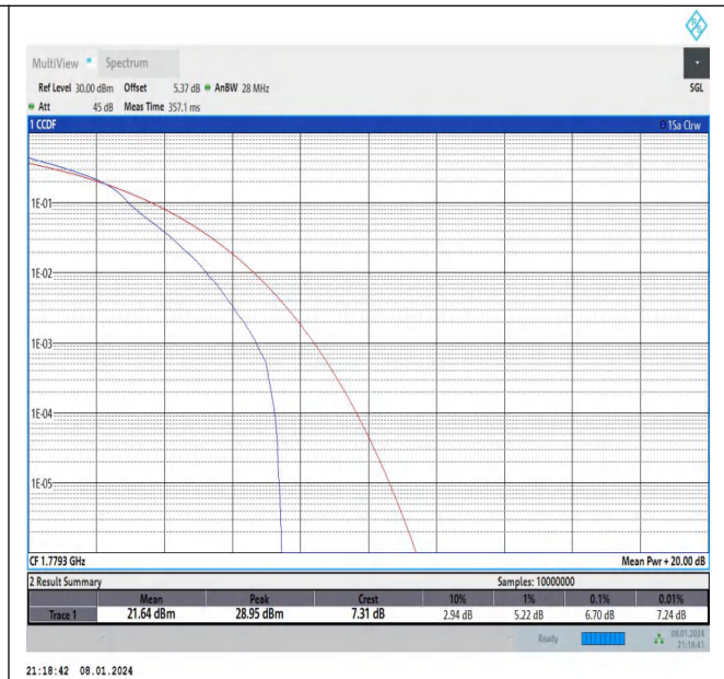
Band66-1.4MHz-16QAM-132665-1RB#0-PASS
