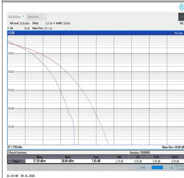
Band66-1.4MHz-QPSK-132665-6RB#0-PASS
