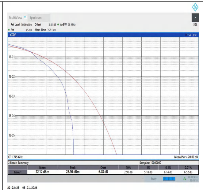
Band66-10MHz-16QAM-132322-1RB#0-PASS
