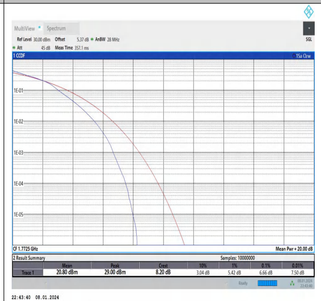
Band66-15MHz-16QAM-132597-75RB#0-PASS
