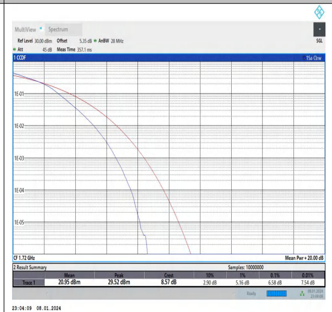
Band66-20MHz-16QAM-132072-100RB#0-PASS
