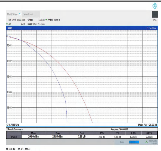
Band66-5MHz-16QAM-131997-25RB#0-PASS
