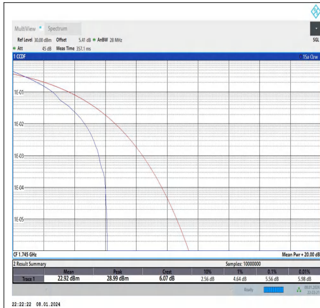
Band66-10MHz-QPSK-132322-1RB#0-PASS
