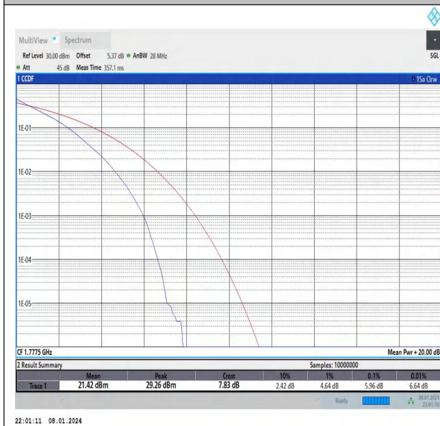
Band66-5MHz-QPSK-132647-25RB#0-PASS
