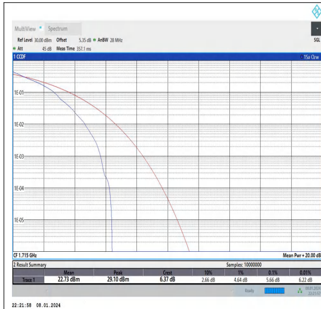
Band66-10MHz-QPSK-132022-1RB#0-PASS
