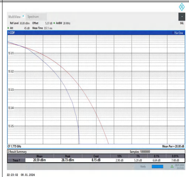
Band66-10MHz-16QAM-132622-50RB#0-PASS
