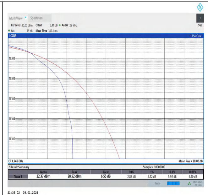
Band66-3MHz-16QAM-132322-1RB#0-PASS
