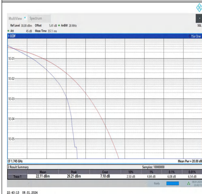
Band66-15MHz-QPSK-132322-75RB#0-PASS
