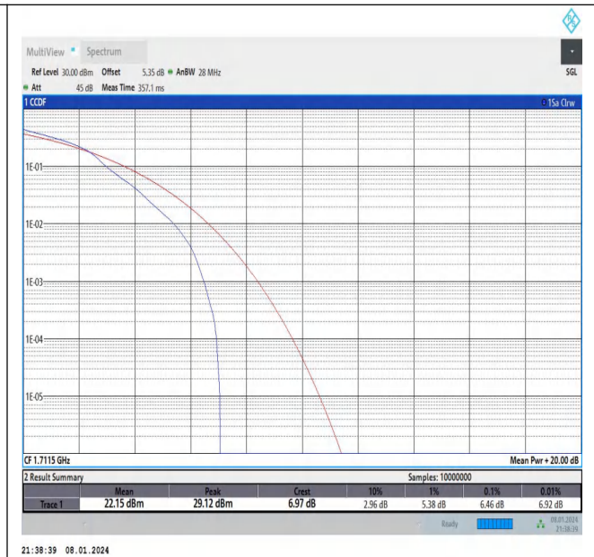
Band66-3MHz-16QAM-131987-1RB#0-PASS
