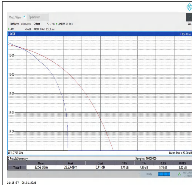
Band66-1.4MHz-QPSK-132665-1RB#0-PASS
