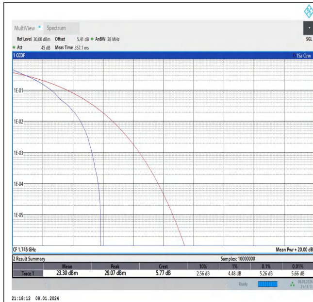
Band66-1.4MHz-QPSK-132322-1RB#0-PASS
