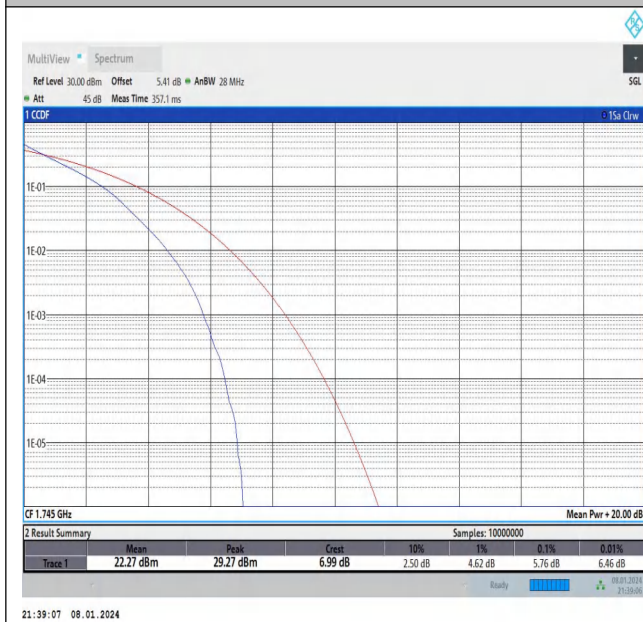
Band66-3MHz-QPSK-132322-15RB#0-PASS
