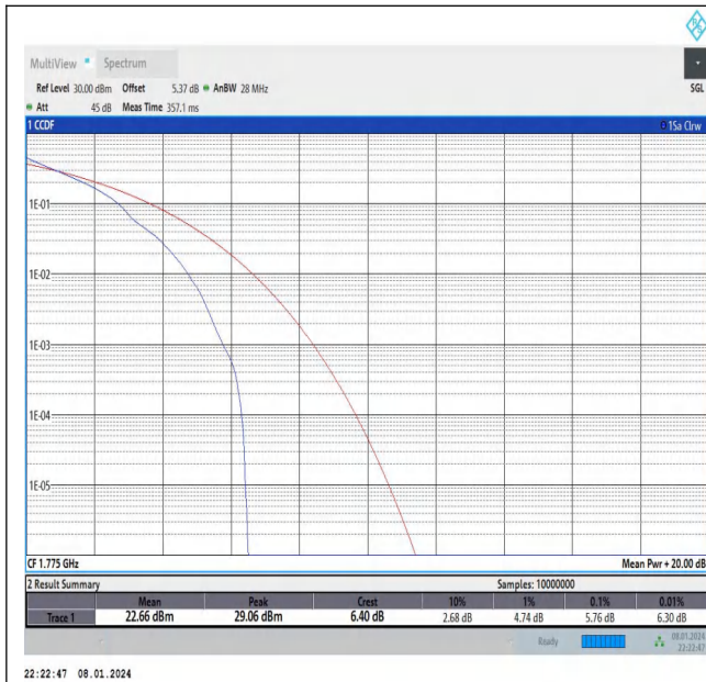
Band66-10MHz-QPSK-132622-1RB#0-PASS
