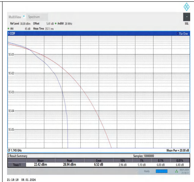
Band66-1.4MHz-16QAM-132322-1RB#0-PASS
