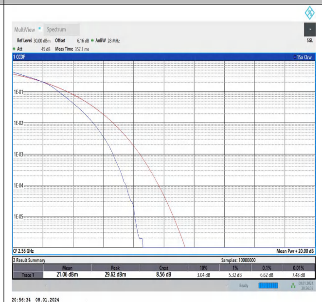
Band7-20MHz-16QAM-21350-100RB#0-PASS
