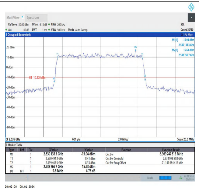
Band7-10MHz-16QAM-21100-50RB#0-PASS
