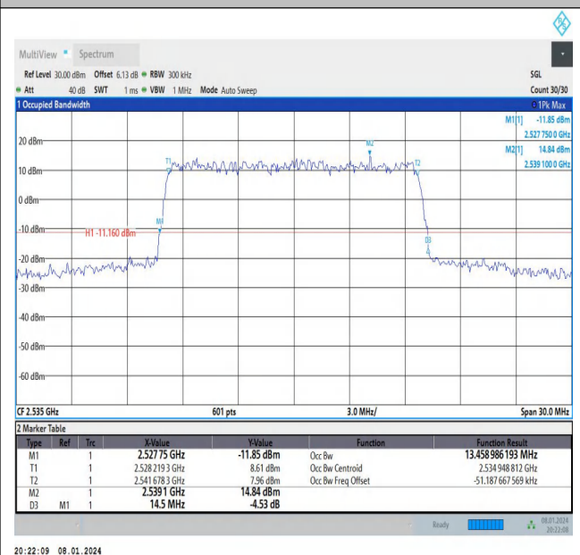
Band7-15MHz-16QAM-21100-75RB#0-PASS
