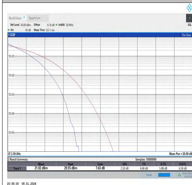
Band7-20MHz-QPSK-21350-100RB#0-PASS
