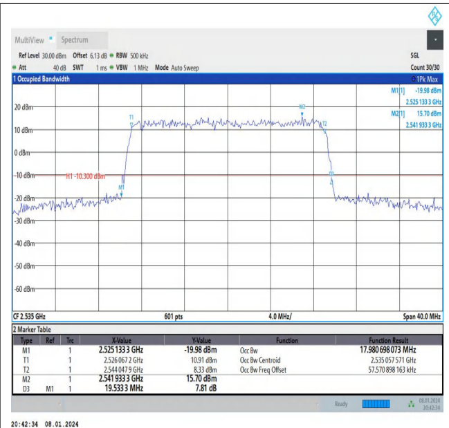
Band7-20MHz-16QAM-21100-100RB#0-PASS
