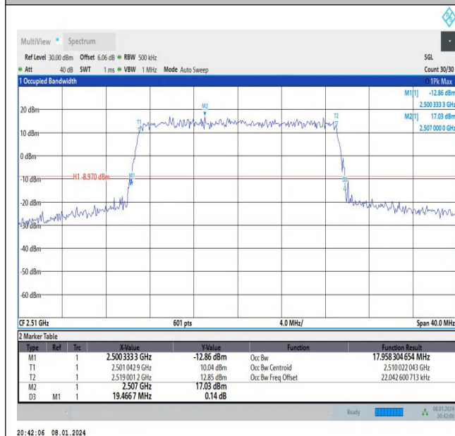
Band7-20MHz-QPSK-20850-100RB#0-PASS
