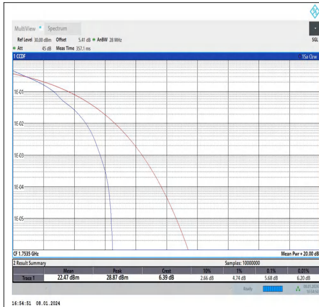
Band4-3MHz-QPSK-20385-1RB#0-PASS
