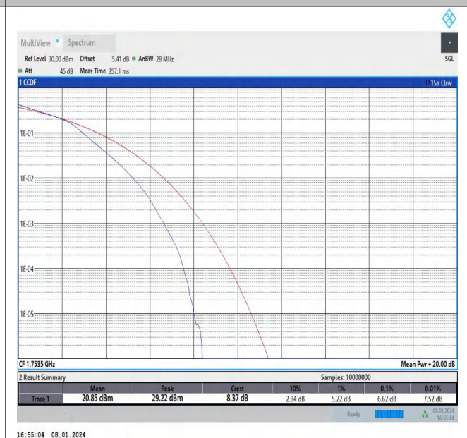
Band4-3MHz-16QAM-20385-15RB#0-PASS
