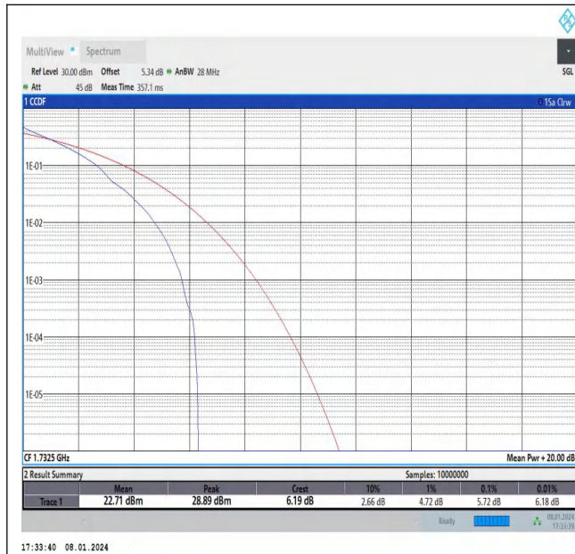
Band4-10MHz-QPSK-20175-1RB#0-PASS
