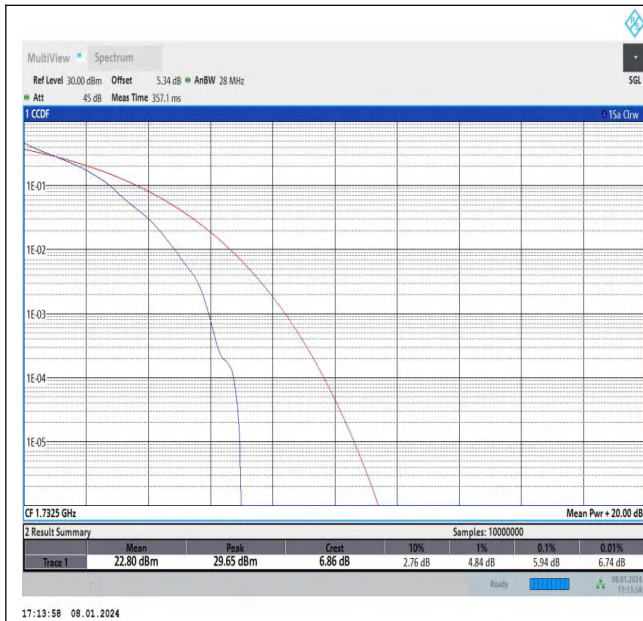
Band4-5MHz-QPSK-20175-1RB#0-PASS
