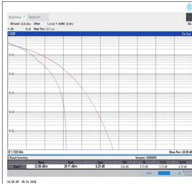
Band4-3MHz-QPSK-20175-1RB#0-PASS
