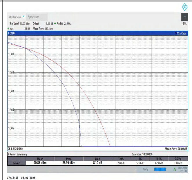
Band4-5MHz-16QAM-19975-25RB#0-PASS
