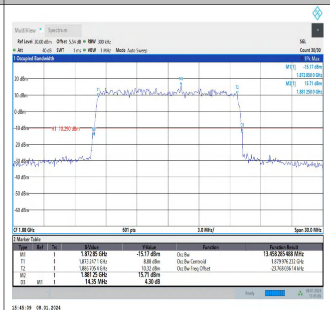
Band2-15MHz-16QAM-18900-75RB#0-PASS
