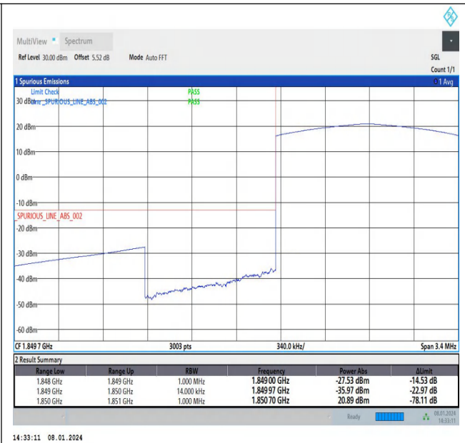
Band2_1.4MHz_16QAM_18607_6RB#0
