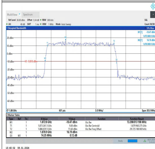
Band2-15MHz-QPSK-18900-75RB#0-PASS
