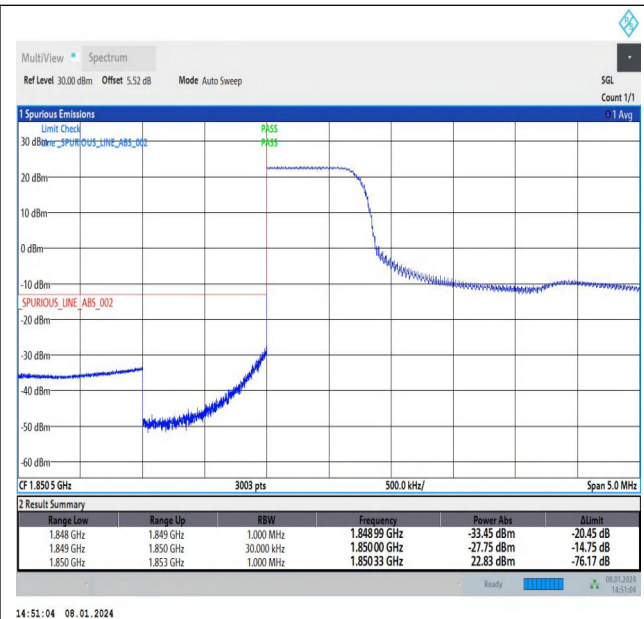
Band2_3MHz_16QAM_18615_1RB#0
