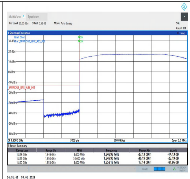
Band2_3MHz_16QAM_18615_15RB#0
