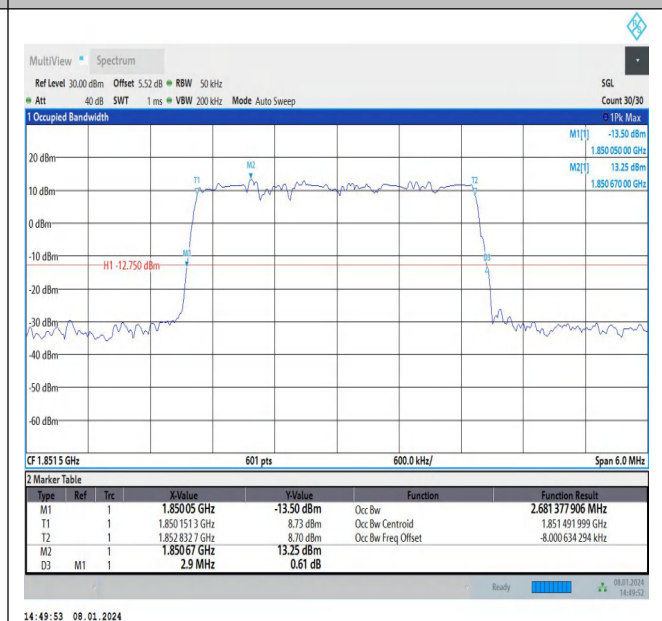
Band2-3MHz-16QAM-18615-15RB#0-PASS
