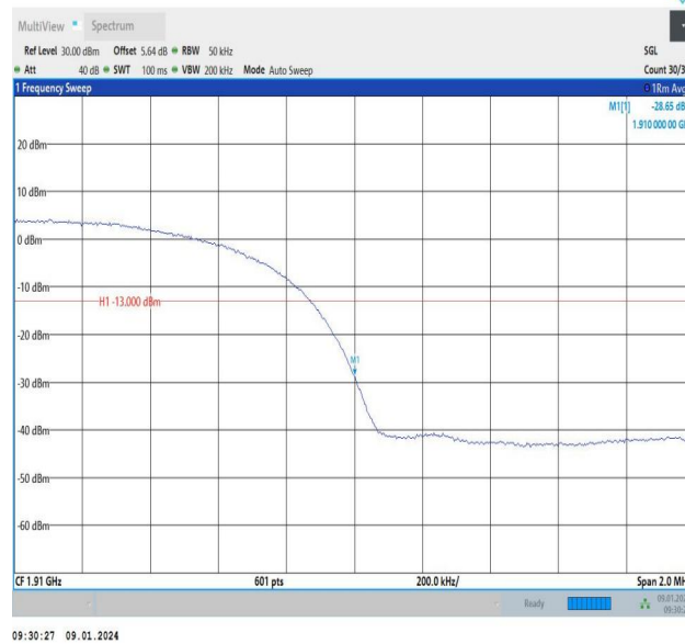
Band2-9538-PASS
