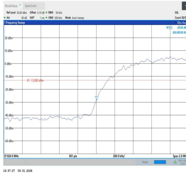
Band5-4132-PASS
