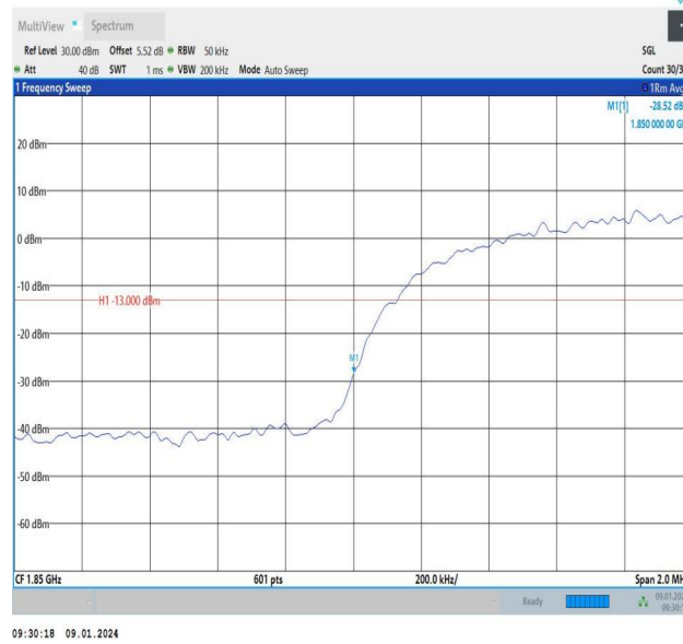
Band2-9262-PASS
