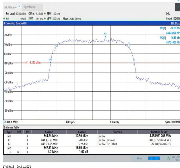
Band5-4233-4-PASS
