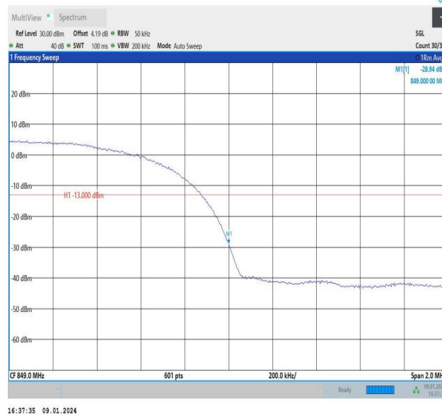
Band5-4233-PASS
