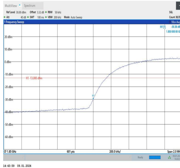
Band2-9262-2-PASS
