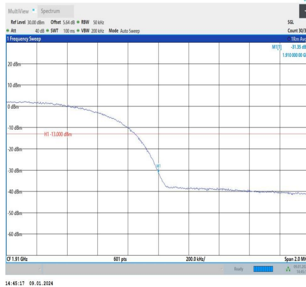
Band2-9538-2-PASS
