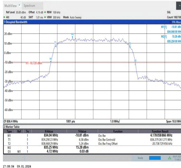
Band5-4182-4-PASS
