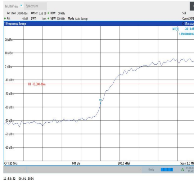
Band2-9262-1-PASS
