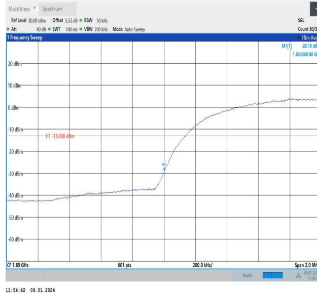
Band2-9262-3-PASS
