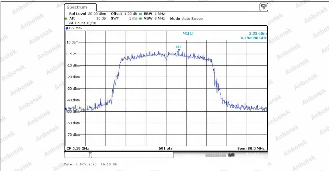
11N40SISO_Ant2_5190
