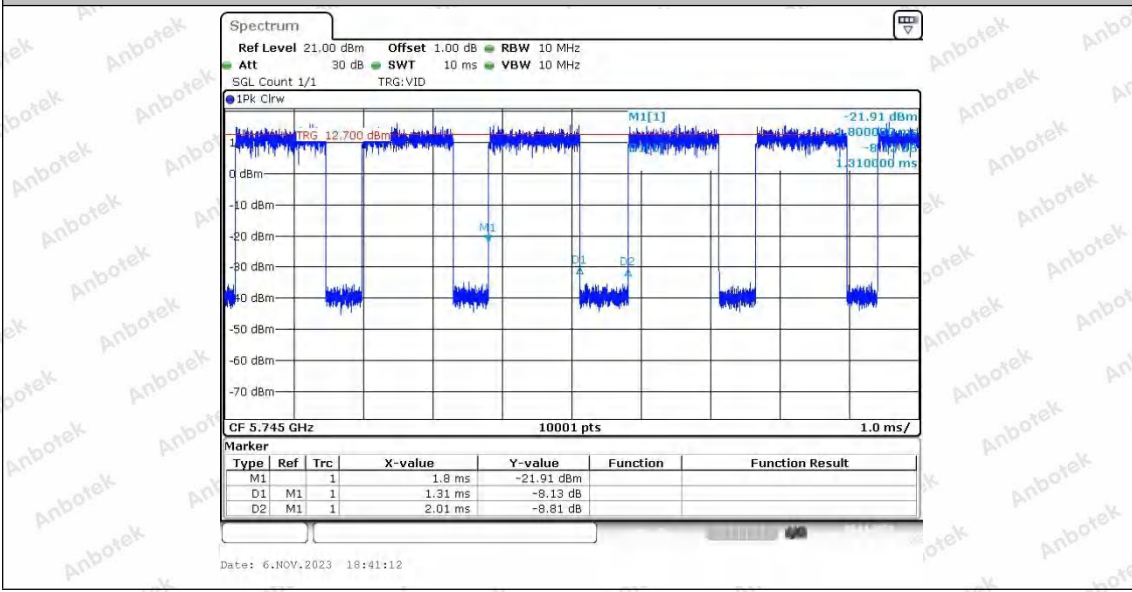
11AC20SISO_Ant2_5745
