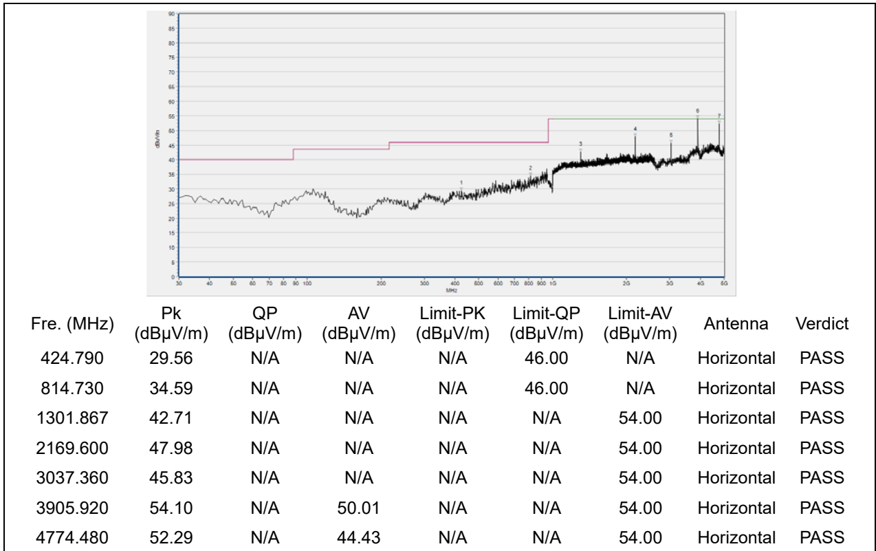
(433.92MHz, Antenna Horizontal, 30MHz to 5GHz)
