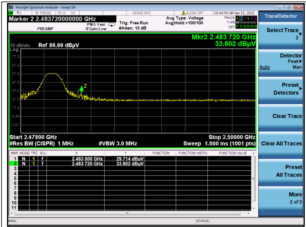
(PEAK, Channel 81)
