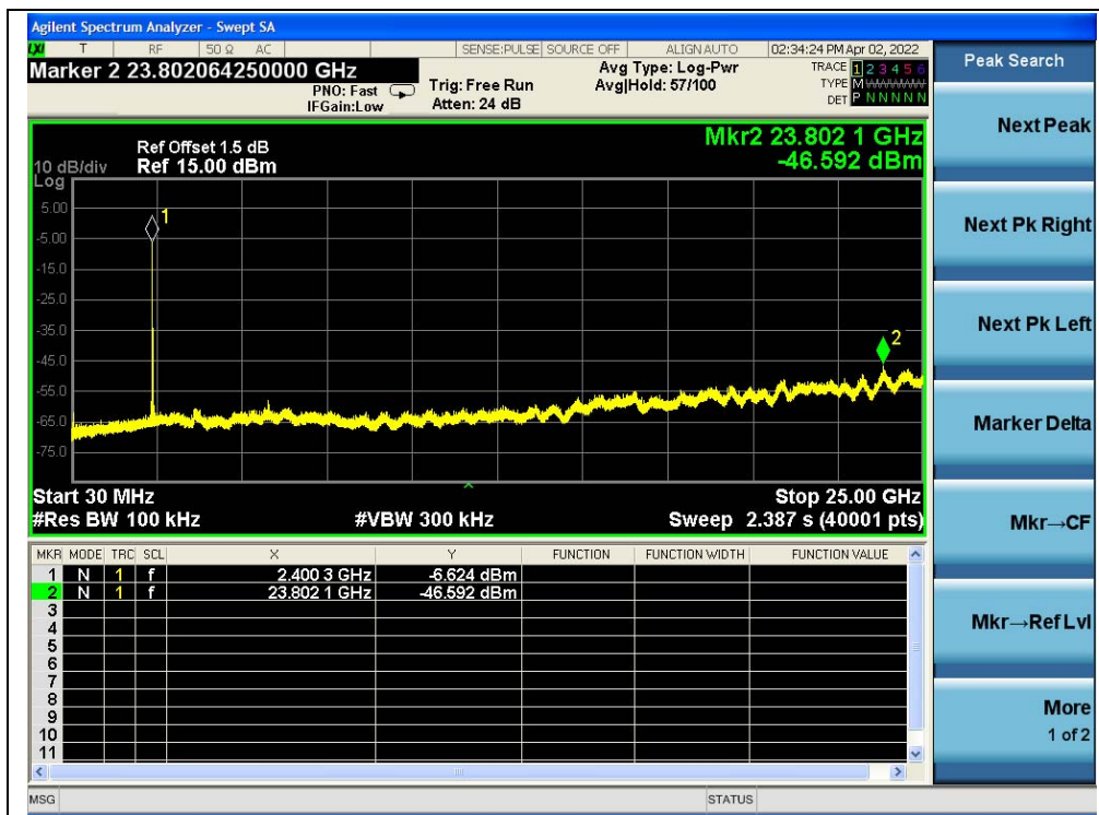
(30MHz to 25GHz, Channel 1)
