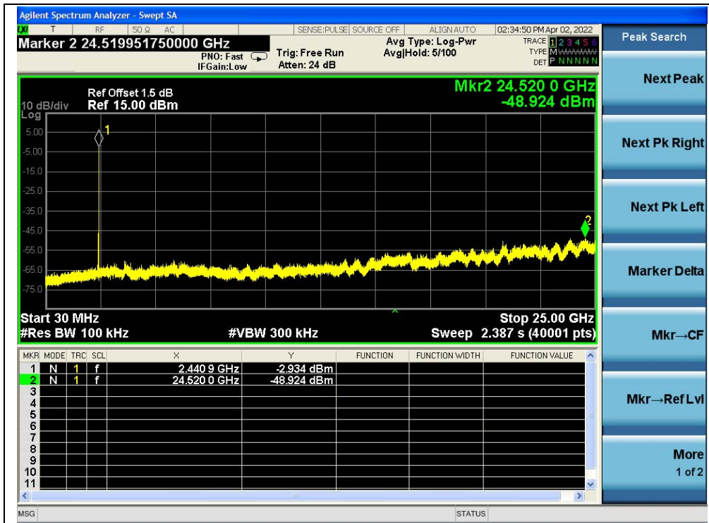
(30MHz to 25GHz, Channel 41)
