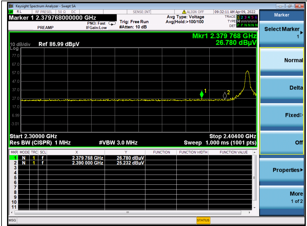
(PEAK, Channel 1)
