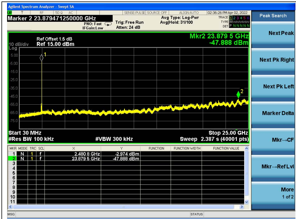
(30MHz to 25GHz, Channel 81)
