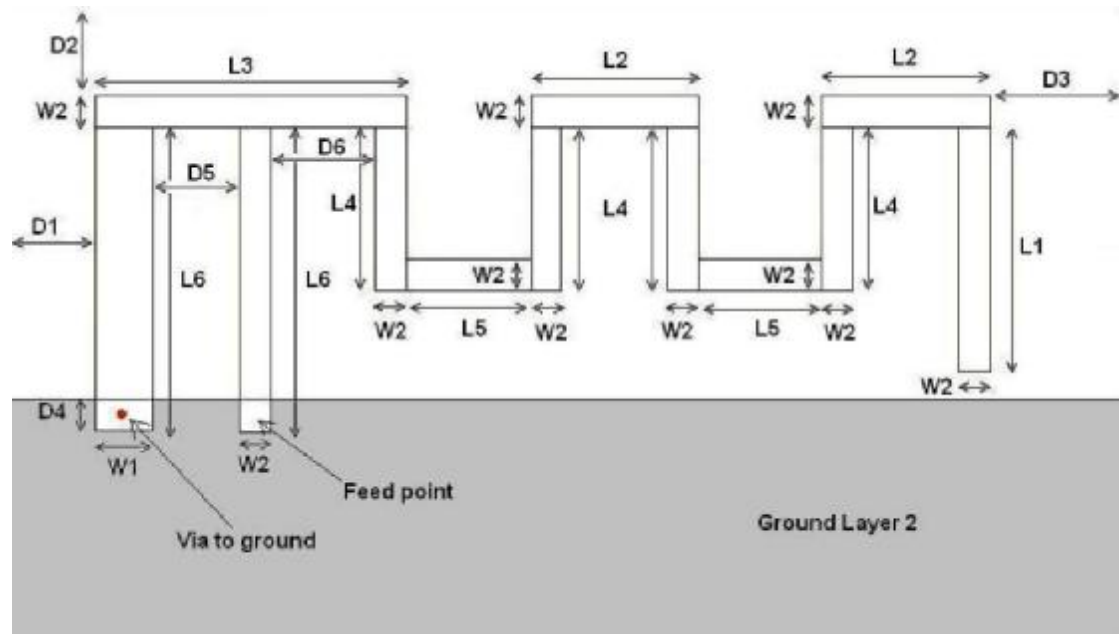
Figure 1: Antenna Dimensions
