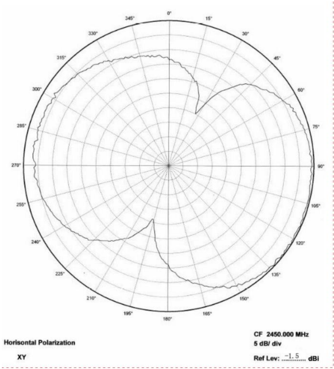
Figure 3: The radiation pattern for the antenna
