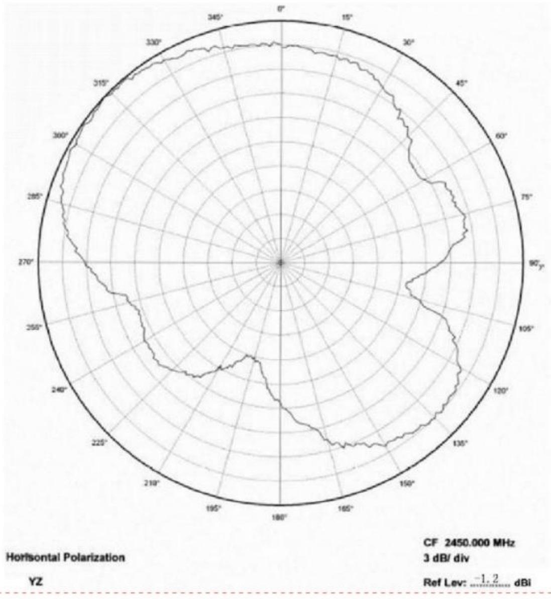
Figure 5: The radiation pattern for the antenna
