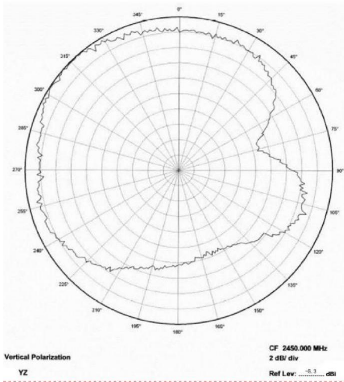
Figure 4: The radiation pattern for the antenna
