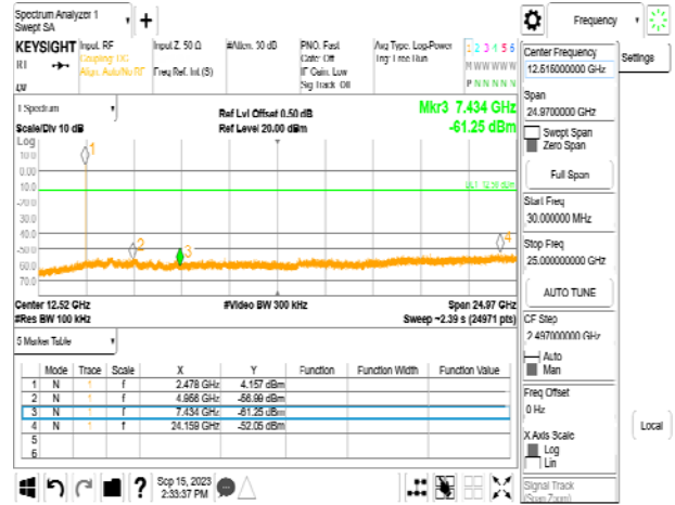
Spurious Emission_BLE 2M_HighCH38-2478MHz
