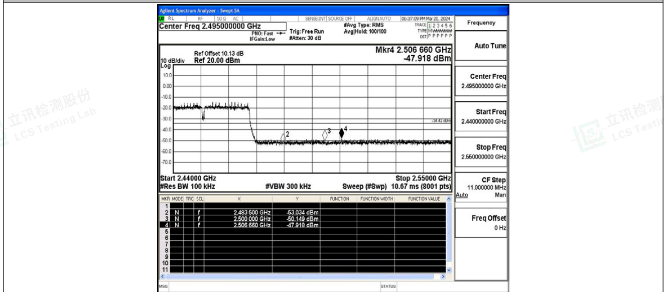
11N40SISO_Ant1_High_2452
