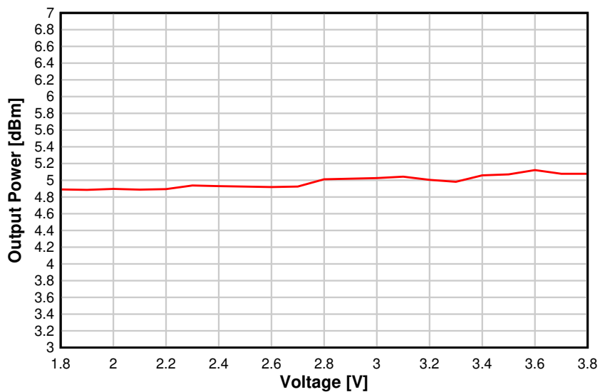
Figure 8-21. Output Power vs. Supply Voltage (VDDS) (BLE 1 Mbps, 2.44 GHz, +5 dBm)
