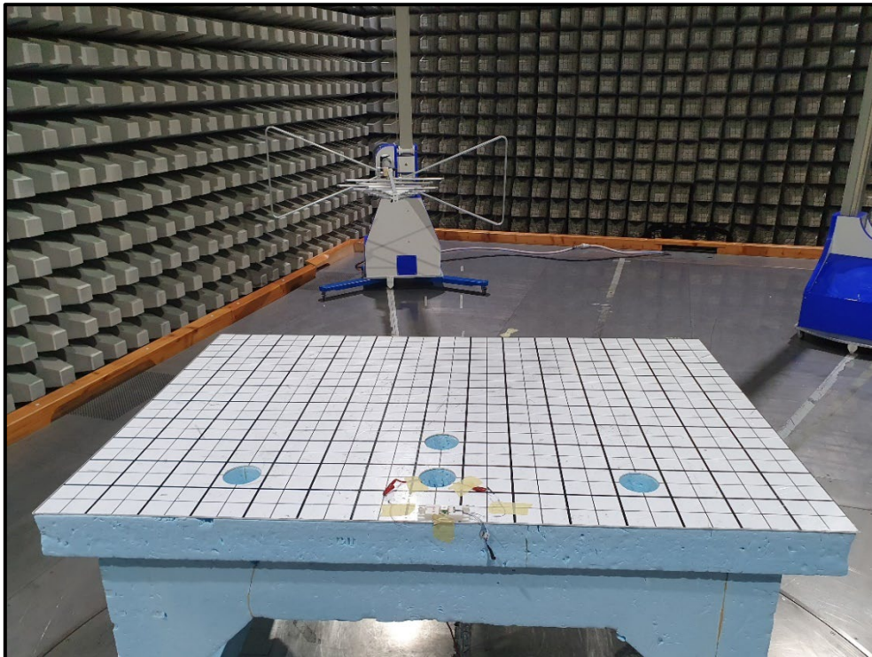
Photo 5: Radiated Test Setup - 30 MHz to 1GHz - EUT+ Internal Antenna
