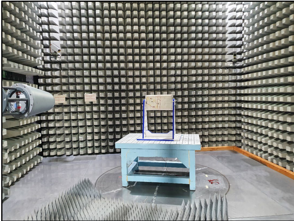
Photo 11: Radiated Test Setup - 1 GHz to 18 GHz - EUT+ External Antenna
