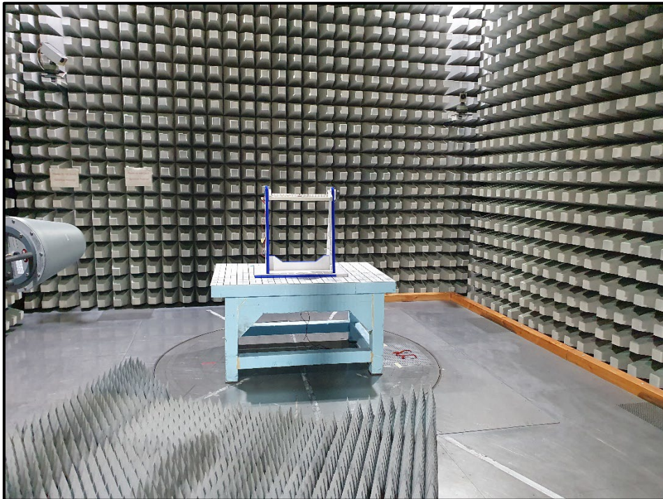
Photo 9: Radiated Test Setup - 1 GHz to 18 GHz - EUT+ Internal Antenna
