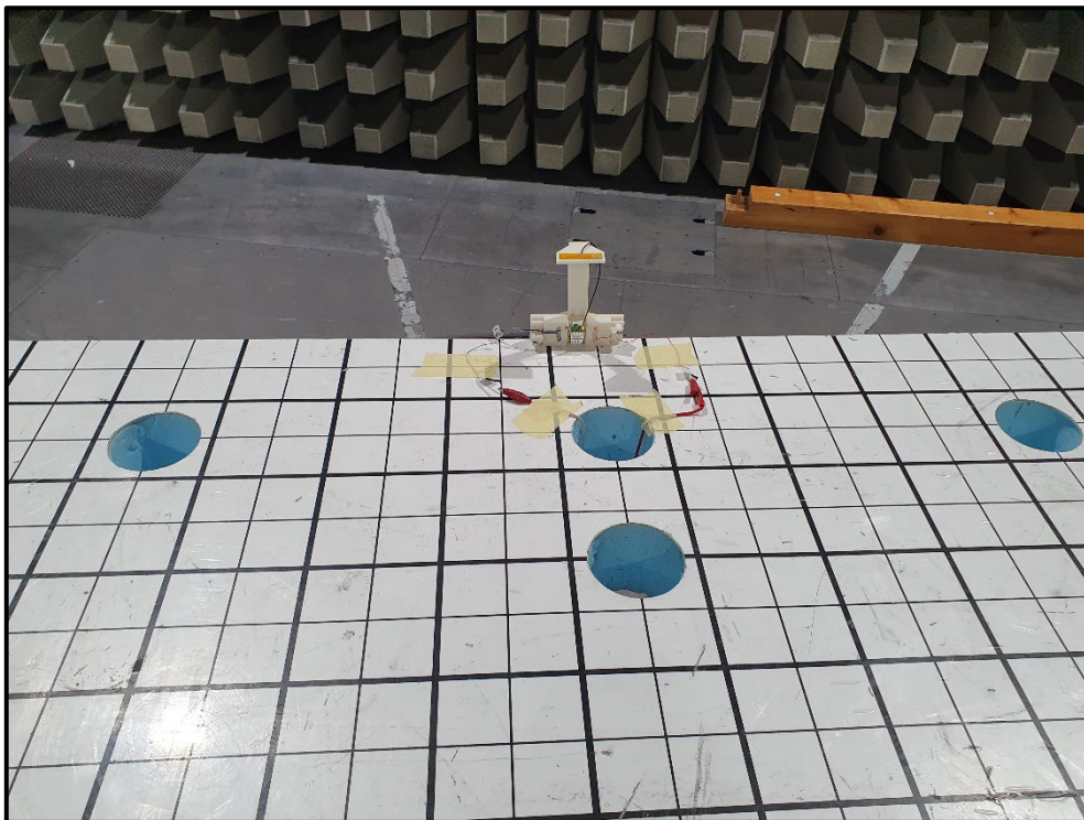
Photo 8: Radiated Test Setup - 30 MHz to 1GHz - EUT+ External Antenna
