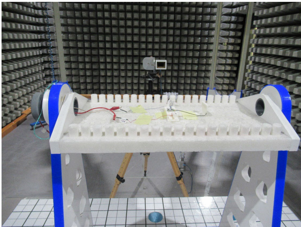
Photo 14: Radiated Test Setup - 18 GHz – 26.5 GHz - EUT+ Internal Antenna
