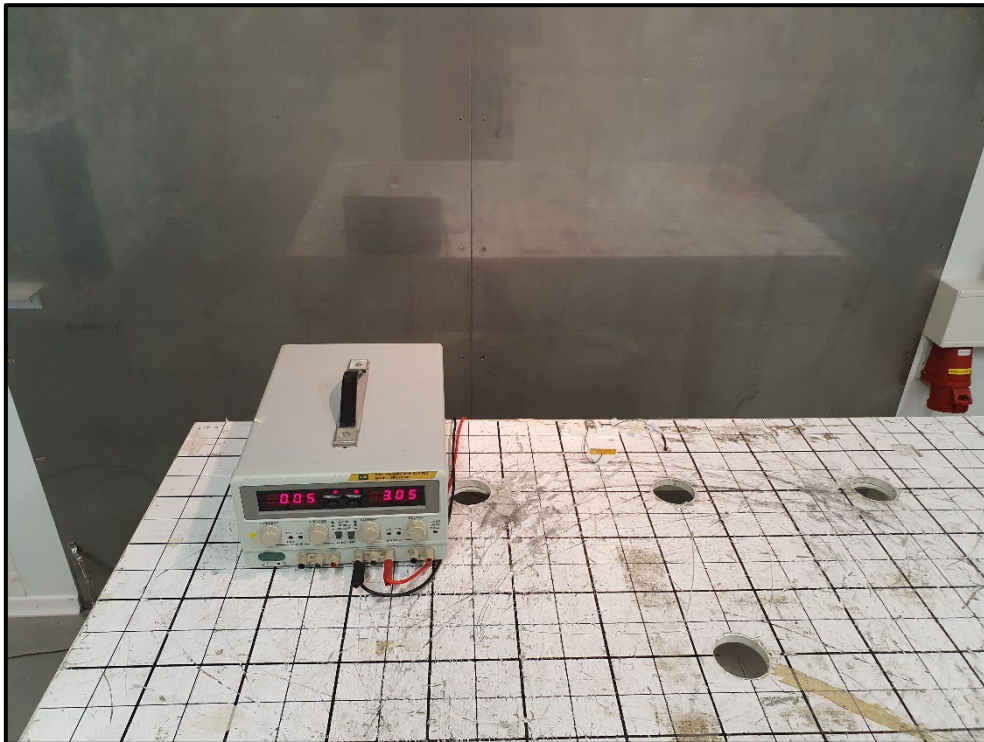
Photo 21 AC Conducted Test Setup- EUT+ External Antenna
