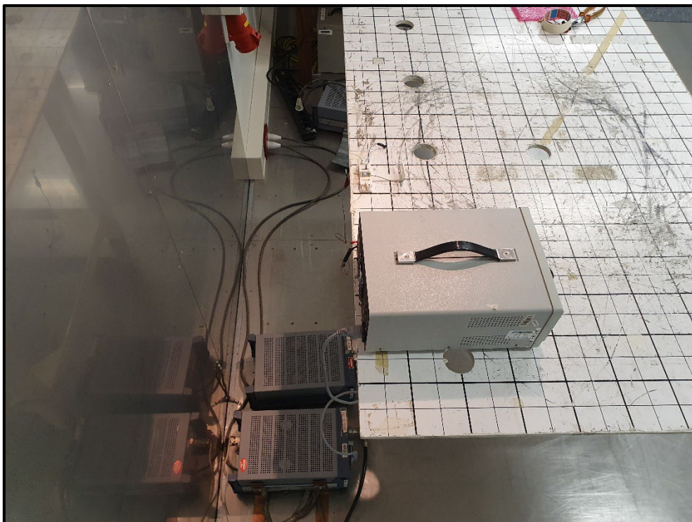
Photo 22 AC Conducted Test Setup- EUT+ External Antenna
