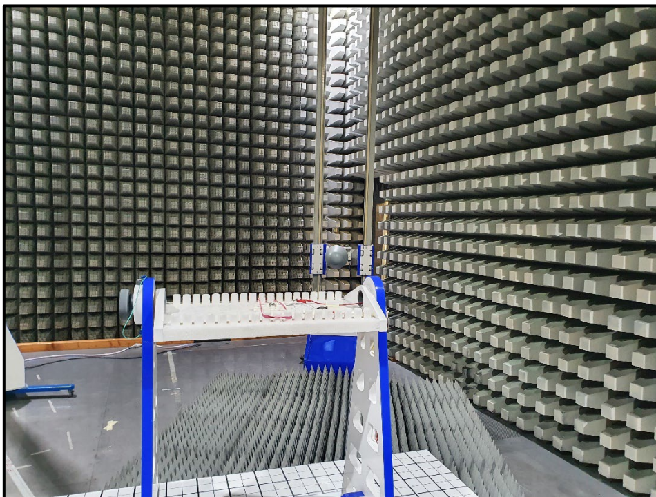
Photo 10: Radiated Test Setup - 1 GHz to 18 GHz - EUT+ Internal Antenna
