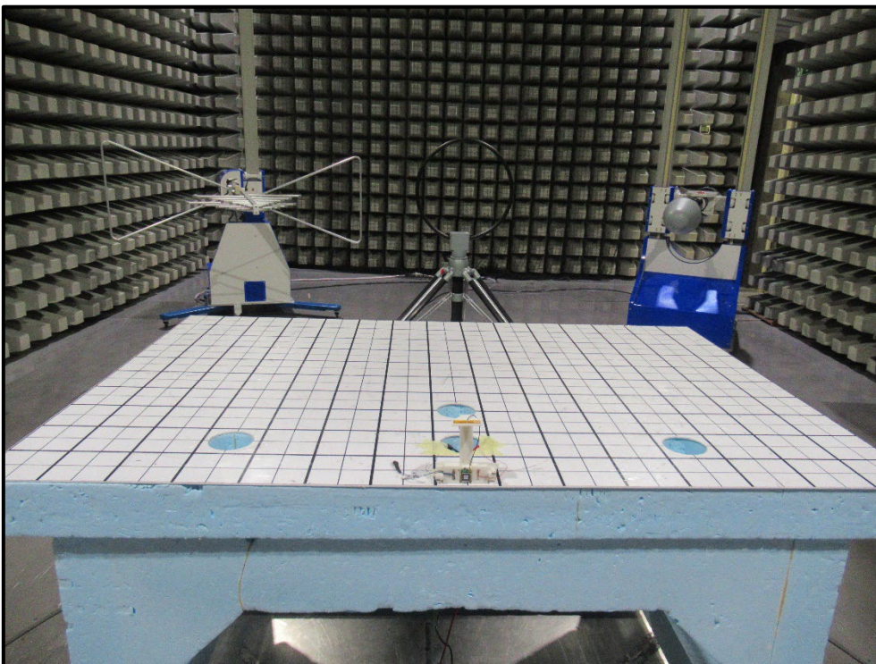
Photo 4: Radiated Test Setup - 9 kHz to 30 MHz - EUT+ External Antenna
