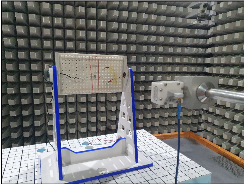
Photo 15: Radiated Test Setup - 18 GHz – 26.5 GHz - EUT+ External Antenna
