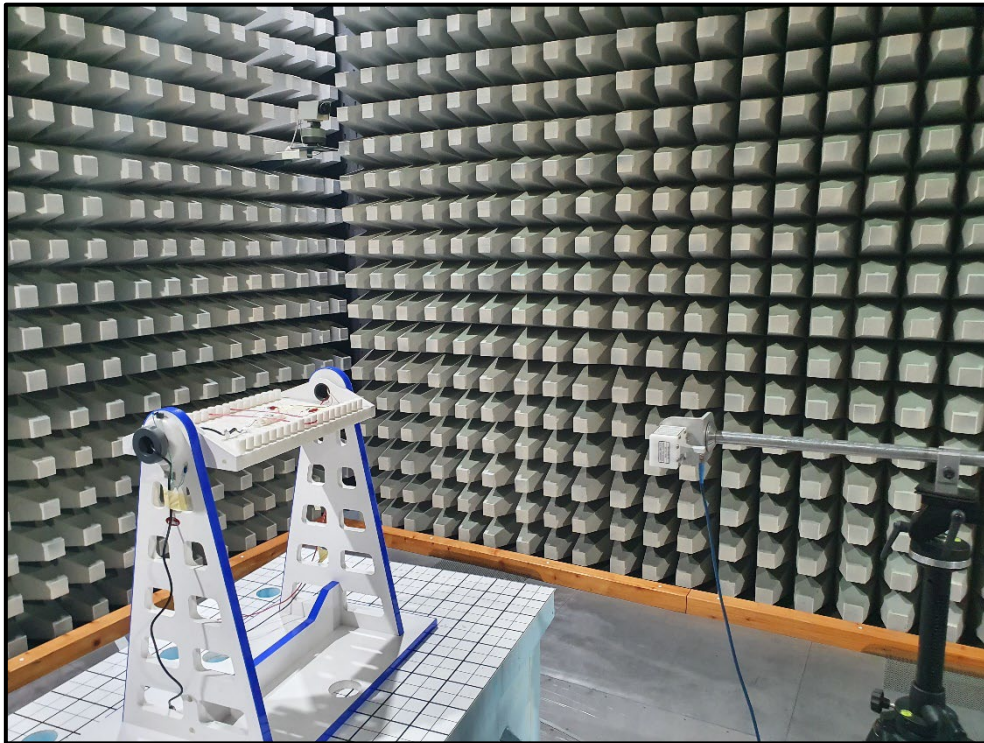
Photo 13: Radiated Test Setup - 18 GHz – 26.5 GHz - EUT+ Internal Antenna
