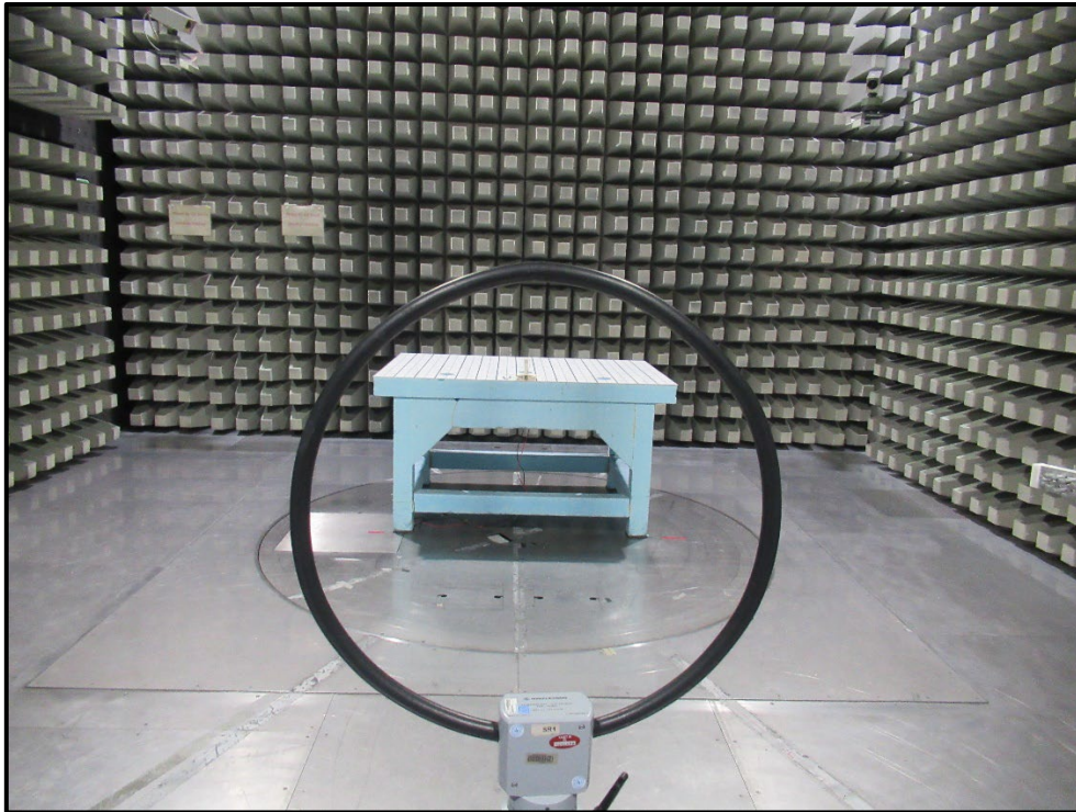
Picture 3: Radiated Test Setup - 9 kHz to 30 MHz – EUT+ External Antenna
