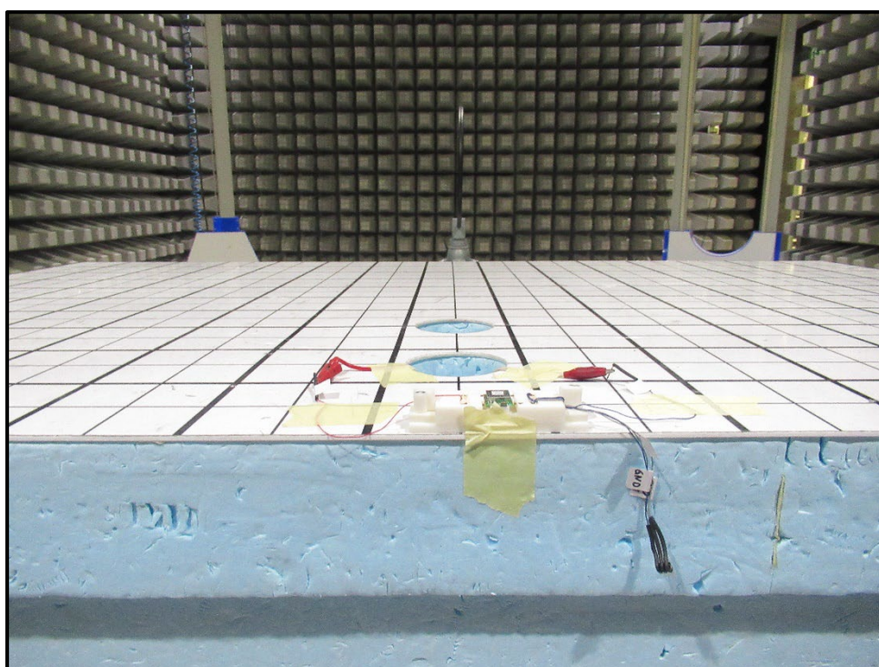
Photo 2: Radiated Test Setup - 9 kHz to 30 MHz - EUT+ Internal Antenna
