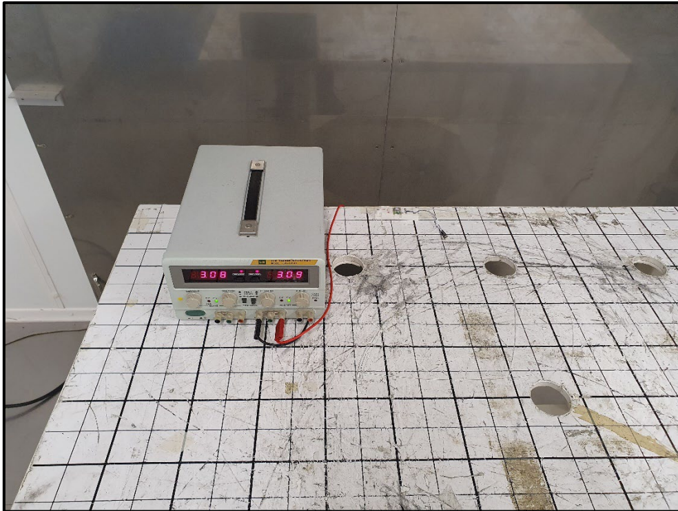
Photo 19 AC Conducted Test Setup- EUT+ Internal Antenna
