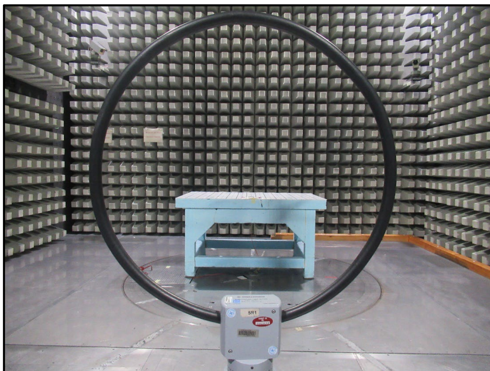
Picture 1: Radiated Test Setup - 9 kHz to 30 MHz – EUT+ Internal Antenna
