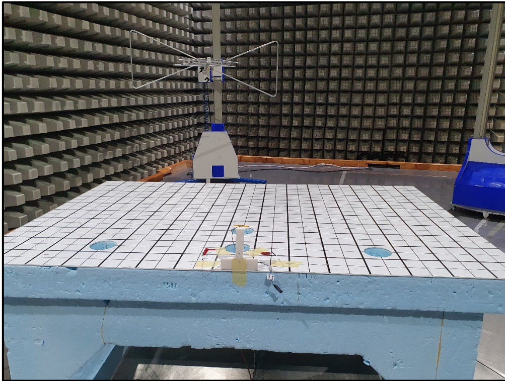
Photo 7: Radiated Test Setup - 30 MHz to 1GHz - EUT+ External Antenna
