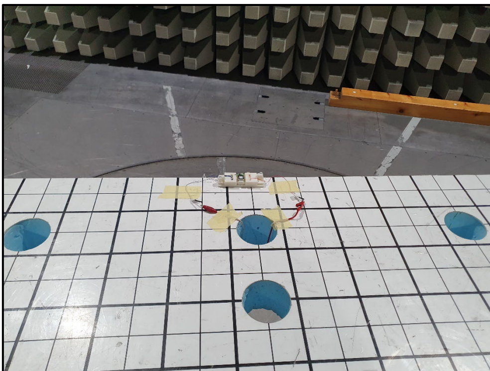
Photo 6: Radiated Test Setup - 30 MHz to 1GHz - EUT+ Internal Antenna
