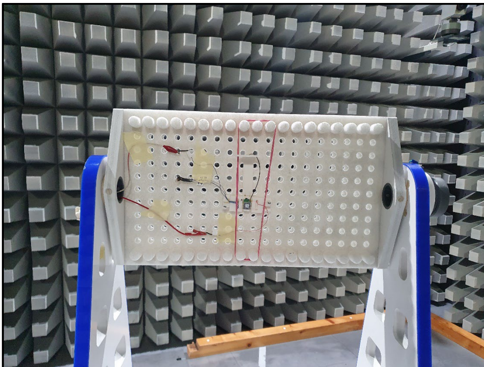
Photo 12: Radiated Test Setup - 1 GHz to 18 GHz - EUT+ External Antenna
