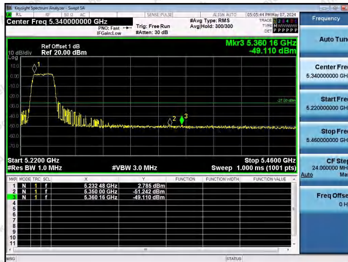
11N20MIMO-Ant2-5240-PASS
