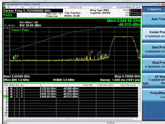
11A-Ant2-5745-PASS
