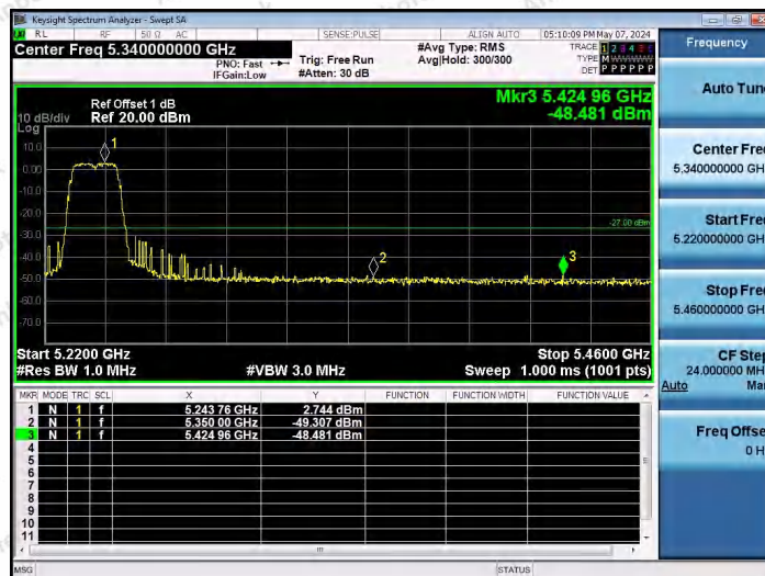
11AC20MIMO-Ant1-5240-PASS
