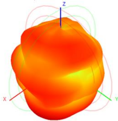
2410.0MHz H+V, Eff: 67.75%
