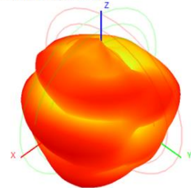
2500.0MHz H+V, Eff: 71.60%
