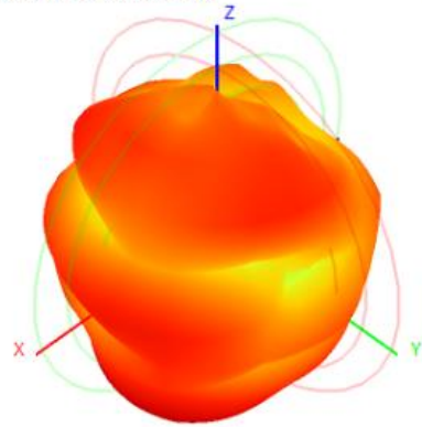
2450.0MHz H+V, Eff: 68.34%
