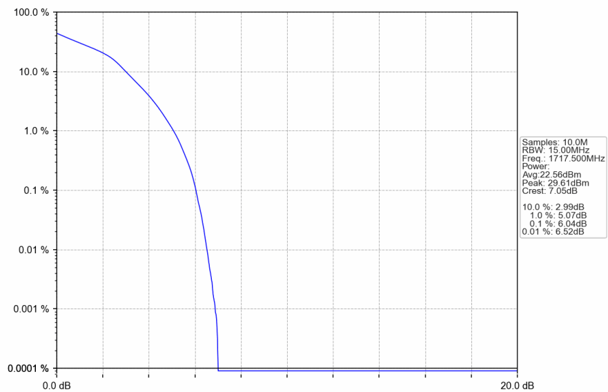
Band66_15MHz_16QAM_LCH_1717.5MHz_RB_75_0_NTNV
