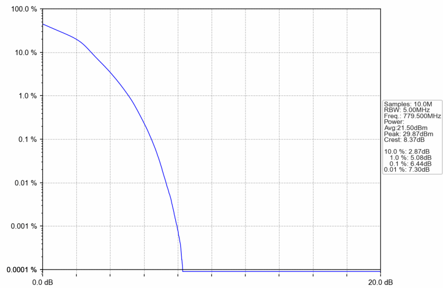
Band13_5MHz_16QAM_LCH_779.5MHz_RB_25_0_NTNV
