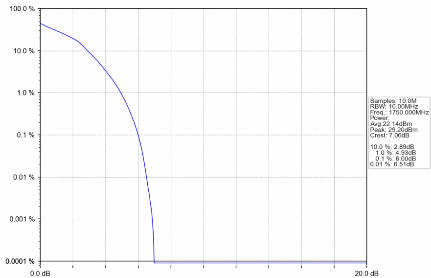
Band4_10MHz_16QAM_HCH_1750MHz_RB_50_0_NTNV
