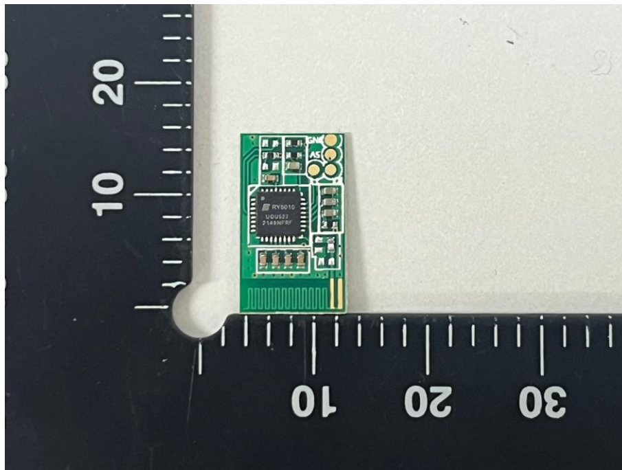
Main board - Front Top
