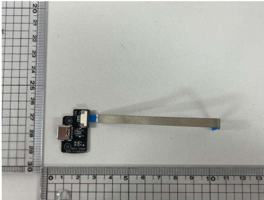
Sub board 2 - Front Top
