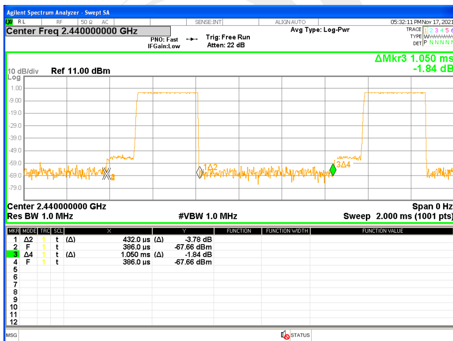
Duty cycle
