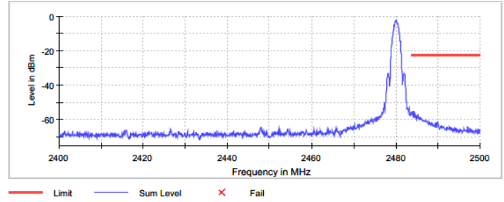
Figure 2.6.6-2: Upper Band-edge
