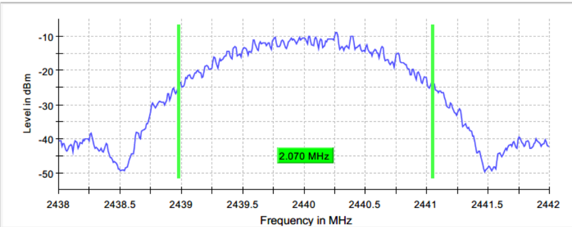
Figure 2.4.6-5: 99% BW - MCH
