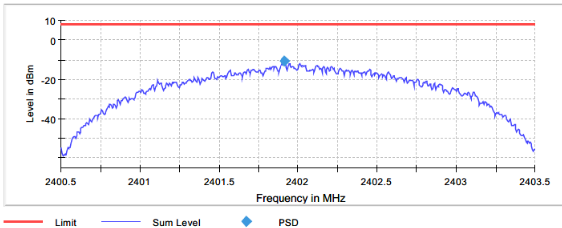
Figure 2.5.6-1: PSD – LCH
