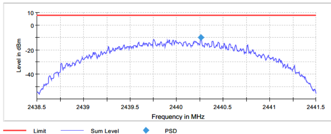
Figure 2.5.6-2: PSD – MCH
