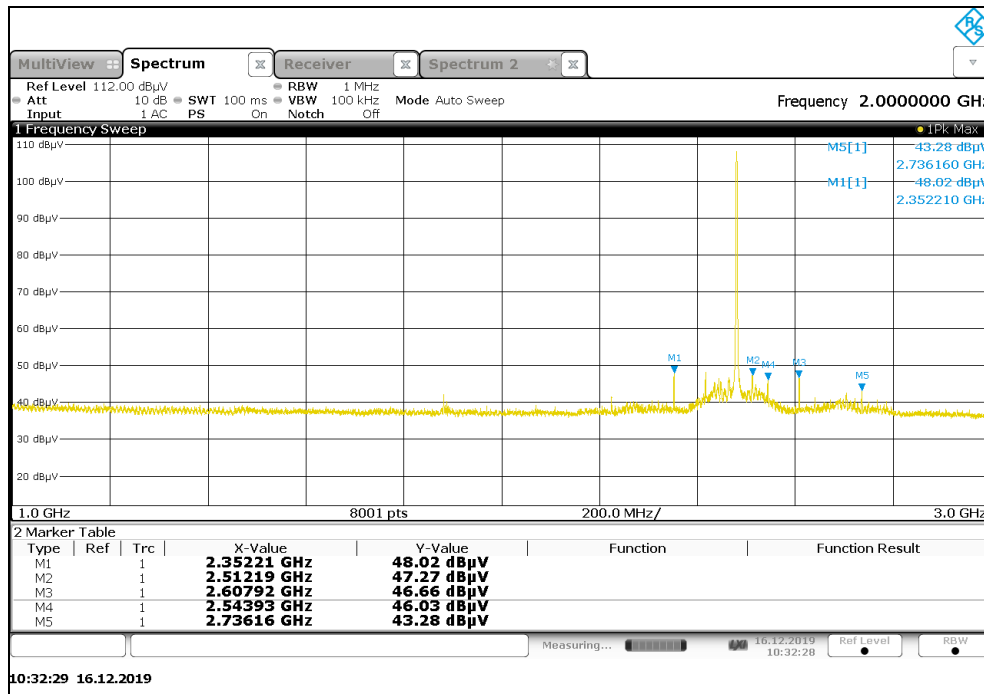
Figure A-4: Radiated Emissions – 1GHz-3GHz
