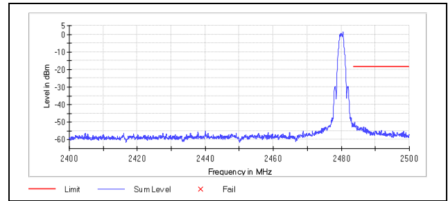
Figure 7.5.1.2-5: Upper Band-edge – 2 MBPS
