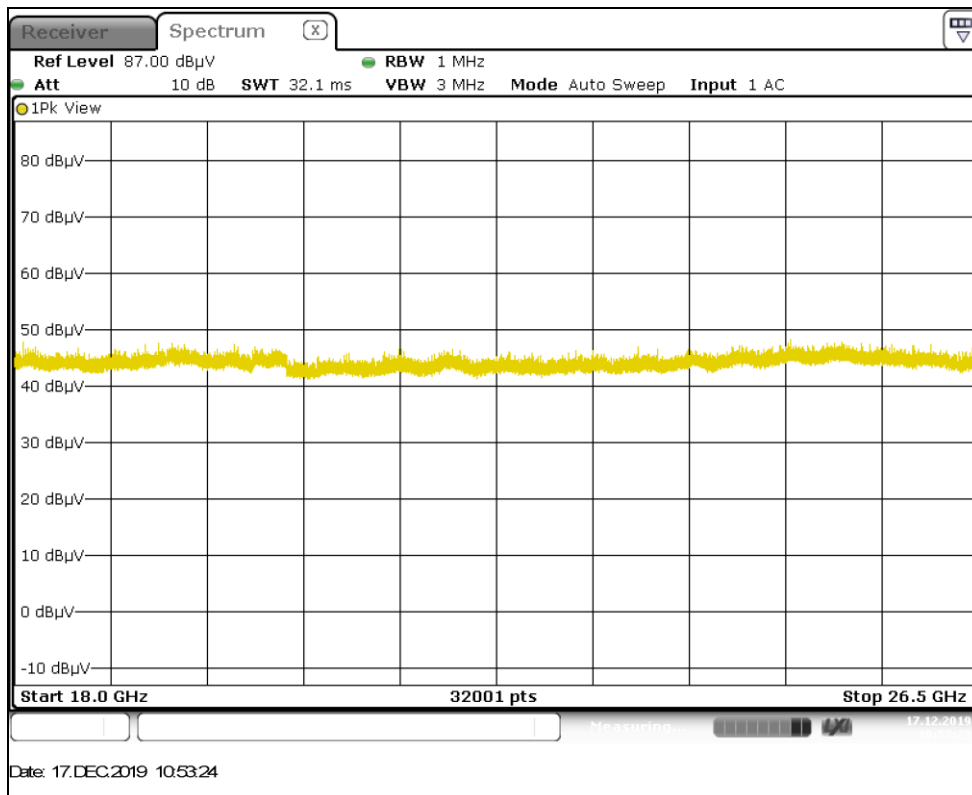
Figure A-6: Radiated Emissions – 18GHz-26.5GHz
