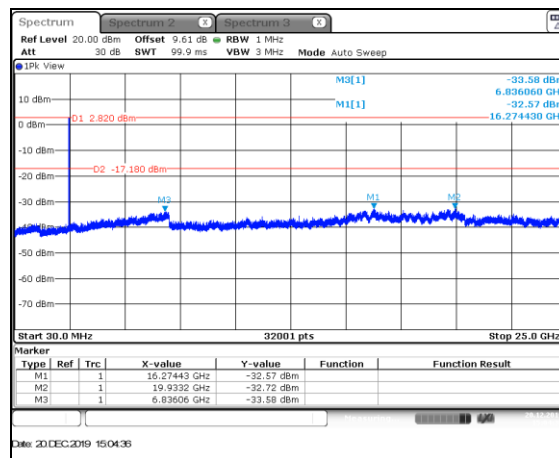
Figure 7.5.1.2-3: HCH – 30MHz–25GHz – 2 MBPS
