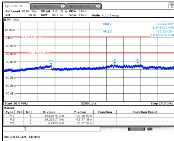
Figure 7.5.1.2-1: LCH – 30MHz–25GHz – 2 MBPS
