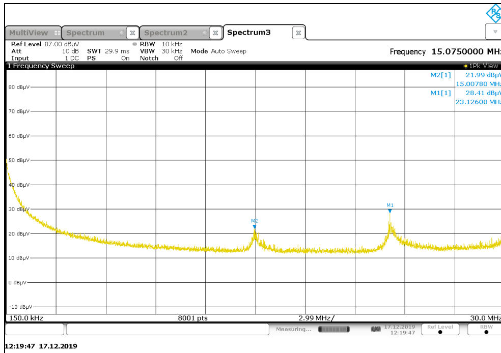
Figure A-2: Radiated Emissions – 150kHz-30MHz
