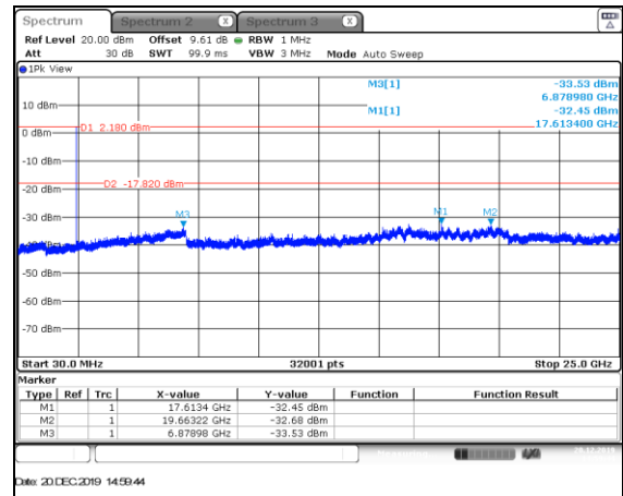
Figure 7.5.1.2-2: MCH – 30MHz–25GHz – 2 MBPS
