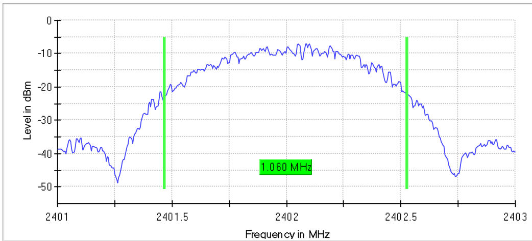
Figure 7.3.2-2: Sample Plot - 99% OBW - 1 MBPS
