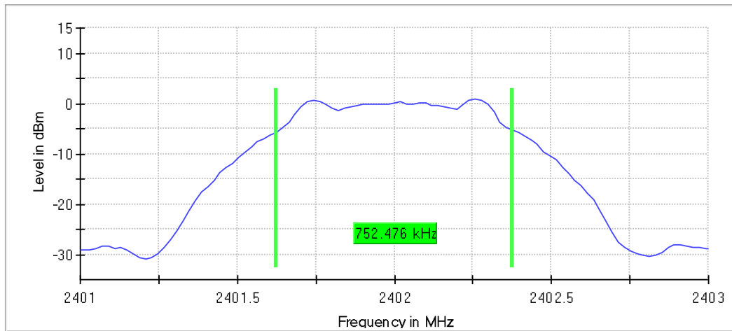
Figure 7.3.2-1: Sample Plot - 6dB BW – 1 MBPS
