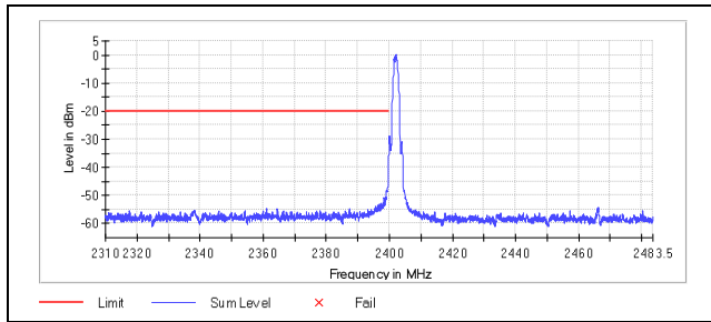
Figure 7.5.1.2-4: Lower Band-edge – 2 MBPS
