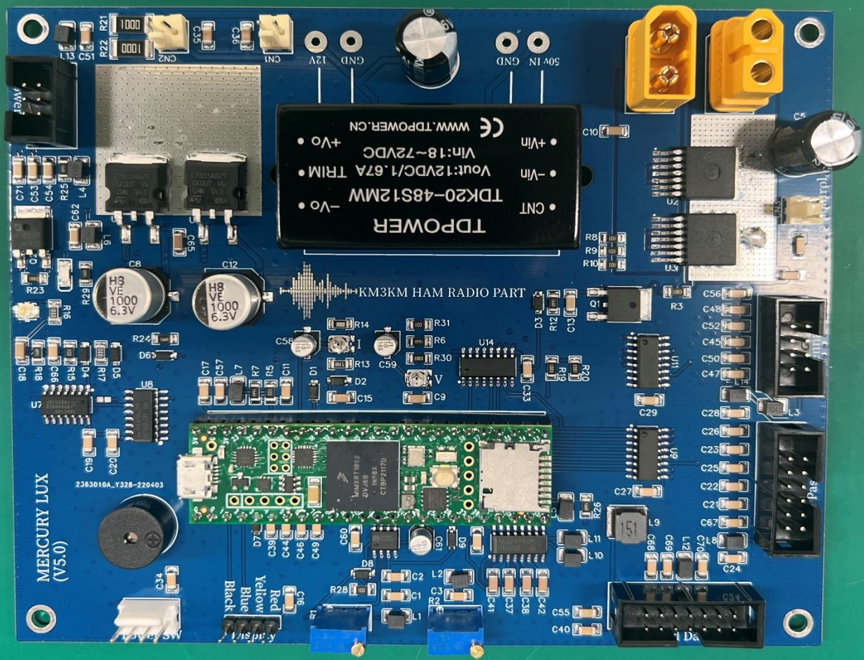
Controller Top View
