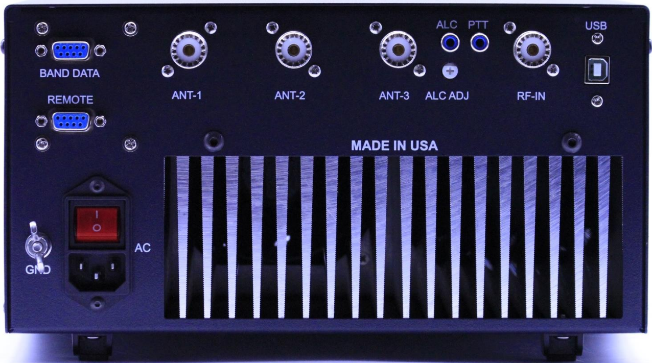
Rear View
